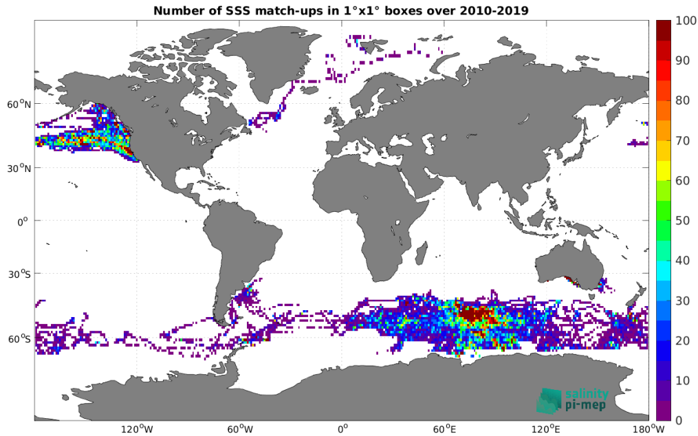
Figure 4: Number of SSS match-ups between Marine mammals SSS and the CCI SSS L4 Merged-OI v3.2 - 30-day running (ESA) SSS product for the Global Ocean Pi-MEP region over 1°x1° boxes and for the full satellite product period.
