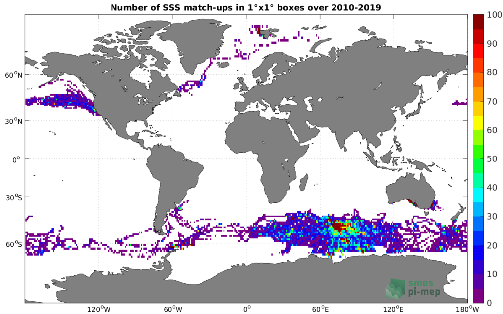
Figure 4: Number of SSS match-ups between Marine mammals SSS and the CCI SSS L4 Merged-OI v3.2 - 30-day running (ESA) SSS product for the Global Ocean Pi-MEP region over 1^\circ \times 1^\circ boxes and for the full satellite product period.
