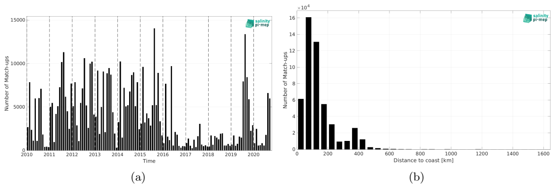
Figure 1: Number of match-ups between ICES and CCI SSS L4 Merged-OI v3.2 - 30-day running (ESA) SSS as a function of time (a) and as function of the distance to coast (b) over the Global Ocean Pi-MEP region and for the full satellite product period.
