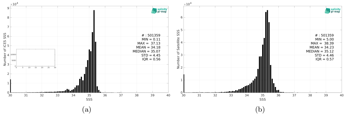
Figure 2: Histograms of SSS from ICES (a) and CCI SSS L4 Merged-OI v3.2 - 30-day running (ESA) (b) considering all match-up pairs per bins of 0.1 over the Global Ocean Pi-MEP region and for the full satellite product period.
