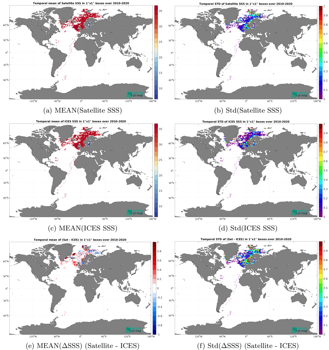
Figure 6: Temporal mean (left) and Std (right) of SSS from CCI SSS L4 Merged-OI v3.2 - 30-day running (ESA) (top), ICES (middle), and of \Delta SSS (Satellite - ICES). Only match-up pairs are used to generate these maps.
