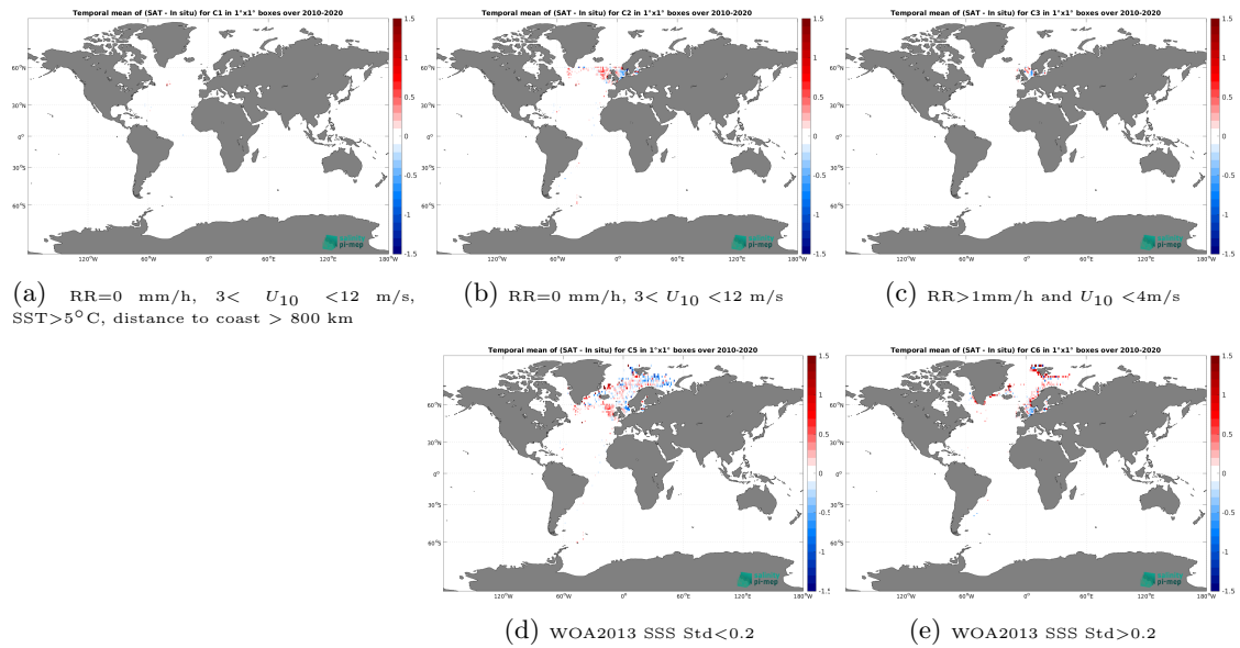
Figure 12: Temporal mean gridded over spatial boxes of size 1^\circ \times 1^\circ of \Delta\text{SSS} (CCI SSS L4 Merged-OI v3.2 - 30-day running (ESA) - ICES) for 5 different subdatasets corresponding to:RR=0 mm/h, 3 < U_{10} < 12 m/s, SST >5^\circ\text{C} , distance to coast > 800 km (a), RR=0 mm/h, 3 < U_{10} < 12 m/s (b), RR >1 mm/h and U_{10} < 4 m/s (c), WOA2013 SSS Std <0.2 (d), WOA2013 SSS Std >0.2 (e).
