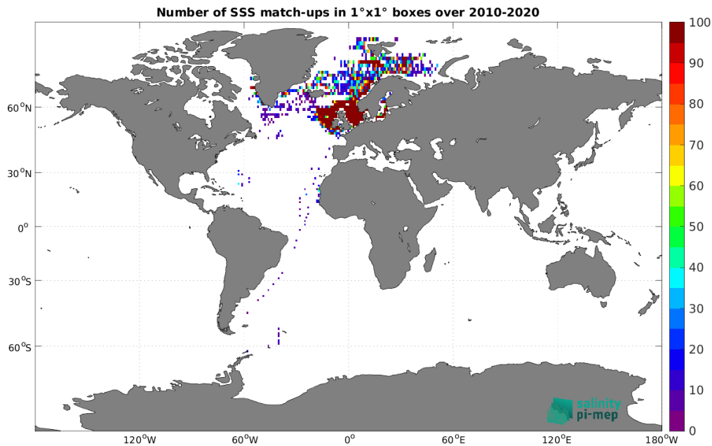
Figure 4: Number of SSS match-ups between ICES SSS and the CCI SSS L4 Merged-OI v3.2 - 30-day running (ESA) SSS product for the Global Ocean Pi-MEP region over 1^\circ \times 1^\circ boxes and for the full satellite product period.
