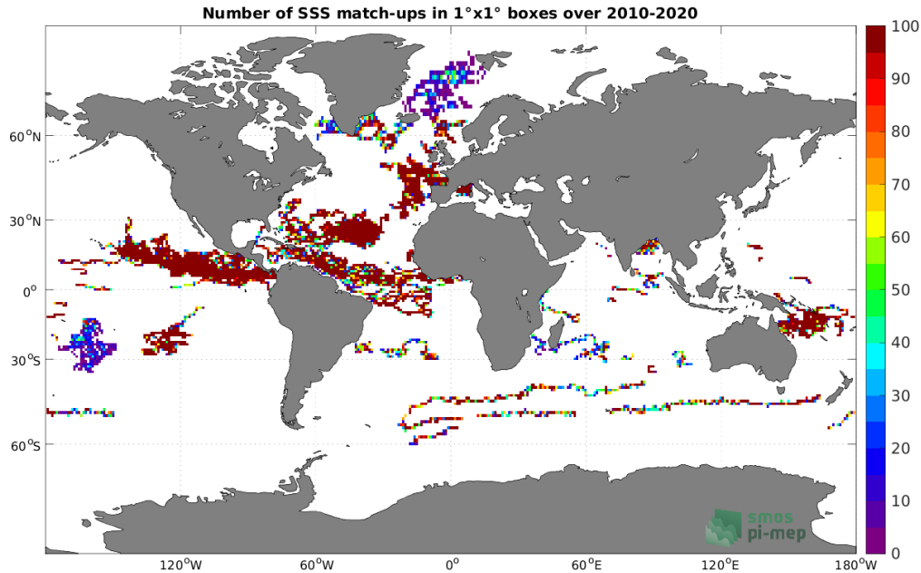
Figure 3: Number of SSS match-ups between Surface drifters SSS and the CCI SSS L4 Merged-OI v3.2 - 30-day running (ESA) SSS product for the Global Ocean Pi-MEP region over 1^\circ \times 1^\circ boxes and for the full satellite product period.
