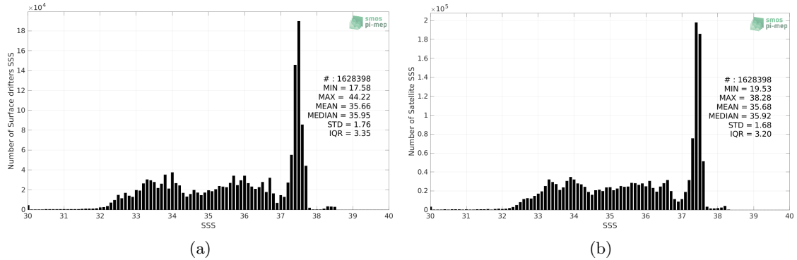
Figure 2: Histograms of SSS from Surface drifters (a) and CCI SSS L4 Merged-OI v3.2 - 30-day running (ESA) (b) considering all match-up pairs per bins of 0.1 over the Global Ocean Pi-MEP region and for the full satellite product period.
