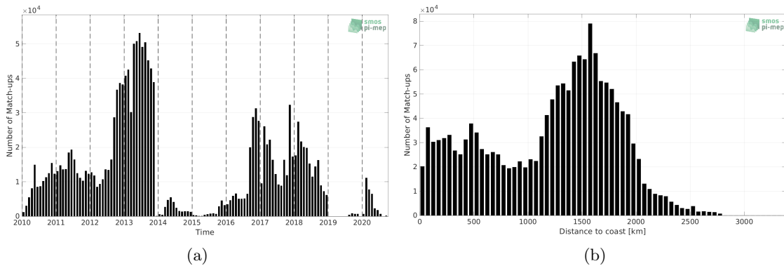
Figure 1: Number of match-ups between Surface drifters and CCI SSS L4 Merged-OI v3.2 - 30-day running (ESA) SSS as a function of time (a) and as function of the distance to coast (b) over the Global Ocean Pi-MEP region and for the full satellite product period.
