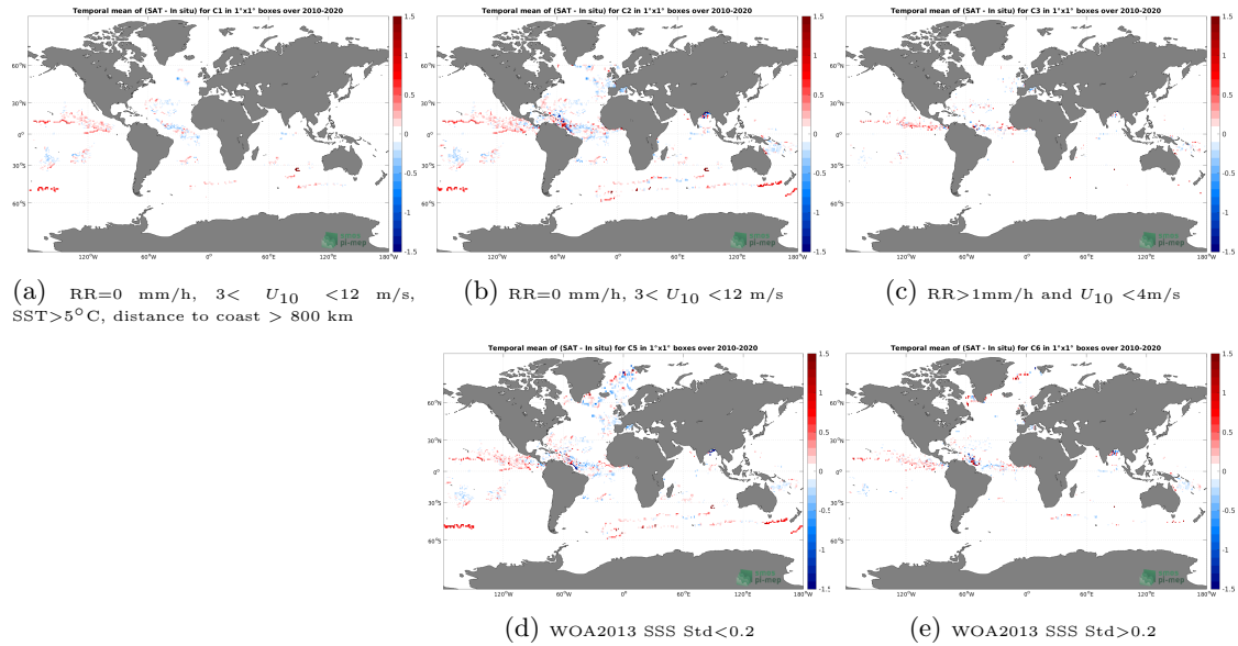
Figure 11: Temporal mean gridded over spatial boxes of size 1^\circ \times 1^\circ of \Delta\text{SSS} (CCI SSS L4 Merged-OI v3.2 - 30-day running (ESA) - Surface drifters) for 5 different subdatasets corresponding to:RR=0 mm/h, 3 < U_{10} < 12 m/s, SST >5^\circ\text{C} , distance to coast > 800 km (a), RR=0 mm/h, 3 < U_{10} < 12 m/s (b), RR >1 mm/h and U_{10} < 4 m/s (c), WOA2013 SSS Std <0.2 (d), WOA2013 SSS Std >0.2 (e).
