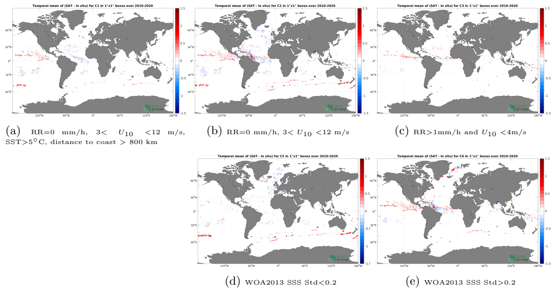
Figure 11: Temporal mean gridded over spatial boxes of size 1^\circ \times 1^\circ of \Delta SSS (CCI SSS L4 Merged-OI v3.2 - 30-day running (ESA) - Surface drifters) for 5 different subdatasets corresponding to:RR=0 mm/h, 3 < U_{10} < 12 m/s, SST > 5^\circ\text{C} , distance to coast > 800 km (a), RR=0 mm/h, 3 < U_{10} < 12 m/s (b), RR > 1 mm/h and U_{10} < 4 m/s (c), WOA2013 SSS Std < 0.2 (d), WOA2013 SSS Std > 0.2 (e).
