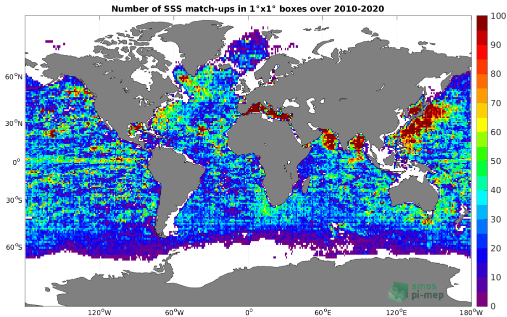
Figure 4: Number of SSS match-ups between Argo SSS and the CCI SSS L4 Merged-OI v3.2 - 30-day running (ESA) SSS product for the Global Ocean Pi-MEP region over 1°×1° boxes and for the full satellite product period.
