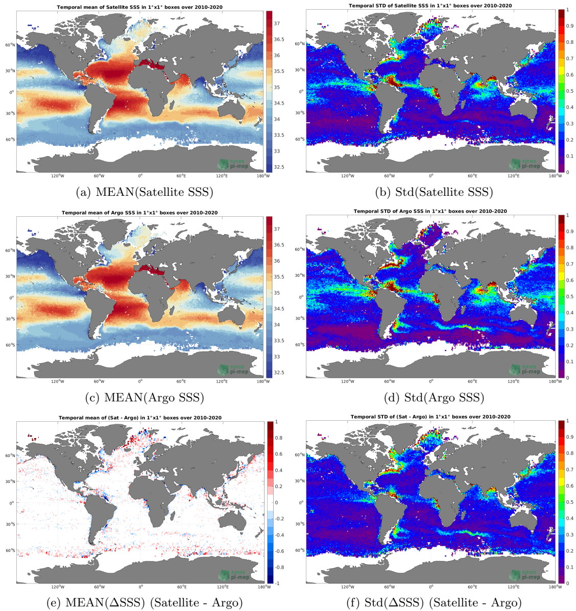
Figure 6: Temporal mean (left) and Std (right) of SSS from CCI SSS L4 Merged-OI v3.2 - 30-day running (ESA) (top), Argo (middle), and of \Delta SSS (Satellite - Argo). Only match-up pairs are used to generate these maps.
