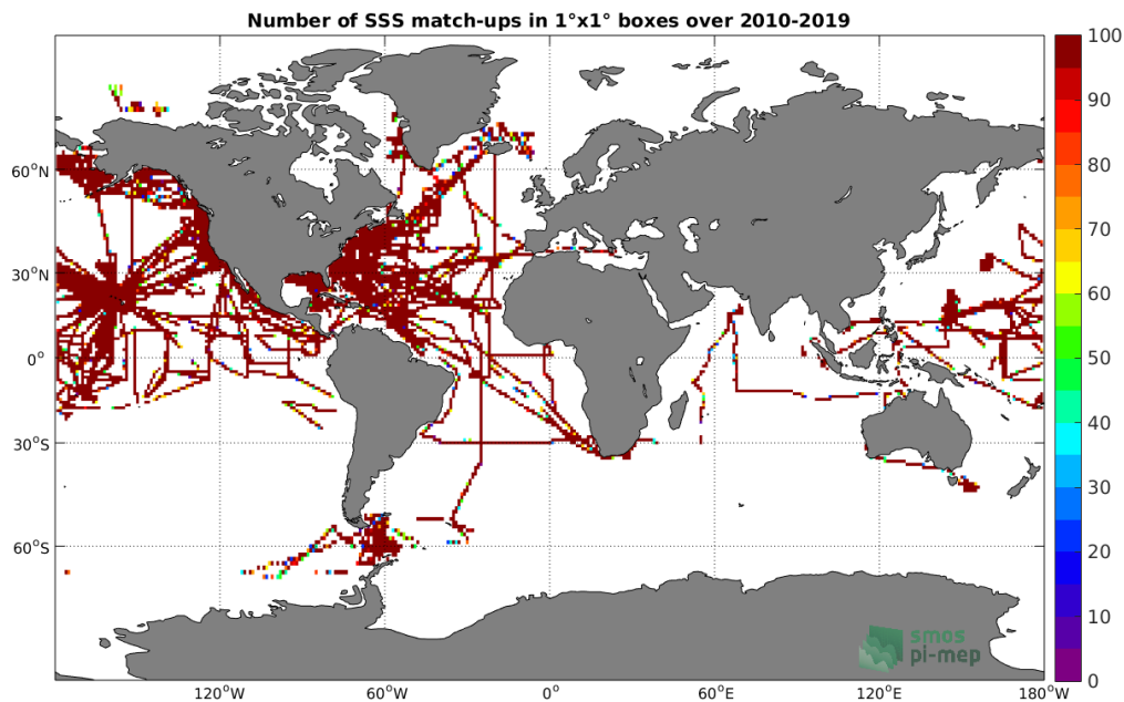
Figure 4: Number of SSS match-ups between TSG (SAMOS) SSS and the CCI L4 Merged-OI v2.31 - 7-day running (ESA) SSS product for the Global Ocean Pi-MEP region over 1^\circ \times 1^\circ boxes and for the full satellite product period.
