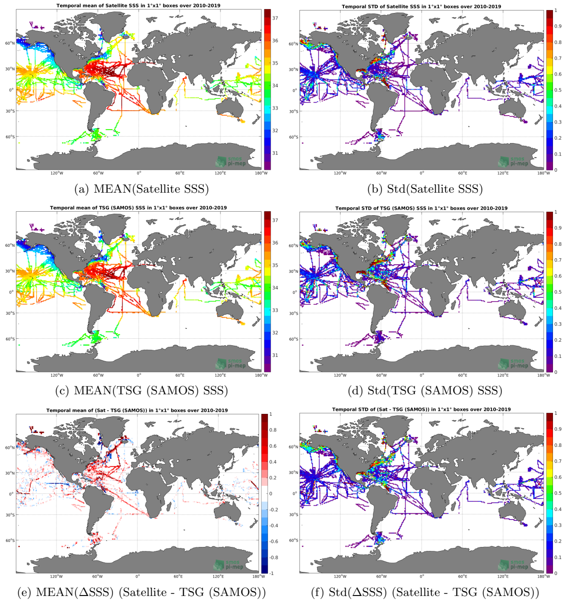
Figure 6: Temporal mean (left) and Std (right) of SSS from CCI L4 Merged-OI v2.31 - 7-day running (ESA) (top), TSG (SAMOS) (middle), and of \Delta SSS (Satellite - TSG (SAMOS)). Only match-up pairs are used to generate these maps.
