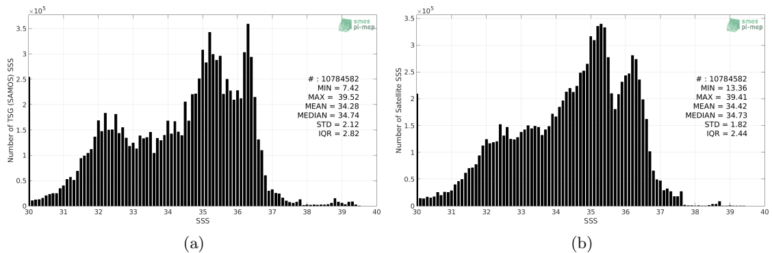
Figure 2: Histograms of SSS from TSG (SAMOS) (a) and CCI L4 Merged-OI v2.31 - 7-day running (ESA) (b) considering all match-up pairs per bins of 0.1 over the Global Ocean Pi-MEP region and for the full satellite product period.
