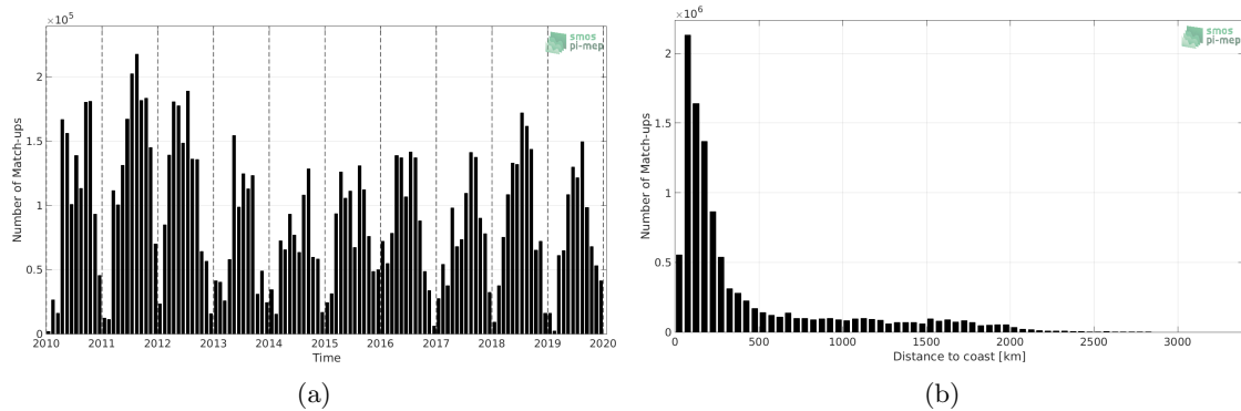
Figure 1: Number of match-ups between TSG (SAMOS) and CCI L4 Merged-OI v2.31 - 7-day running (ESA) SSS as a function of time (a) and as function of the distance to coast (b) over the Global Ocean Pi-MEP region and for the full satellite product period.
