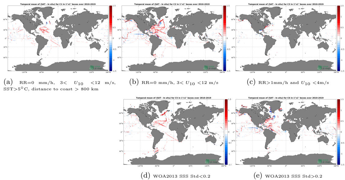
Figure 12: Temporal mean gridded over spatial boxes of size 1^\circ \times 1^\circ of \Delta SSS (CCI L4 Merged-OI v2.31 - 7-day running (ESA) - TSG (SAMOS)) for 5 different subdatasets corresponding to:RR=0 mm/h, 3 < U_{10} < 12 m/s, SST >5^\circ\text{C} , distance to coast > 800 km (a), RR=0 mm/h, 3 < U_{10} < 12 m/s (b), RR >1 mm/h and U_{10} < 4 m/s (c), WOA2013 SSS Std <0.2 (d), WOA2013 SSS Std >0.2 (e).
