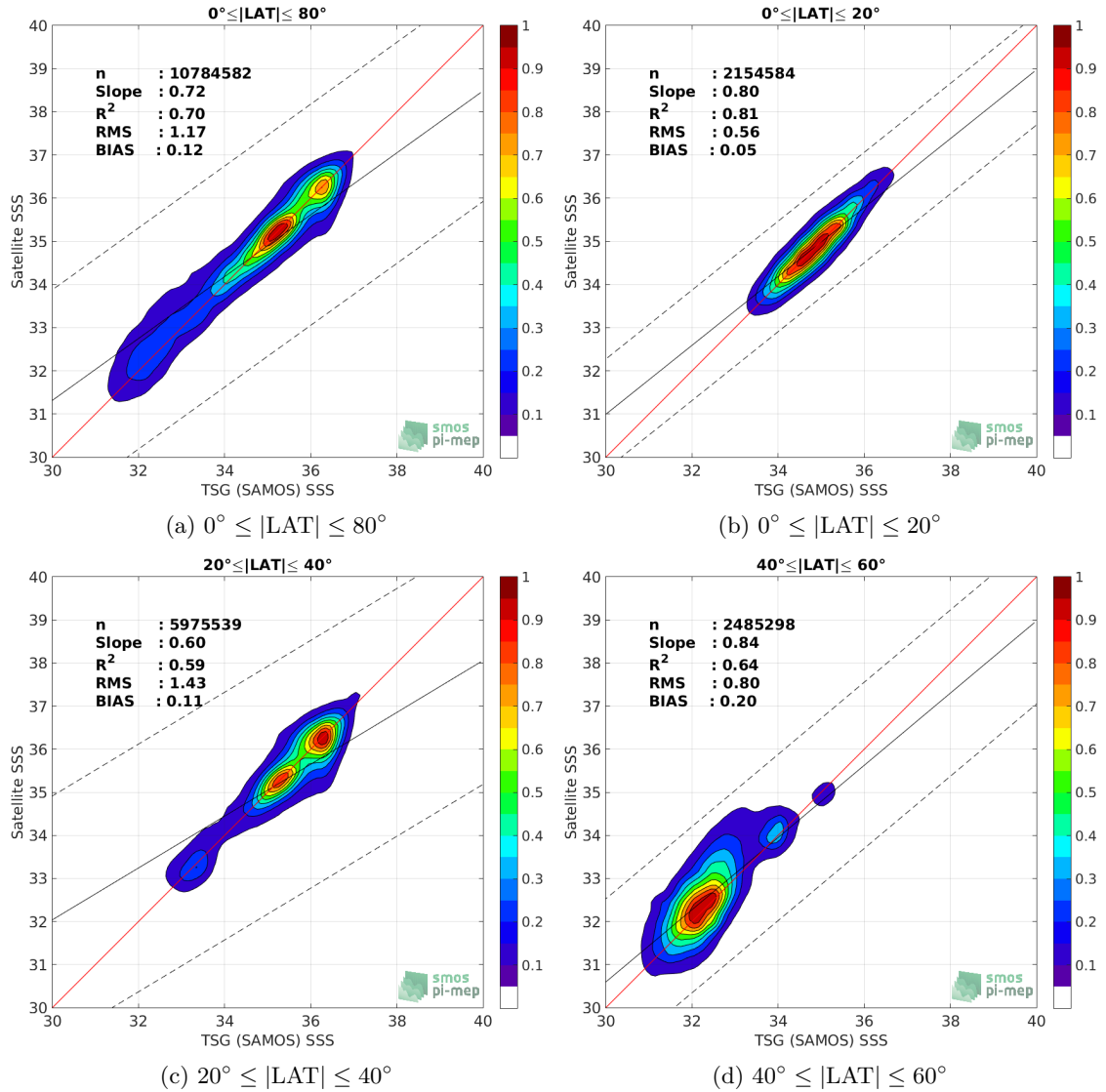
Figure 9: Contour maps of the concentration of CCI L4 Merged-OI v2.31 - 7-day running (ESA) SSS (y-axis) versus TSG (SAMOS) SSS (x-axis) at match-up pairs for different latitude bands. For each plot, the red line shows x=y . The black thin and dashed lines indicate a linear fit through the data cloud and the \pm 95\% confidence levels, respectively. The number match-up pairs n , the slope and R^2 coefficient of the linear fit, the root mean square (RMS) and the mean bias between satellite and in situ data are indicated for each latitude band in each plots.
