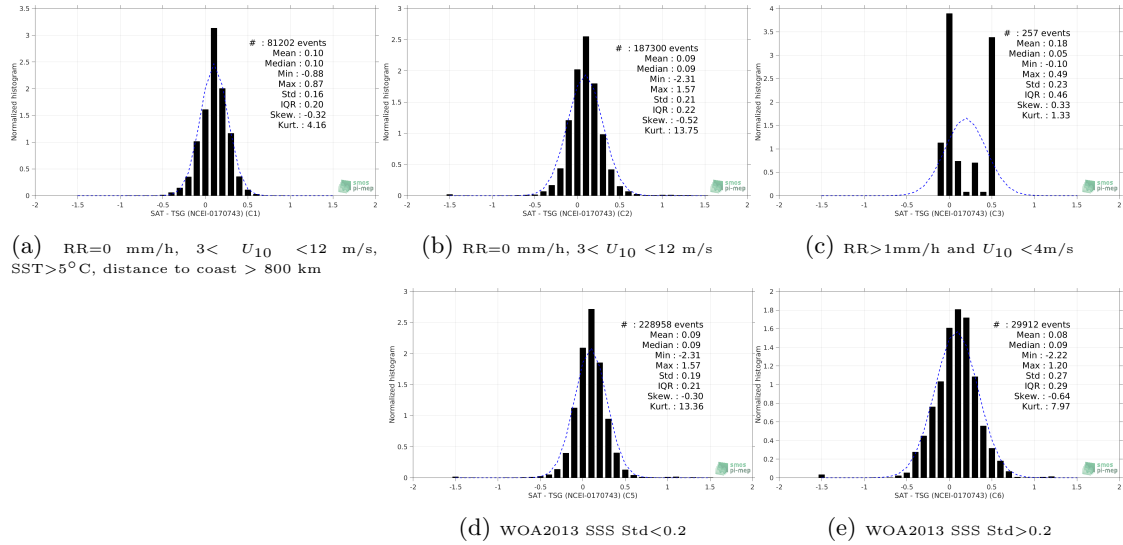
Figure 13: Normalized histogram of \Delta SSS (CCI SSS L4 Merged-OI v2.31 - 7-day running (ESA) - TSG (NCEI-0170743)) for 5 different subdatasets corresponding to: RR=0 mm/h, 3 < U_{10} < 12 m/s, SST>5°C, distance to coast > 800 km (a), RR=0 mm/h, 3 < U_{10} < 12 m/s (b), RR>1mm/h and U_{10} < 4 m/s (c), WOA2013 SSS Std<0.2 (d), WOA2013 SSS Std>0.2 (e).
