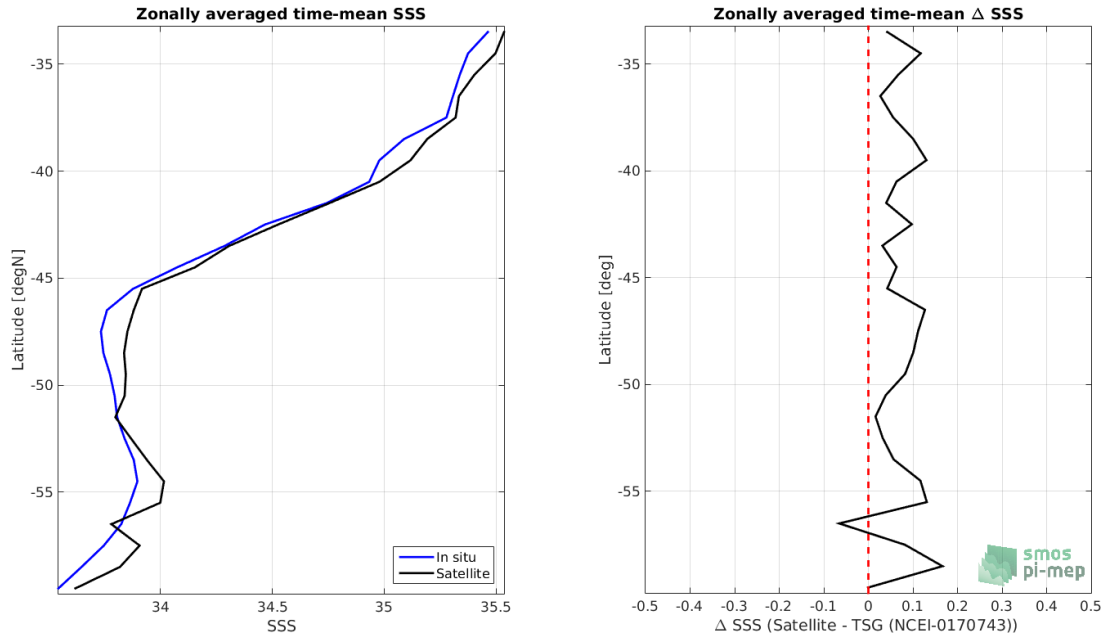
Figure 8: Left panel: Zonal mean SSS from CCI SSS L4 Merged-OI v2.31 - 7-day running (ESA) satellite product (black) and from TSG (NCEI-0170743) (blue). Right panel: Zonal mean of \Delta SSS (Satellite - TSG (NCEI-0170743)) for all the collected Pi-MEP match-up pairs estimated over the full satellite product period.
