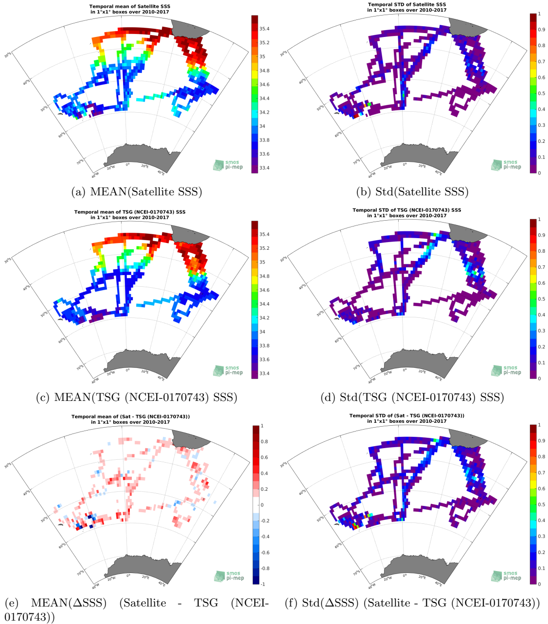
Figure 6: Temporal mean (left) and Std (right) of SSS from CCI SSS L4 Merged-OI v2.31 - 7-day running (ESA) (top), TSG (NCEI-0170743) (middle), and of \Delta SSS (Satellite - TSG (NCEI-0170743)). Only match-up pairs are used to generate these maps.
