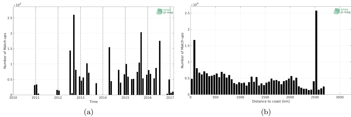
Figure 1: Number of match-ups between TSG (NCEI-0170743) and CCI SSS L4 Merged-OI v2.31 - 7-day running (ESA) SSS as a function of time (a) and as function of the distance to coast (b) over the Global Ocean Pi-MEP region and for the full satellite product period.
