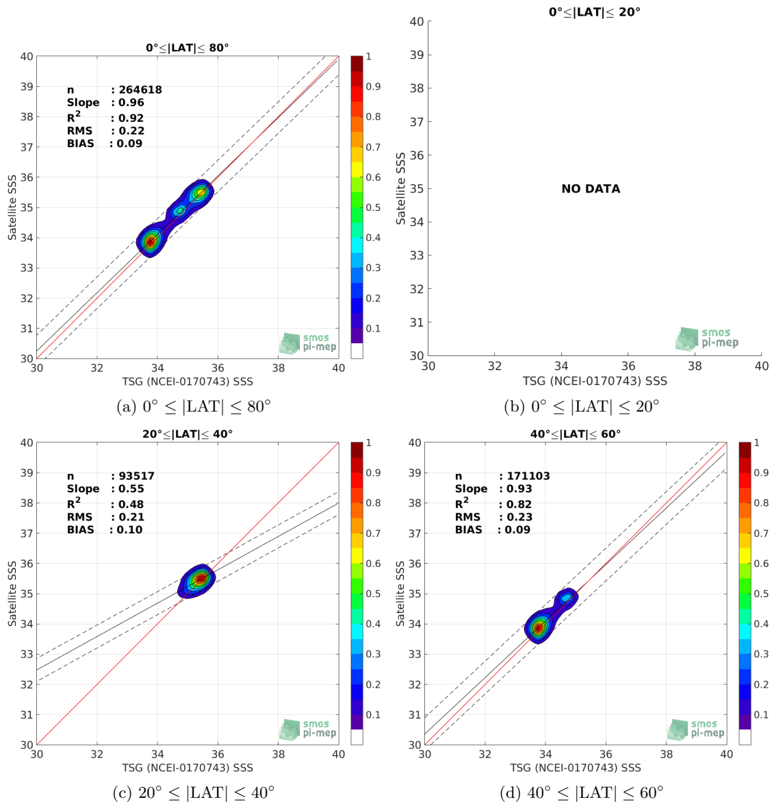
Figure 9: Contour maps of the concentration of CCI SSS L4 Merged-OI v2.31 - 7-day running (ESA) SSS ( y -axis) versus TSG (NCEI-0170743) SSS ( x -axis) at match-up pairs for different latitude bands. For each plot, the red line shows x=y . The black thin and dashed lines indicate a linear fit through the data cloud and the \pm 95\% confidence levels, respectively. The number match-up pairs n , the slope and R^2 coefficient of the linear fit, the root mean square (RMS) and the mean bias between satellite and in situ data are indicated for each latitude band in each plots.
