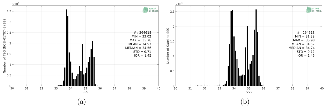
Figure 2: Histograms of SSS from TSG (NCEI-0170743) (a) and CCI SSS L4 Merged-OI v2.31 - 7-day running (ESA) (b) considering all match-up pairs per bins of 0.1 over the Global Ocean Pi-MEP region and for the full satellite product period.
