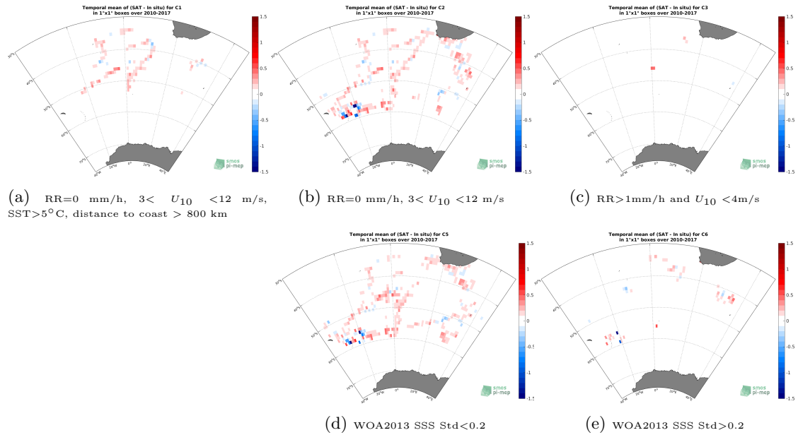
Figure 12: Temporal mean gridded over spatial boxes of size 1^{\circ}\times 1^{\circ} of \Delta\text{SSS} (CCI SSS L4 Merged-OI v2.31 - 7-day running (ESA) - TSG (NCEI-0170743)) for 5 different subdatasets corresponding to:RR=0 mm/h, 3 < U_{10} < 12 m/s, SST >5^{\circ}\text{C} , distance to coast > 800 km (a), RR=0 mm/h, 3 < U_{10} < 12 m/s (b), RR >1 mm/h and U_{10} < 4 m/s (c), WOA2013 SSS Std <0.2 (d), WOA2013 SSS Std >0.2 (e).
