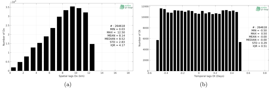
Figure 5: Histograms of the spatial (a) and temporal (b) lags between the time of the TSG (NCEI-0170743) measurements and the date of the corresponding CCI SSS L4 Merged-OI v2.31 - 7-day running (ESA) SSS product.
