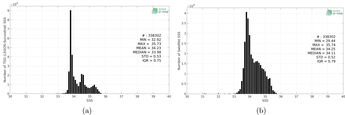
Figure 2: Histograms of SSS from TSG (LEGOS-Survostral) (a) and CCI SSS L4 Merged-OI v2.31 - 7-day running (ESA) (b) considering all match-up pairs per bins of 0.1 over the Global Ocean Pi-MEP region and for the full satellite product period.
