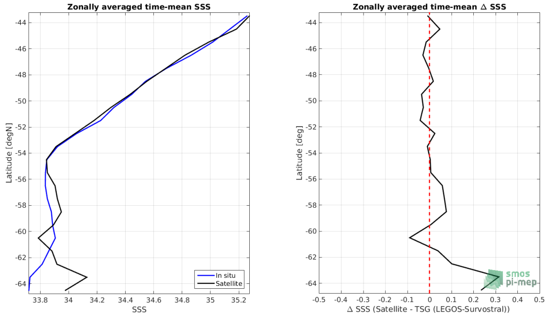
Figure 8: Left panel: Zonal mean SSS from CCI SSS L4 Merged-OI v2.31 - 7-day running (ESA) satellite product (black) and from TSG (LEGOS-Survostral) (blue). Right panel: Zonal mean of \Delta SSS (Satellite - TSG (LEGOS-Survostral)) for all the collected Pi-MEP match-up pairs estimated over the full satellite product period.
