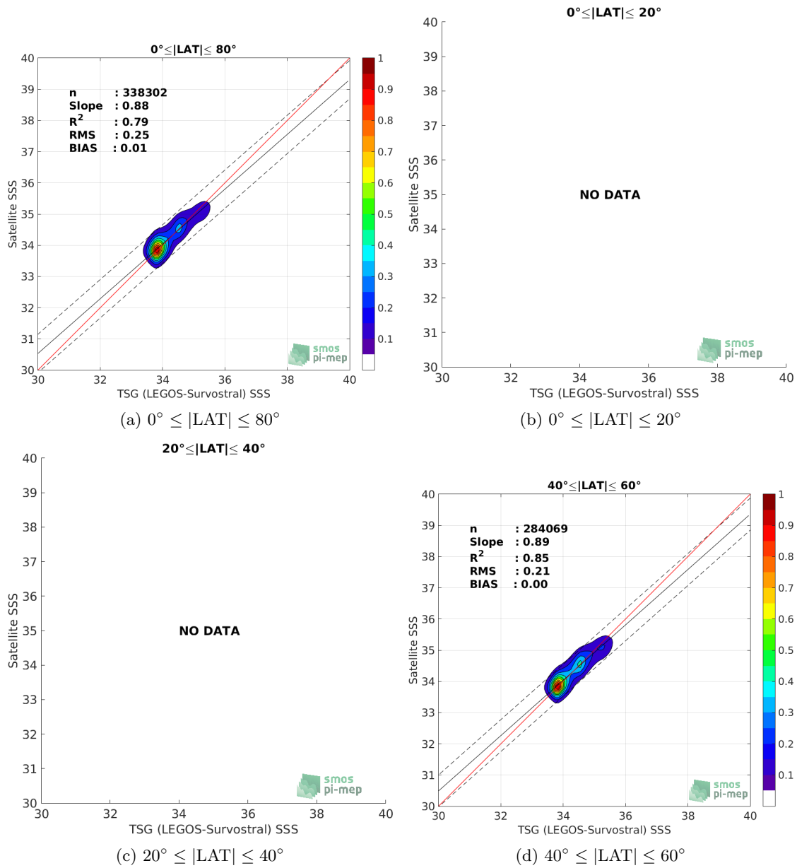
Figure 9: Contour maps of the concentration of CCI SSS L4 Merged-OI v2.31 - 7-day running (ESA) SSS (y-axis) versus TSG (LEGOS-Survostral) SSS (x-axis) at match-up pairs for different latitude bands. For each plot, the red line shows x=y . The black thin and dashed lines indicate a linear fit through the data cloud and the \pm 95\% confidence levels, respectively. The number match-up pairs n , the slope and R^2 coefficient of the linear fit, the root mean square (RMS) and the mean bias between satellite and in situ data are indicated for each latitude band in each plots.
