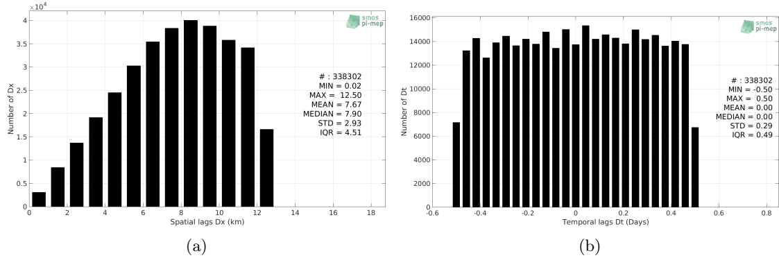
Figure 5: Histograms of the spatial (a) and temporal (b) lags between the time of the TSG (LEGOS-Survostral) measurements and the date of the corresponding CCI SSS L4 Merged-OI v2.31 - 7-day running (ESA) SSS product.
