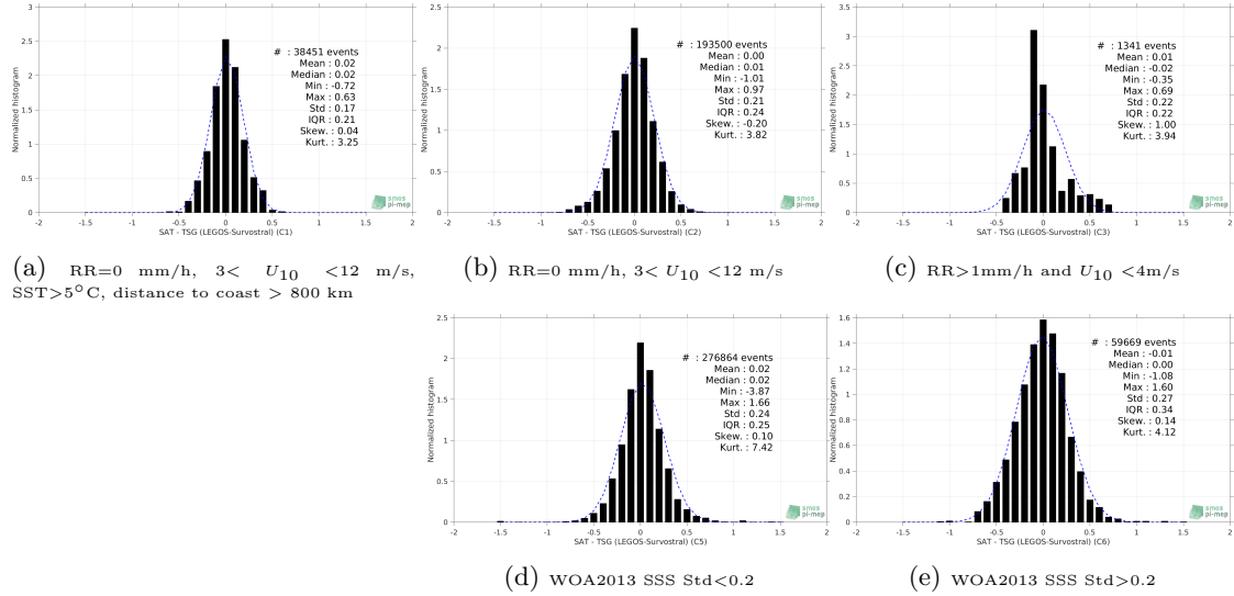
Figure 13: Normalized histogram of \Delta SSS (CCI SSS L4 Merged-OI v2.31 - 7-day running (ESA) - TSG (LEGOS-Survostral)) for 5 different subdatasets corresponding to: RR=0 mm/h, 3 < U_{10} < 12 m/s, SST > 5°C, distance to coast > 800 km (a), RR=0 mm/h, 3 < U_{10} < 12 m/s (b), RR > 1mm/h and U_{10} < 4 m/s (c), WOA2013 SSS Std < 0.2 (d), WOA2013 SSS Std > 0.2 (e).
