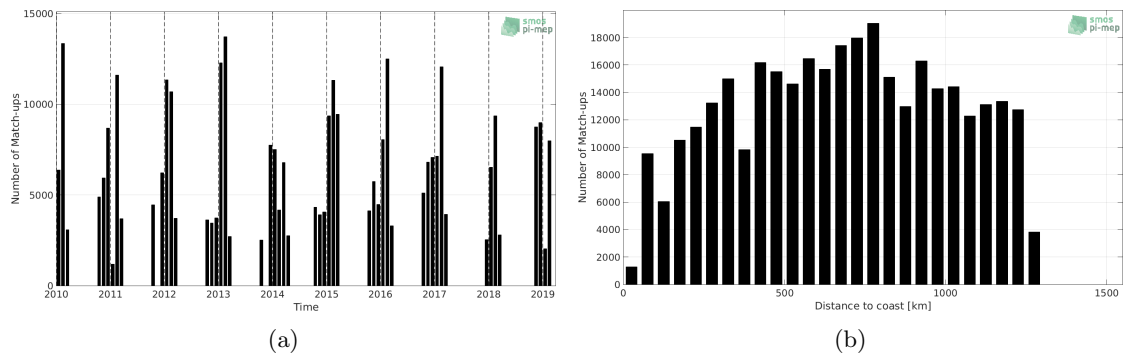
Figure 1: Number of match-ups between TSG (LEGOS-Survostral) and CCI SSS L4 Merged-OI v2.31 - 7-day running (ESA) SSS as a function of time (a) and as function of the distance to coast (b) over the Global Ocean Pi-MEP region and for the full satellite product period.
