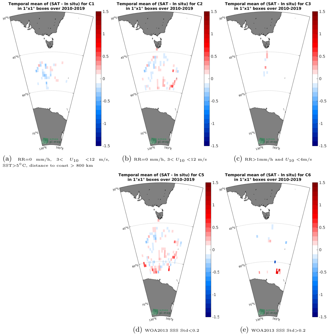
Figure 12: Temporal mean gridded over spatial boxes of size 1°x1° of \Delta SSS (CCI SSS L4 Merged-OI v2.31 - 7-day running (ESA) - TSG (LEGOS-Survostral)) for 5 different subdatasets corresponding to:RR=0 mm/h, 3 < U_{10} < 12 m/s, SST>5°C, distance to coast > 800 km (a), RR=0 mm/h, 3 < U_{10} < 12 m/s (b), RR>1mm/h and U_{10} < 4 m/s (c), WOA2013 SSS Std<0.2 (d), WOA2013 SSS Std>0.2 (e).
