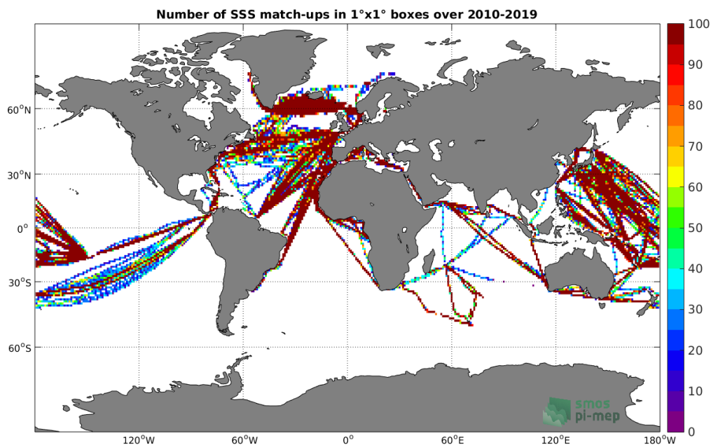
Figure 4: Number of SSS match-ups between TSG (LEGOS-DM) SSS and the CCI SSS L4 Merged-OI v2.31 - 7-day running (ESA) SSS product for the Global Ocean Pi-MEP region over 1^\circ \times 1^\circ boxes and for the full satellite product period.
