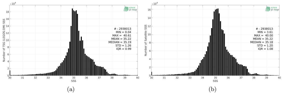
Figure 2: Histograms of SSS from TSG (LEGOS-DM) (a) and CCI SSS L4 Merged-OI v2.31 - 7-day running (ESA) (b) considering all match-up pairs per bins of 0.1 over the Global Ocean Pi-MEP region and for the full satellite product period.
