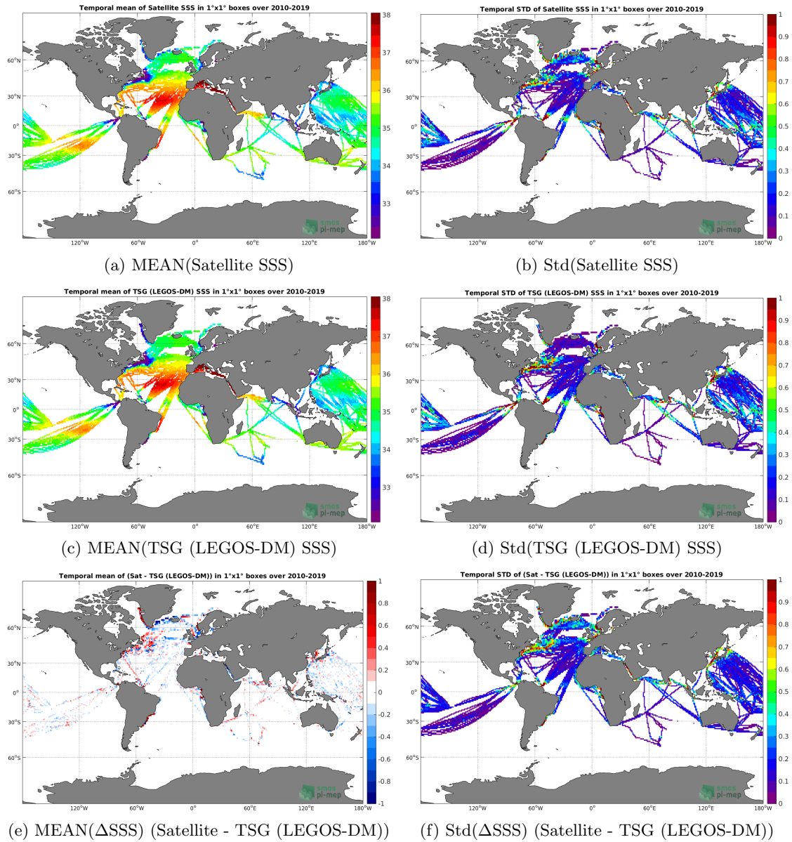
Figure 6: Temporal mean (left) and Std (right) of SSS from CCI SSS L4 Merged-OI v2.31 - 7-day running (ESA) (top), TSG (LEGOS-DM) (middle), and of \Delta SSS (Satellite - TSG (LEGOS-DM)). Only match-up pairs are used to generate these maps.
