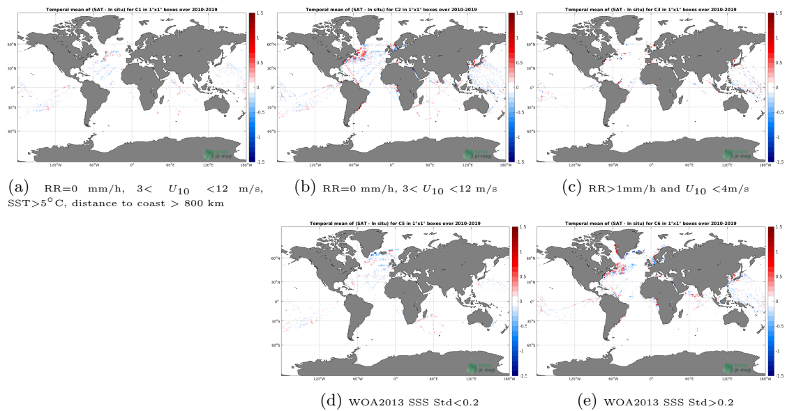
Figure 12: Temporal mean gridded over spatial boxes of size 1^\circ \times 1^\circ of \Delta SSS (CCI SSS L4 Merged-OI v2.31 - 7-day running (ESA) - TSG (LEGOS-DM)) for 5 different subdatasets corresponding to: RR=0 mm/h, 3 < U_{10} < 12 m/s, SST >5^\circ C, distance to coast > 800 km (a), RR=0 mm/h, 3 < U_{10} < 12 m/s (b), RR >1 mm/h and U_{10} < 4 m/s (c), WOA2013 SSS Std <0.2 (d), WOA2013 SSS Std >0.2 (e).
