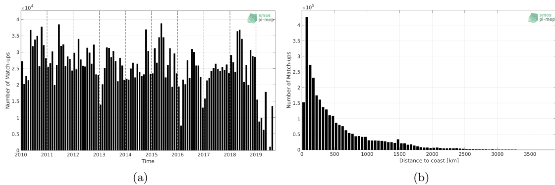
Figure 1: Number of match-ups between TSG (LEGOS-DM) and CCI SSS L4 Merged-OI v2.31 - 7-day running (ESA) SSS as a function of time (a) and as function of the distance to coast (b) over the Global Ocean Pi-MEP region and for the full satellite product period.
