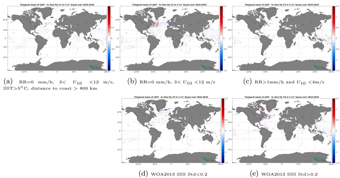
Figure 12: Temporal mean gridded over spatial boxes of size 1^\circ \times 1^\circ of \Delta SSS (CCI L4 Merged-OI v2.31 - 7-day running (ESA) - TSG (LEGOS-DM)) for 5 different subdatasets corresponding to:RR=0 mm/h, 3 < U_{10} < 12 m/s, SST >5^\circ\text{C} , distance to coast > 800 km (a), RR=0 mm/h, 3 < U_{10} < 12 m/s (b), RR >1 mm/h and U_{10} < 4 m/s (c), WOA2013 SSS Std <0.2 (d), WOA2013 SSS Std >0.2 (e).
