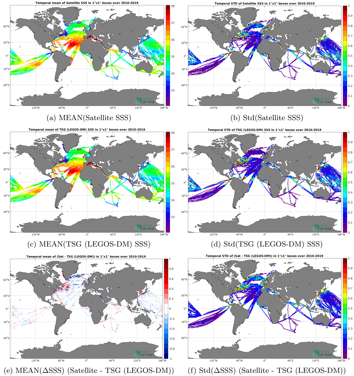
Figure 6: Temporal mean (left) and Std (right) of SSS from CCI L4 Merged-OI v2.31 - 7-day running (ESA) (top), TSG (LEGOS-DM) (middle), and of \Delta SSS (Satellite - TSG (LEGOS-DM)). Only match-up pairs are used to generate these maps.
