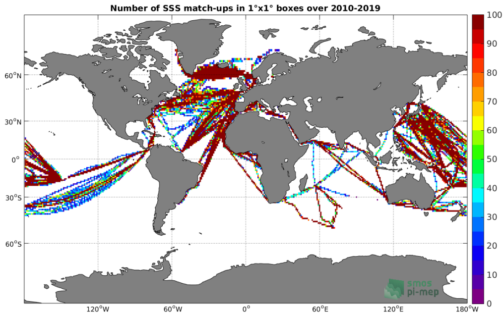
Figure 4: Number of SSS match-ups between TSG (LEGOS-DM) SSS and the CCI L4 Merged-OI v2.31 - 7-day running (ESA) SSS product for the Global Ocean Pi-MEP region over 1°x1° boxes and for the full satellite product period.
