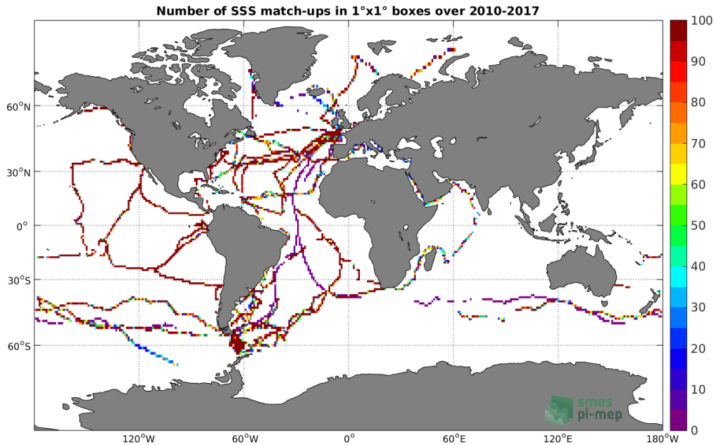
Figure 4: Number of SSS match-ups between TSG (GOSUD-Sailing-ship) SSS and the CCI SSS L4 Merged-OI v2.31 - 7-day running (ESA) SSS product for the Global Ocean Pi-MEP region over 1°x1° boxes and for the full satellite product period.
