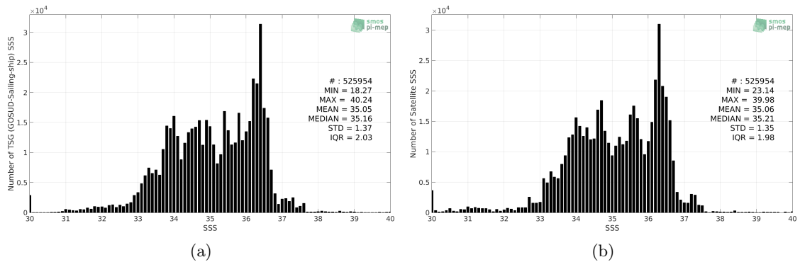
Figure 2: Histograms of SSS from TSG (GOSUD-Sailing-ship) (a) and CCI SSS L4 Merged-OI v2.31 - 7-day running (ESA) (b) considering all match-up pairs per bins of 0.1 over the Global Ocean Pi-MEP region and for the full satellite product period.
