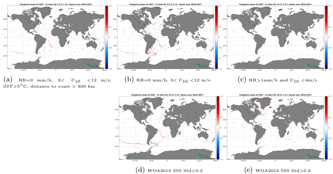
Figure 12: Temporal mean gridded over spatial boxes of size 1^\circ \times 1^\circ of \Delta SSS (CCI SSS L4 Merged-OI v2.31 - 7-day running (ESA) - TSG (GOSUD-Sailing-ship)) for 5 different subdatasets corresponding to:RR=0 mm/h, 3 < U_{10} < 12 m/s, SST>5°C, distance to coast > 800 km (a), RR=0 mm/h, 3 < U_{10} < 12 m/s (b), RR>1mm/h and U_{10} < 4 m/s (c), WOA2013 SSS Std<0.2 (d), WOA2013 SSS Std>0.2 (e).
