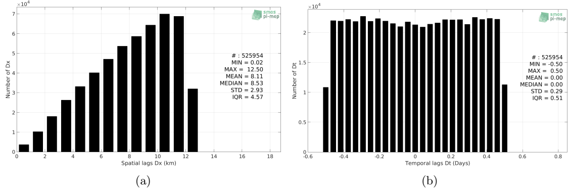
Figure 5: Histograms of the spatial (a) and temporal (b) lags between the time of the TSG (GOSUD-Sailing-ship) measurements and the date of the corresponding CCI SSS L4 Merged-OI v2.31 - 7-day running (ESA) SSS product.
