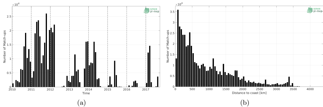
Figure 1: Number of match-ups between TSG (GOSUD-Sailing-ship) and CCI SSS L4 Merged-OI v2.31 - 7-day running (ESA) SSS as a function of time (a) and as function of the distance to coast (b) over the Global Ocean Pi-MEP region and for the full satellite product period.
