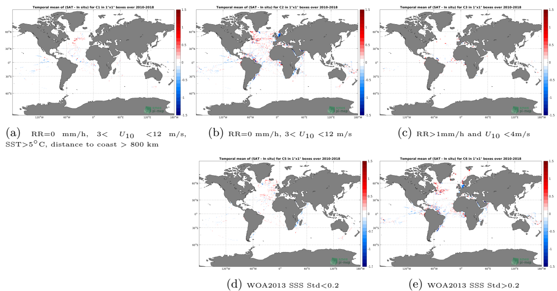
Figure 12: Temporal mean gridded over spatial boxes of size 1^\circ \times 1^\circ of \Delta SSS (CCI SSS L4 Merged-OI v2.31 - 7-day running (ESA) - TSG (GOSUD-Research-vessel)) for 5 different subdatasets corresponding to:RR=0 mm/h, 3 < U_{10} < 12 m/s, SST>5°C, distance to coast > 800 km (a), RR=0 mm/h, 3 < U_{10} < 12 m/s (b), RR>1mm/h and U_{10} < 4 m/s (c), WOA2013 SSS Std<0.2 (d), WOA2013 SSS Std>0.2 (e).
