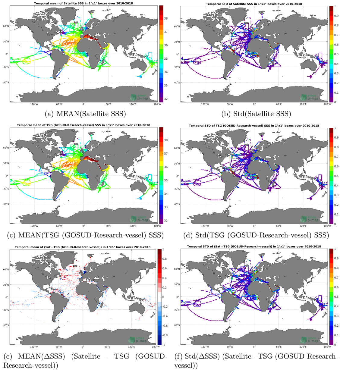
Figure 6: Temporal mean (left) and Std (right) of SSS from CCI SSS L4 Merged-OI v2.31 - 7-day running (ESA) (top), TSG (GOSUD-Research-vessel) (middle), and of \Delta SSS (Satellite - TSG (GOSUD-Research-vessel)). Only match-up pairs are used to generate these maps.
