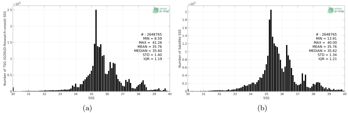
Figure 2: Histograms of SSS from TSG (GOSUD-Research-vessel) (a) and CCI SSS L4 Merged-OI v2.31 - 7-day running (ESA) (b) considering all match-up pairs per bins of 0.1 over the Global Ocean Pi-MEP region and for the full satellite product period.
