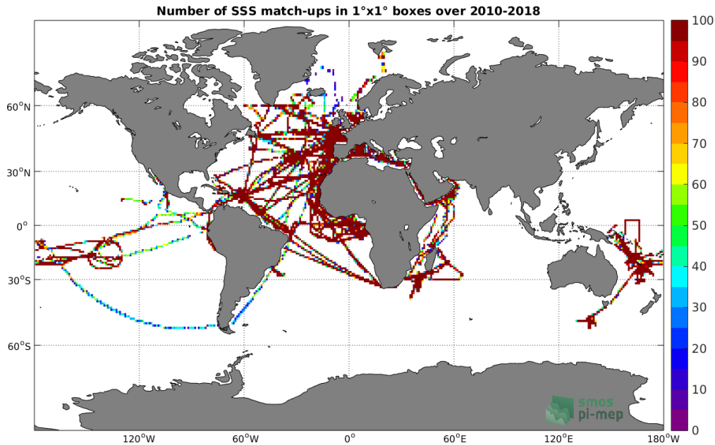
Figure 4: Number of SSS match-ups between TSG (GOSUD-Research-vessel) SSS and the CCI SSS L4 Merged-OI v2.31 - 7-day running (ESA) SSS product for the Global Ocean Pi-MEP region over 1^\circ \times 1^\circ boxes and for the full satellite product period.
