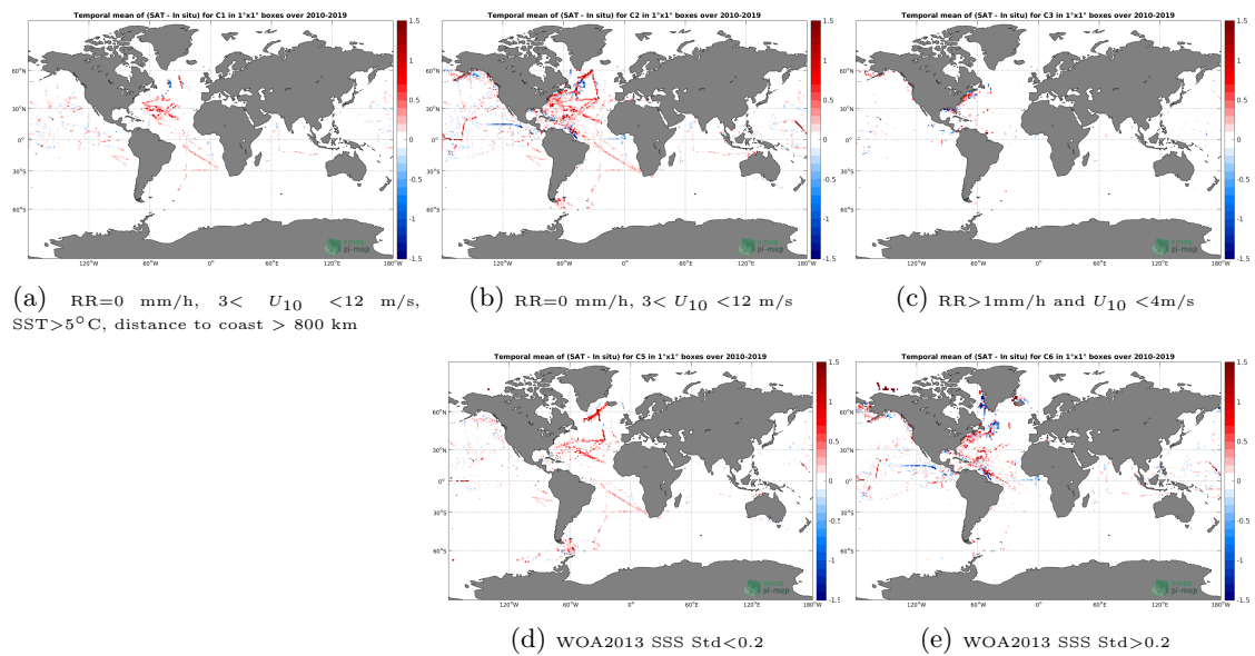
Figure 12: Temporal mean gridded over spatial boxes of size 1^\circ \times 1^\circ of \Delta SSS (CCI SSS L4 Merged-OI v2.31 - 30-day running (ESA) - TSG (SAMOS)) for 5 different subdatasets corresponding to:RR=0 mm/h, 3 < U_{10} < 12 m/s, SST >5^\circ\text{C} , distance to coast > 800 km (a), RR=0 mm/h, 3 < U_{10} < 12 m/s (b), RR >1 mm/h and U_{10} < 4 m/s (c), WOA2013 SSS Std <0.2 (d), WOA2013 SSS Std >0.2 (e).
