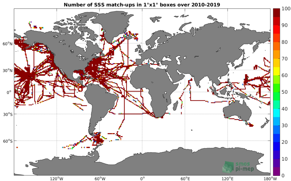
Figure 4: Number of SSS match-ups between TSG (SAMOS) SSS and the CCI SSS L4 Merged-OI v2.31 - 30-day running (ESA) SSS product for the Global Ocean Pi-MEP region over 1°x1° boxes and for the full satellite product period.
