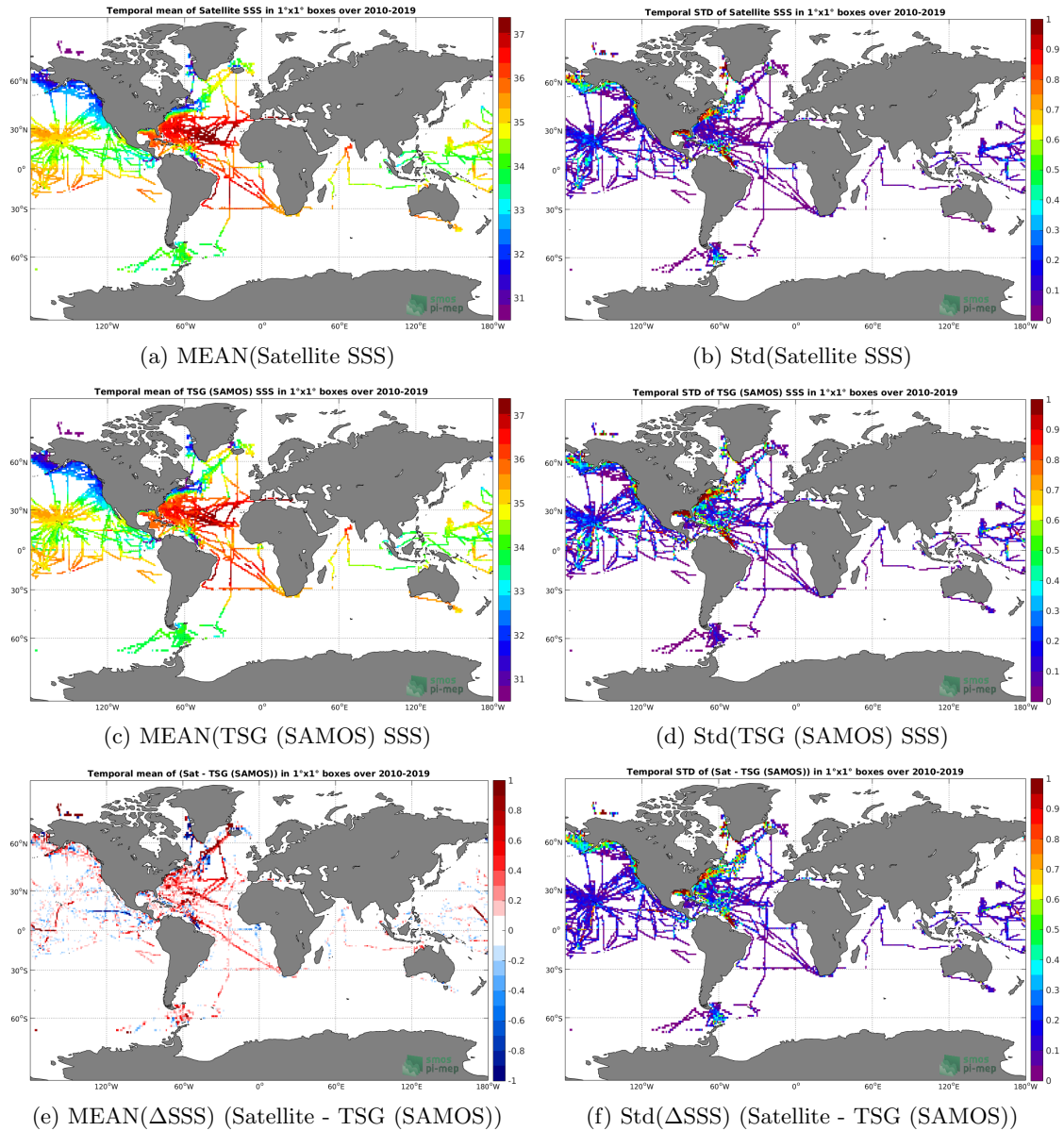
Figure 6: Temporal mean (left) and Std (right) of SSS from CCI SSS L4 Merged-OI v2.31 - 30-day running (ESA) (top), TSG (SAMOS) (middle), and of \Delta SSS (Satellite - TSG (SAMOS)). Only match-up pairs are used to generate these maps.
