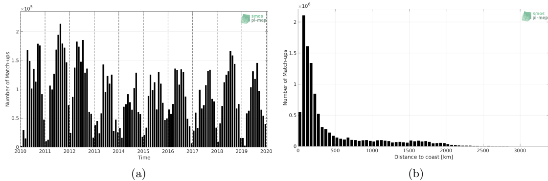
Figure 1: Number of match-ups between TSG (SAMOS) and CCI SSS L4 Merged-OI v2.31 - 30-day running (ESA) SSS as a function of time (a) and as function of the distance to coast (b) over the Global Ocean Pi-MEP region and for the full satellite product period.
