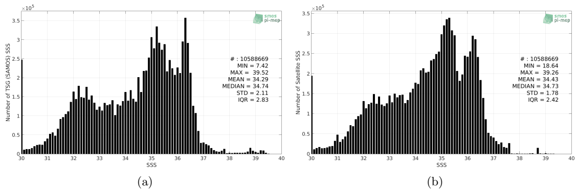
Figure 2: Histograms of SSS from TSG (SAMOS) (a) and CCI SSS L4 Merged-OI v2.31 - 30-day running (ESA) (b) considering all match-up pairs per bins of 0.1 over the Global Ocean Pi-MEP region and for the full satellite product period.
