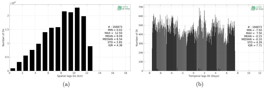
Figure 5: Histograms of the spatial (a) and temporal (b) lags between the location/time of the TSG (Polarstern) measurement and the date of the corresponding CCI SSS L4 Merged-OI v2.31 - 30-day running (ESA) SSS pixel.
