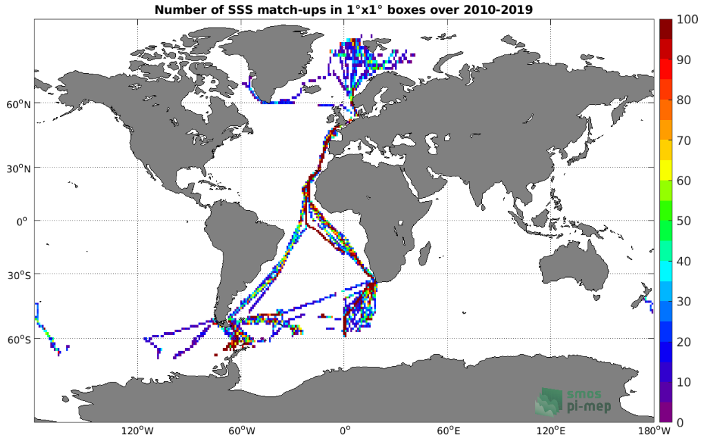
Figure 4: Number of SSS match-ups between TSG (Polarstern) SSS and the CCI SSS L4 Merged-OI v2.31 - 30-day running (ESA) SSS product for the Global Ocean Pi-MEP region over 1^\circ \times 1^\circ boxes and for the full satellite product period.
