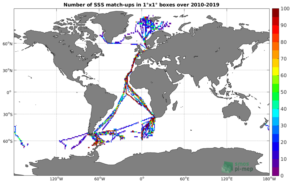
Figure 4: Number of SSS match-ups between TSG (Polarstern) SSS and the CCI SSS L4 Merged-OI v2.31 - 30-day running (ESA) SSS product for the Global Ocean Pi-MEP region over 1°x1° boxes and for the full satellite product period.
