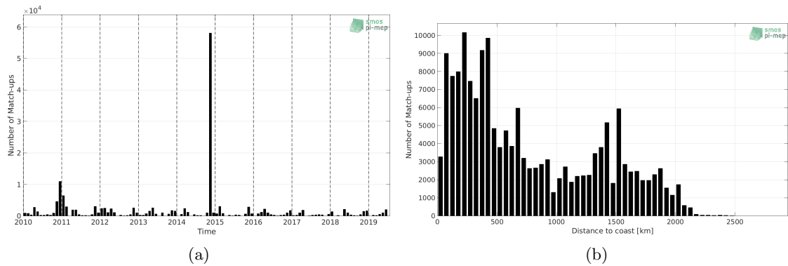
Figure 1: Number of match-ups between TSG (Polarstern) and CCI SSS L4 Merged-OI v2.31 - 30-day running (ESA) SSS as a function of time (a) and as function of the distance to coast (b) over the Global Ocean Pi-MEP region and for the full satellite product period.
