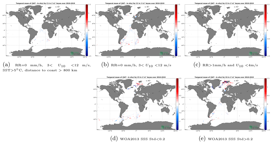
Figure 12: Temporal mean gridded over spatial boxes of size 1^\circ \times 1^\circ of \Delta SSS (CCI SSS L4 Merged-OI v2.31 - 30-day running (ESA) - TSG (Polarstern)) for 5 different subdatasets corresponding to:RR=0 mm/h, 3 < U_{10} < 12 m/s, SST >5^\circ C, distance to coast > 800 km (a), RR=0 mm/h, 3 < U_{10} < 12 m/s (b), RR >1 mm/h and U_{10} < 4 m/s (c), WOA2013 SSS Std <0.2 (d), WOA2013 SSS Std >0.2 (e).
