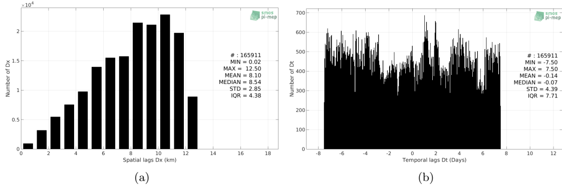
Figure 5: Histograms of the spatial (a) and temporal (b) lags between the time of the TSG (Polarstern) measurements and the date of the corresponding CCI SSS L4 Merged-OI v2.31 - 30-day running (ESA) SSS product.
