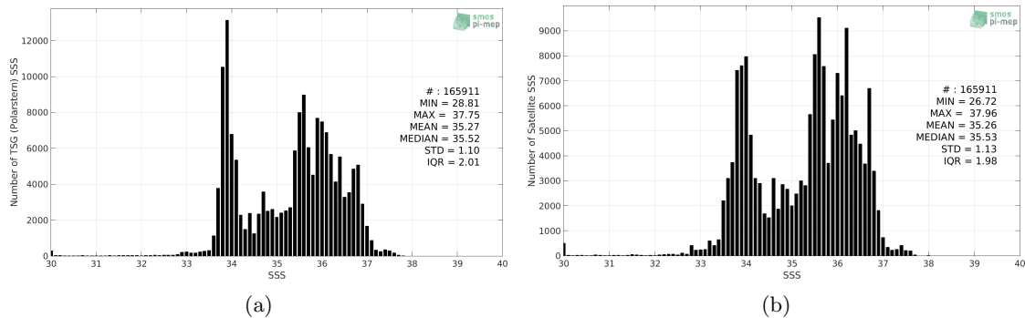
Figure 2: Histograms of SSS from TSG (Polarstern) (a) and CCI SSS L4 Merged-OI v2.31 - 30-day running (ESA) (b) considering all match-up pairs per bins of 0.1 over the Global Ocean Pi-MEP region and for the full satellite product period.
