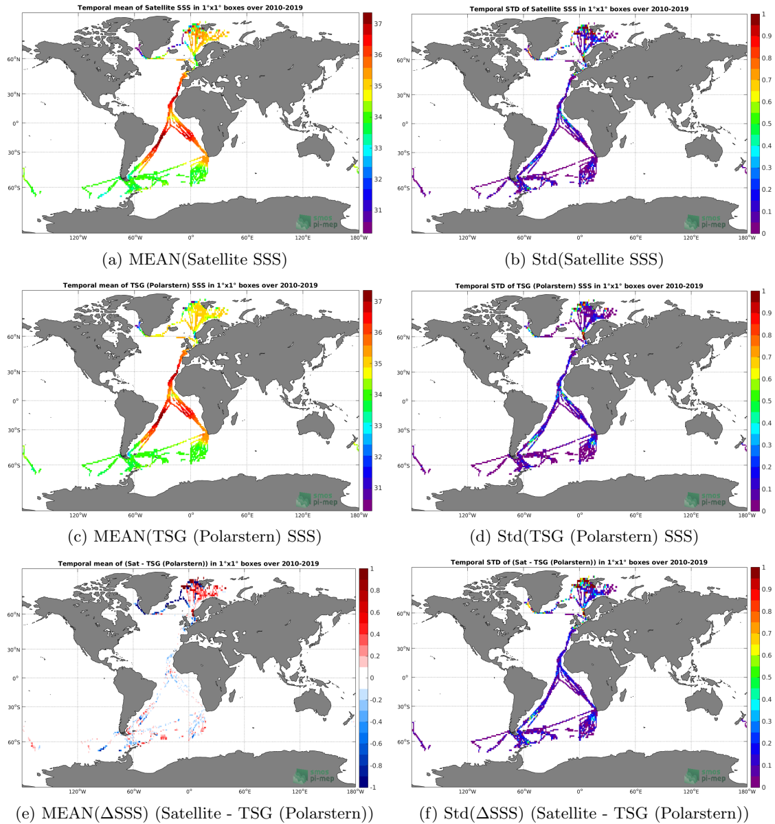
Figure 6: Temporal mean (left) and Std (right) of SSS from CCI SSS L4 Merged-OI v2.31 - 30-day running (ESA) (top), TSG (Polarstern) (middle), and of \Delta SSS (Satellite - TSG (Polarstern)). Only match-up pairs are used to generate these maps.
