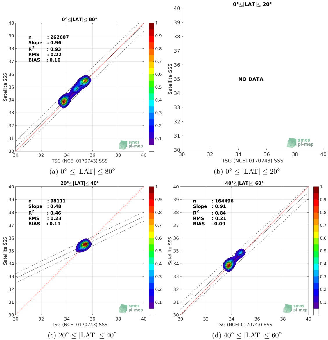
Figure 9: Contour maps of the concentration of CCI SSS L4 Merged-OI v2.31 - 30-day running (ESA) SSS ( y -axis) versus TSG (NCEI-0170743) SSS ( x -axis) at match-up pairs for different latitude bands. For each plot, the red line shows x=y . The black thin and dashed lines indicate a linear fit through the data cloud and the \pm 95\% confidence levels, respectively. The number match-up pairs n , the slope and R^2 coefficient of the linear fit, the root mean square (RMS) and the mean bias between satellite and in situ data are indicated for each latitude band in each plots.
