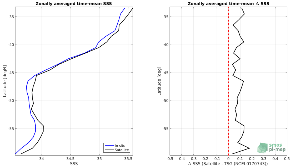
Figure 8: Left panel: Zonal mean SSS from CCI SSS L4 Merged-OI v2.31 - 30-day running (ESA) satellite product (black) and from TSG (NCEI-0170743) (blue). Right panel: Zonal mean of \Delta SSS (Satellite - TSG (NCEI-0170743)) for all the collected Pi-MEP match-up pairs estimated over the full satellite product period.
