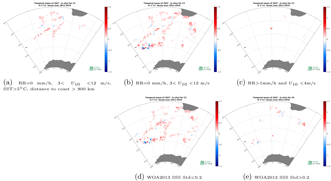
Figure 12: Temporal mean gridded over spatial boxes of size 1^{\circ}\times 1^{\circ} of \Delta\text{SSS} (CCI SSS L4 Merged-OI v2.31 - 30-day running (ESA) - TSG (NCEI-0170743)) for 5 different subdatasets corresponding to:RR=0 mm/h, 3 < U_{10} < 12 m/s, SST >5^{\circ}\text{C} , distance to coast > 800 km (a), RR=0 mm/h, 3 < U_{10} < 12 m/s (b), RR >1 mm/h and U_{10} < 4 m/s (c), WOA2013 SSS Std <0.2 (d), WOA2013 SSS Std >0.2 (e).
