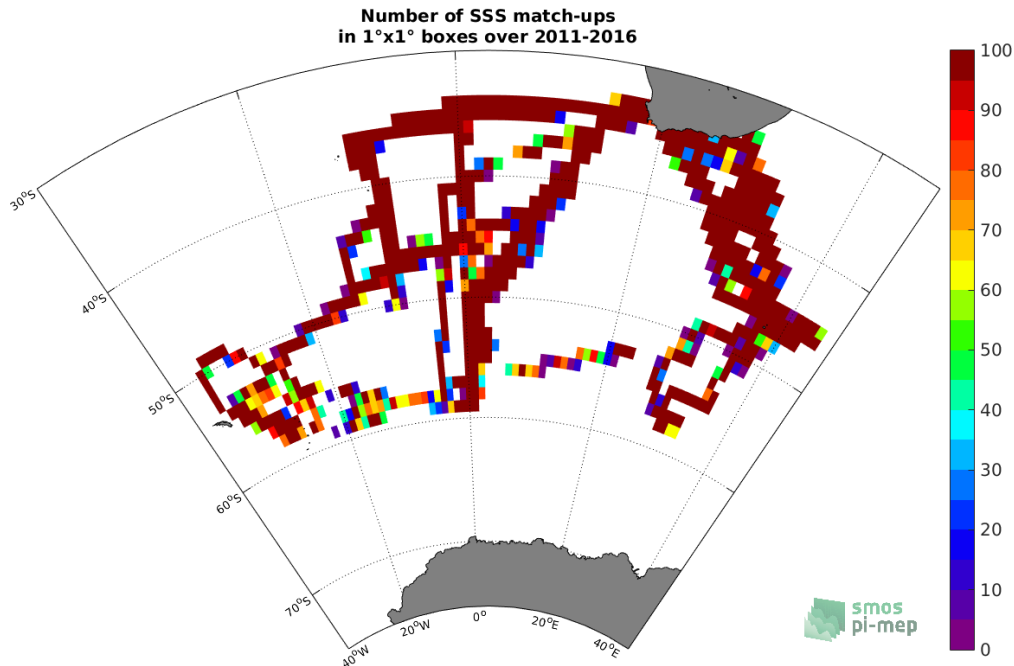
Figure 4: Number of SSS match-ups between TSG (NCEI-0170743) SSS and the CCI SSS L4 Merged-OI v2.31 - 30-day running (ESA) SSS product for the Global Ocean Pi-MEP region over 1°x1° boxes and for the full satellite product period.
