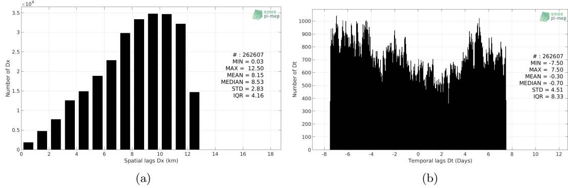
Figure 5: Histograms of the spatial (a) and temporal (b) lags between the time of the TSG (NCEI-0170743) measurements and the date of the corresponding CCI SSS L4 Merged-OI v2.31 - 30-day running (ESA) SSS product.
