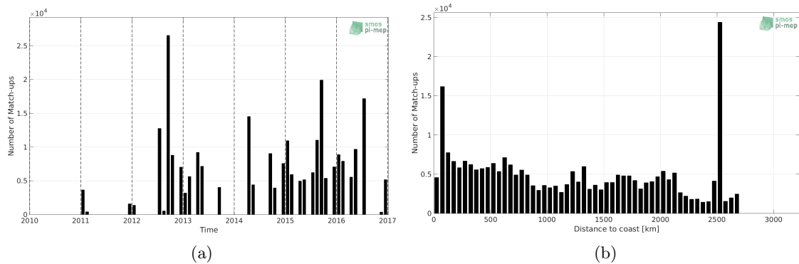
Figure 1: Number of match-ups between TSG (NCEI-0170743) and CCI SSS L4 Merged-OI v2.31 - 30-day running (ESA) SSS as a function of time (a) and as function of the distance to coast (b) over the Global Ocean Pi-MEP region and for the full satellite product period.
