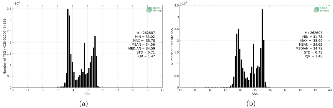
Figure 2: Histograms of SSS from TSG (NCEI-0170743) (a) and CCI SSS L4 Merged-OI v2.31 - 30-day running (ESA) (b) considering all match-up pairs per bins of 0.1 over the Global Ocean Pi-MEP region and for the full satellite product period.
