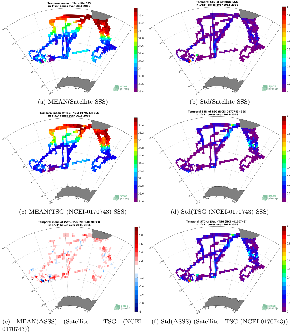
Figure 6: Temporal mean (left) and Std (right) of SSS from CCI SSS L4 Merged-OI v2.31 - 30-day running (ESA) (top), TSG (NCEI-0170743) (middle), and of \Delta SSS (Satellite - TSG (NCEI-0170743)). Only match-up pairs are used to generate these maps.
