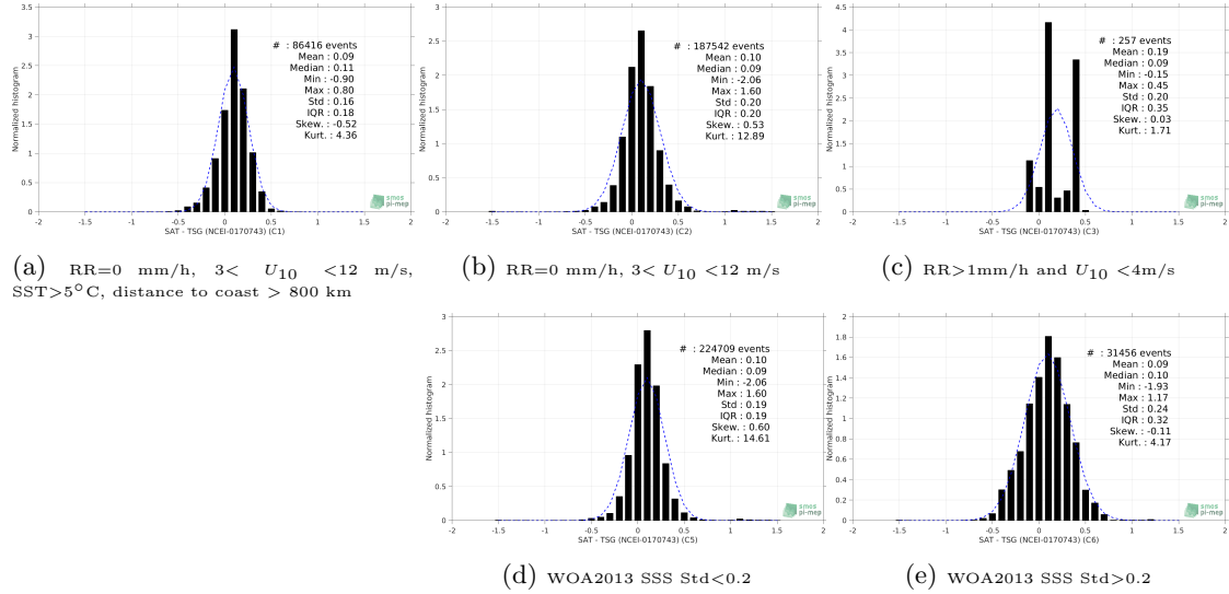
Figure 13: Normalized histogram of \Delta SSS (CCI SSS L4 Merged-OI v2.31 - 30-day running (ESA) - TSG (NCEI-0170743)) for 5 different subdatasets corresponding to: RR=0 mm/h, 3 < U_{10} < 12 m/s, SST>5°C, distance to coast > 800 km (a), RR=0 mm/h, 3 < U_{10} < 12 m/s (b), RR>1mm/h and U_{10} < 4 m/s (c), WOA2013 SSS Std<0.2 (d), WOA2013 SSS Std>0.2 (e).
