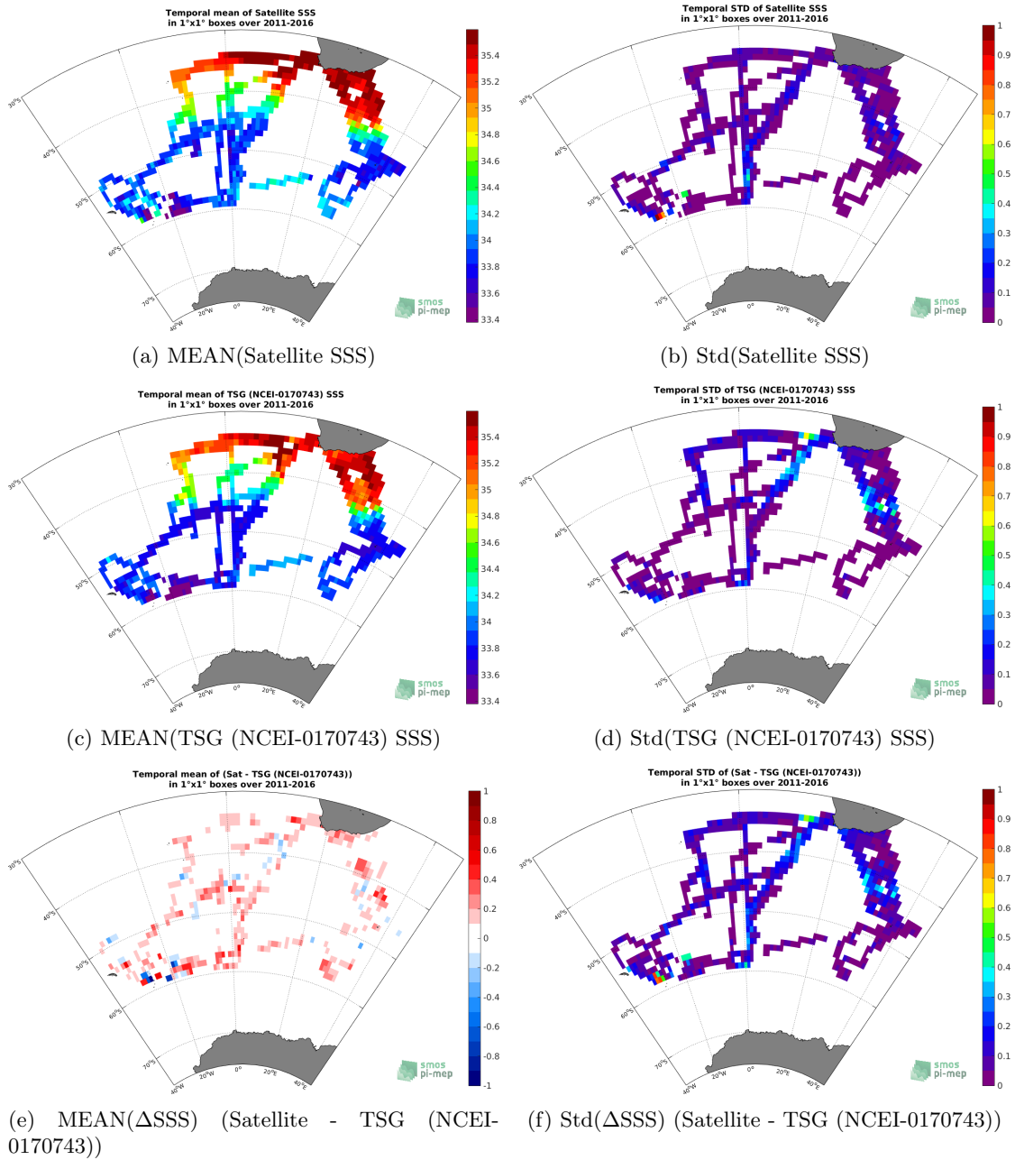
Figure 6: Temporal mean (left) and Std (right) of SSS from CCI L4 Merged-OI v2.31 - 30-day running (ESA) (top), TSG (NCEI-0170743) (middle), and of \Delta SSS (Satellite - TSG (NCEI-0170743)). Only match-up pairs are used to generate these maps.
