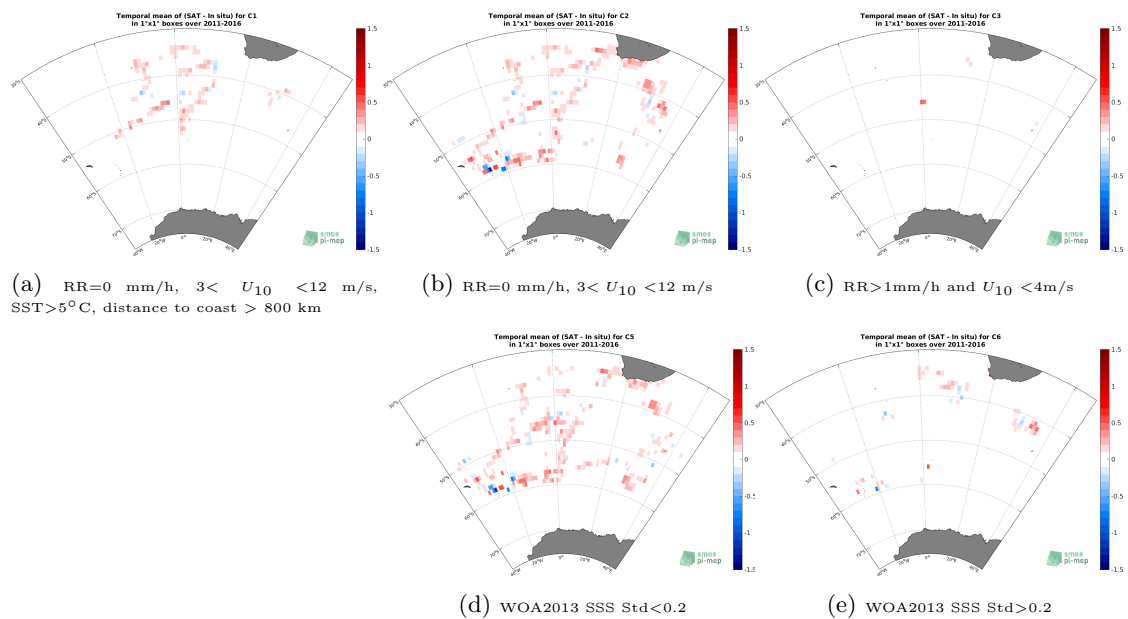
Figure 12: Temporal mean gridded over spatial boxes of size 1^\circ \times 1^\circ of \Delta SSS (CCI L4 Merged-OI v2.31 - 30-day running (ESA) - TSG (NCEI-0170743)) for 5 different subdatasets corresponding to:RR=0 mm/h, 3 < U_{10} < 12 m/s, SST >5^\circ\text{C} , distance to coast > 800 km (a), RR=0 mm/h, 3 < U_{10} < 12 m/s (b), RR >1 mm/h and U_{10} < 4 m/s (c), WOA2013 SSS Std <0.2 (d), WOA2013 SSS Std >0.2 (e).
