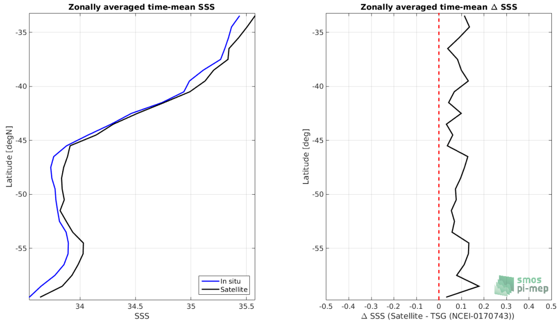
Figure 8: Left panel: Zonal mean SSS from CCI L4 Merged-OI v2.31 - 30-day running (ESA) satellite product (black) and from TSG (NCEI-0170743) (blue). Right panel: Zonal mean of \Delta SSS (Satellite - TSG (NCEI-0170743)) for all the collected Pi-MEP match-up pairs estimated over the full satellite product period.
