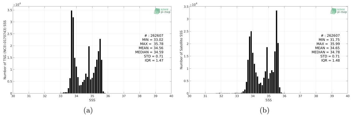
Figure 2: Histograms of SSS from TSG (NCEI-0170743) (a) and CCI L4 Merged-OI v2.31 - 30-day running (ESA) (b) considering all match-up pairs per bins of 0.1 over the Global Ocean Pi-MEP region and for the full satellite product period.
