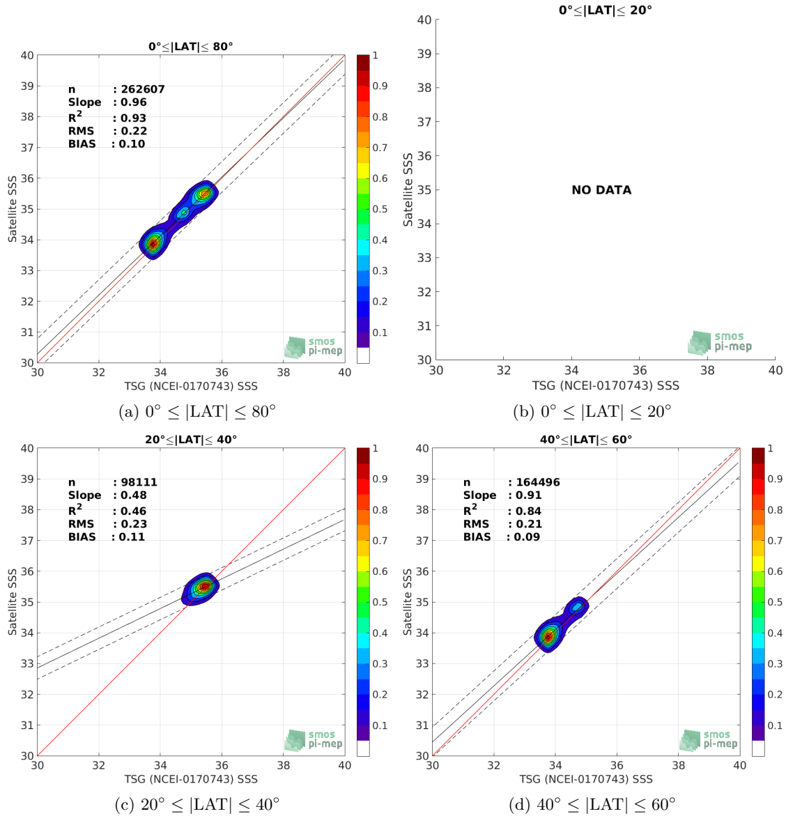
Figure 9: Contour maps of the concentration of CCI L4 Merged-OI v2.31 - 30-day running (ESA) SSS (y-axis) versus TSG (NCEI-0170743) SSS (x-axis) at match-up pairs for different latitude bands. For each plot, the red line shows x=y . The black thin and dashed lines indicate a linear fit through the data cloud and the \pm 95\% confidence levels, respectively. The number match-up pairs n , the slope and R^2 coefficient of the linear fit, the root mean square (RMS) and the mean bias between satellite and in situ data are indicated for each latitude band in each plots.
