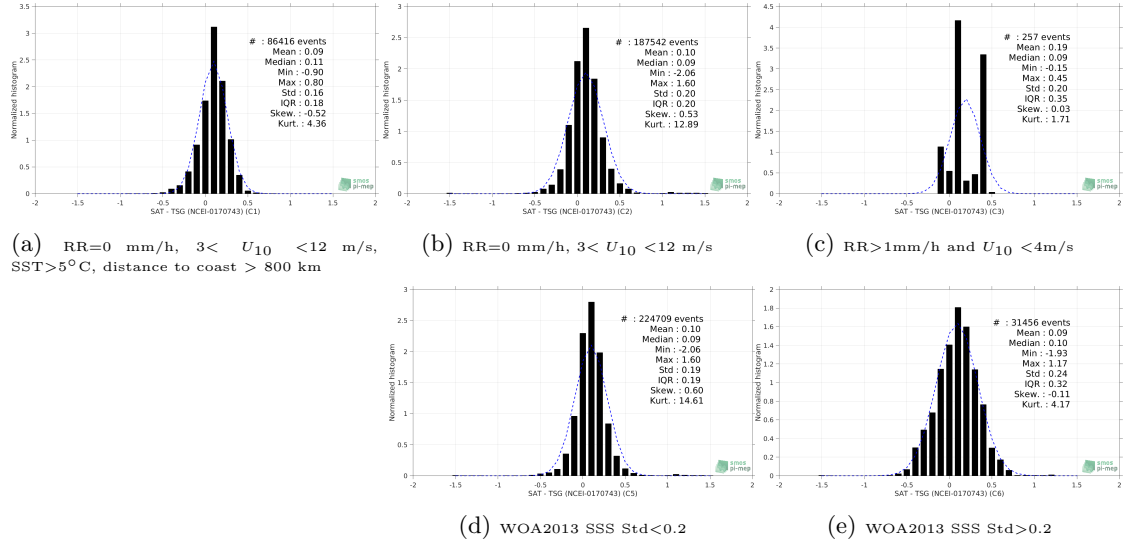
Figure 13: Normalized histogram of \Delta SSS (CCI L4 Merged-OI v2.31 - 30-day running (ESA) - TSG (NCEI-0170743)) for 5 different subdatasets corresponding to: RR=0 mm/h, 3 < U_{10} < 12 m/s, SST>5°C, distance to coast > 800 km (a), RR=0 mm/h, 3 < U_{10} < 12 m/s (b), RR>1mm/h and U_{10} < 4 m/s (c), WOA2013 SSS Std<0.2 (d), WOA2013 SSS Std>0.2 (e).
