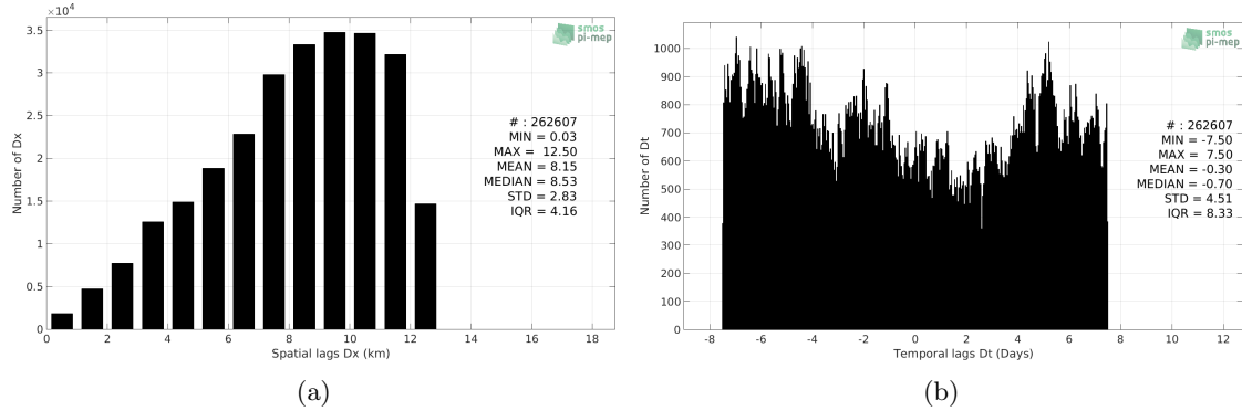
Figure 5: Histograms of the spatial (a) and temporal (b) lags between the time of the TSG (NCEI-0170743) measurements and the date of the corresponding CCI L4 Merged-OI v2.31 - 30-day running (ESA) SSS product.
