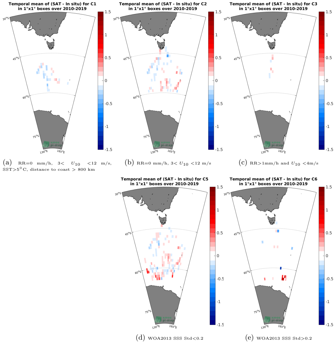
Figure 12: Temporal mean gridded over spatial boxes of size 1°x1° of \Delta SSS (CCI L4 Merged-OI v2.31 - 30-day running (ESA) - TSG (LEGOS-Survostral)) for 5 different subdatasets corresponding to:RR=0 mm/h, 3 < U_{10} < 12 m/s, SST>5°C, distance to coast > 800 km (a), RR=0 mm/h, 3 < U_{10} < 12 m/s (b), RR>1mm/h and U_{10} < 4 m/s (c), WOA2013 SSS Std<0.2 (d), WOA2013 SSS Std>0.2 (e).
