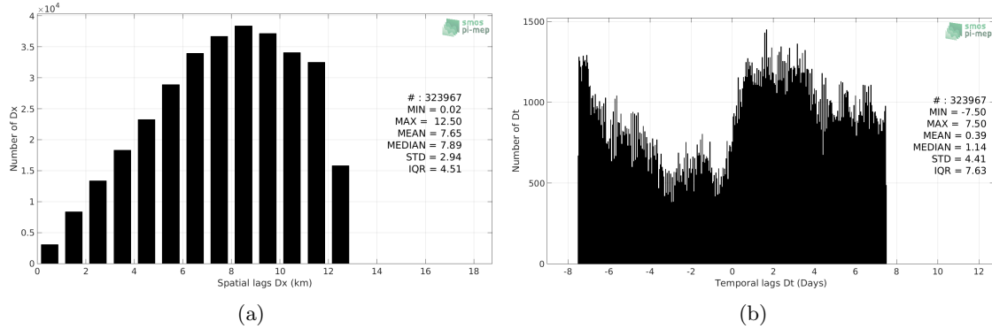
Figure 5: Histograms of the spatial (a) and temporal (b) lags between the time of the TSG (LEGOS-Survostral) measurements and the date of the corresponding CCI L4 Merged-OI v2.31 - 30-day running (ESA) SSS product.
