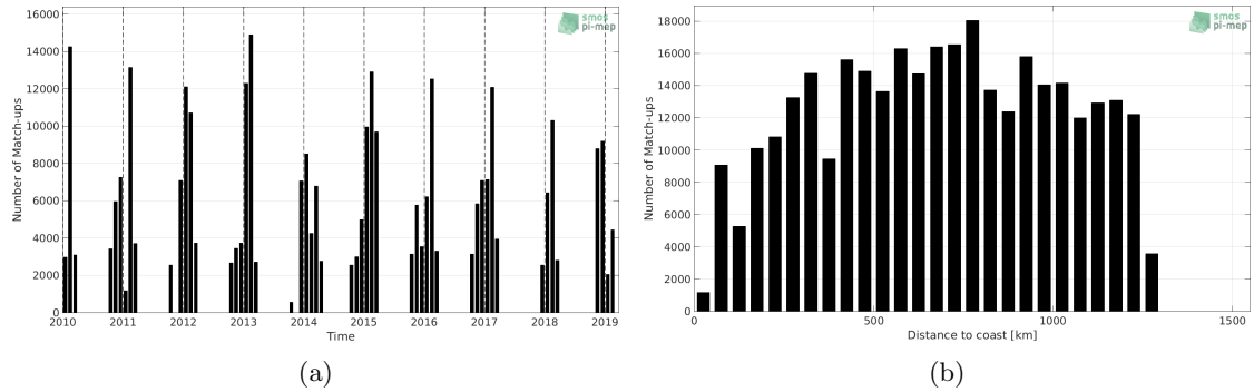
Figure 1: Number of match-ups between TSG (LEGOS-Survostral) and CCI L4 Merged-OI v2.31 - 30-day running (ESA) SSS as a function of time (a) and as function of the distance to coast (b) over the Global Ocean Pi-MEP region and for the full satellite product period.
