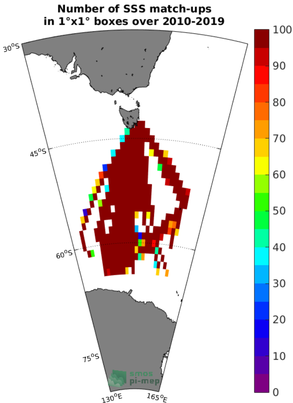
Figure 4: Number of SSS match-ups between TSG (LEGOS-Survostral) SSS and the CCI L4 Merged-OI v2.31 - 30-day running (ESA) SSS product for the Global Ocean Pi-MEP region over 1°x1° boxes and for the full satellite product period.
