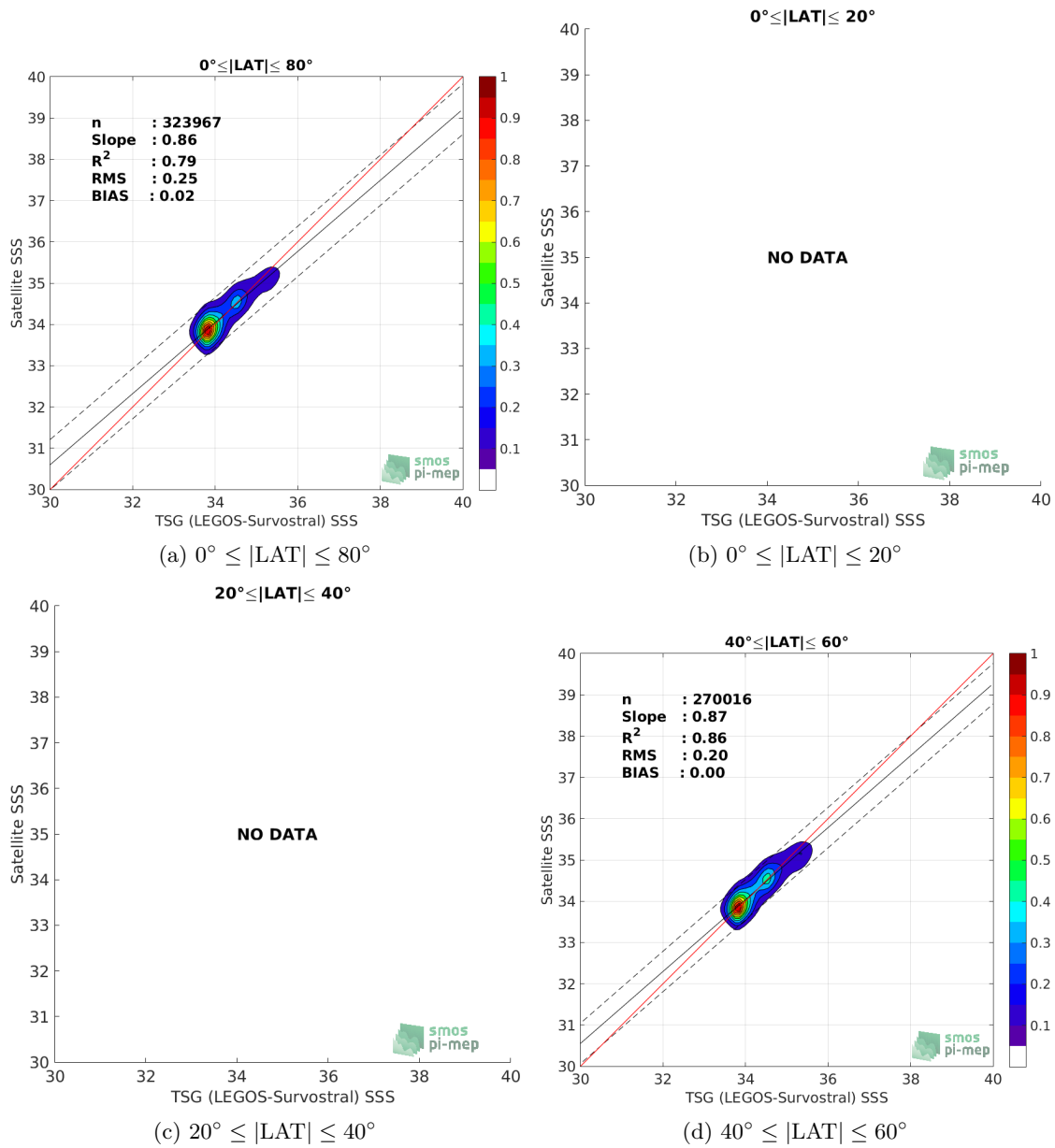
Figure 9: Contour maps of the concentration of CCI L4 Merged-OI v2.31 - 30-day running (ESA) SSS (y-axis) versus TSG (LEGOS-Survostral) SSS (x-axis) at match-up pairs for different latitude bands. For each plot, the red line shows x=y . The black thin and dashed lines indicate a linear fit through the data cloud and the \pm 95\% confidence levels, respectively. The number match-up pairs n , the slope and R^2 coefficient of the linear fit, the root mean square (RMS) and the mean bias between satellite and in situ data are indicated for each latitude band in each plots.
