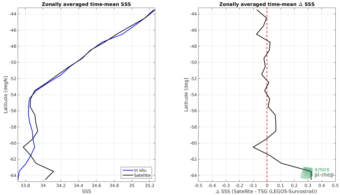
Figure 8: Left panel: Zonal mean SSS from CCI L4 Merged-OI v2.31 - 30-day running (ESA) satellite product (black) and from TSG (LEGOS-Survostral) (blue). Right panel: Zonal mean of \Delta SSS (Satellite - TSG (LEGOS-Survostral)) for all the collected Pi-MEP match-up pairs estimated over the full satellite product period.
