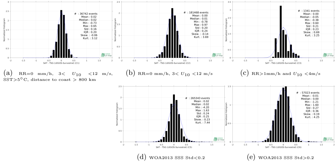
Figure 13: Normalized histogram of \Delta SSS (CCI L4 Merged-OI v2.31 - 30-day running (ESA) - TSG (LEGOS-Survostral)) for 5 different subdatasets corresponding to: RR=0 mm/h, 3 < U_{10} < 12 m/s, SST>5°C, distance to coast > 800 km (a), RR=0 mm/h, 3 < U_{10} < 12 m/s (b), RR>1mm/h and U_{10} < 4 m/s (c), WOA2013 SSS Std<0.2 (d), WOA2013 SSS Std>0.2 (e).
