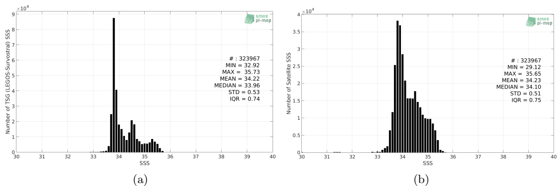
Figure 2: Histograms of SSS from TSG (LEGOS-Survostral) (a) and CCI L4 Merged-OI v2.31 - 30-day running (ESA) (b) considering all match-up pairs per bins of 0.1 over the Global Ocean Pi-MEP region and for the full satellite product period.
