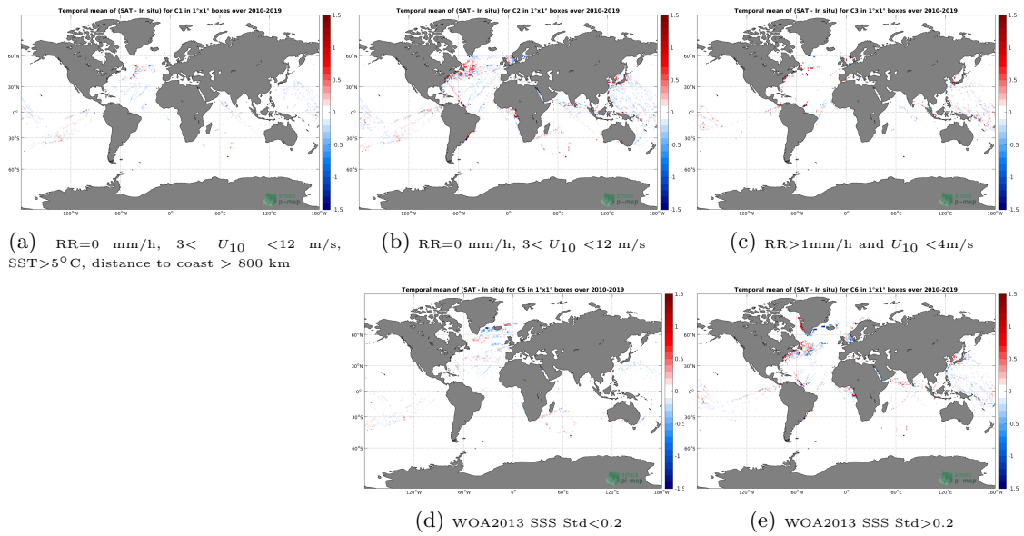
Figure 12: Temporal mean gridded over spatial boxes of size 1°x1° of \Delta SSS (CCI SSS L4 Merged-OI v2.31 - 30-day running (ESA) - TSG (LEGOS-DM)) for 5 different subdatasets corresponding to:RR=0 mm/h, 3 < U_{10} < 12 m/s, SST>5°C, distance to coast > 800 km (a), RR=0 mm/h, 3 < U_{10} < 12 m/s (b), RR>1mm/h and U_{10} < 4 m/s (c), WOA2013 SSS Std<0.2 (d), WOA2013 SSS Std>0.2 (e).
