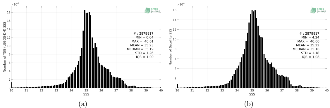
Figure 2: Histograms of SSS from TSG (LEGOS-DM) (a) and CCI SSS L4 Merged-OI v2.31 - 30-day running (ESA) (b) considering all match-up pairs per bins of 0.1 over the Global Ocean Pi-MEP region and for the full satellite product period.
