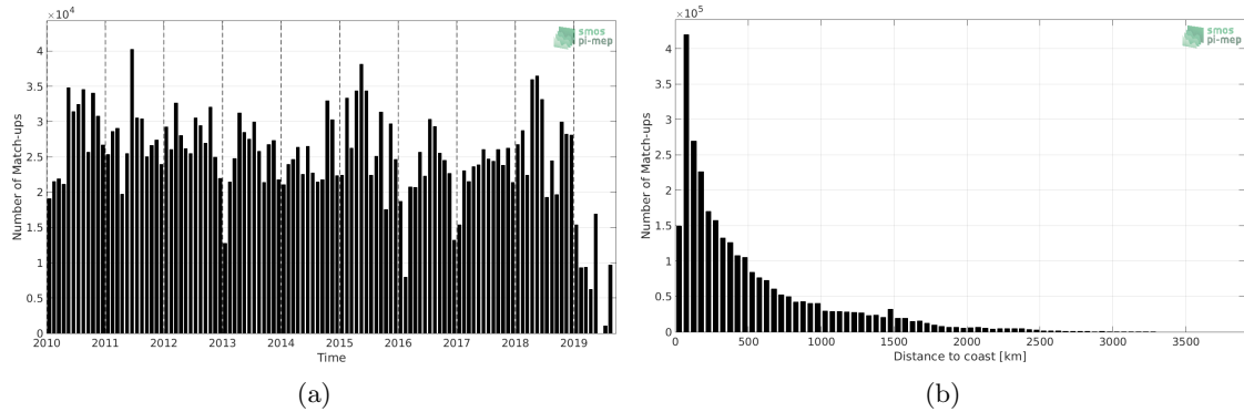
Figure 1: Number of match-ups between TSG (LEGOS-DM) and CCI SSS L4 Merged-OI v2.31 - 30-day running (ESA) SSS as a function of time (a) and as function of the distance to coast (b) over the Global Ocean Pi-MEP region and for the full satellite product period.
