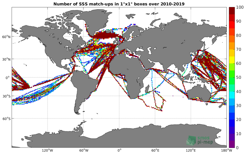
Figure 4: Number of SSS match-ups between TSG (LEGOS-DM) SSS and the CCI SSS L4 Merged-OI v2.31 - 30-day running (ESA) SSS product for the Global Ocean Pi-MEP region over 1°x1° boxes and for the full satellite product period.
