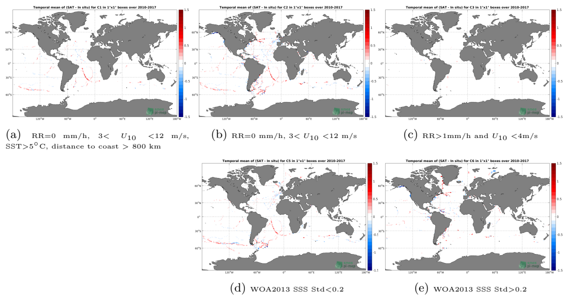
Figure 12: Temporal mean gridded over spatial boxes of size 1^\circ \times 1^\circ of \Delta SSS (CCI SSS L4 Merged-OI v2.31 - 30-day running (ESA) - TSG (GOSUD-Sailing-ship)) for 5 different subdatasets corresponding to: RR=0 mm/h, 3 < U_{10} < 12 m/s, SST > 5°C, distance to coast > 800 km (a), RR=0 mm/h, 3 < U_{10} < 12 m/s (b), RR > 1mm/h and U_{10} < 4 m/s (c), WOA2013 SSS Std < 0.2 (d), WOA2013 SSS Std > 0.2 (e).
