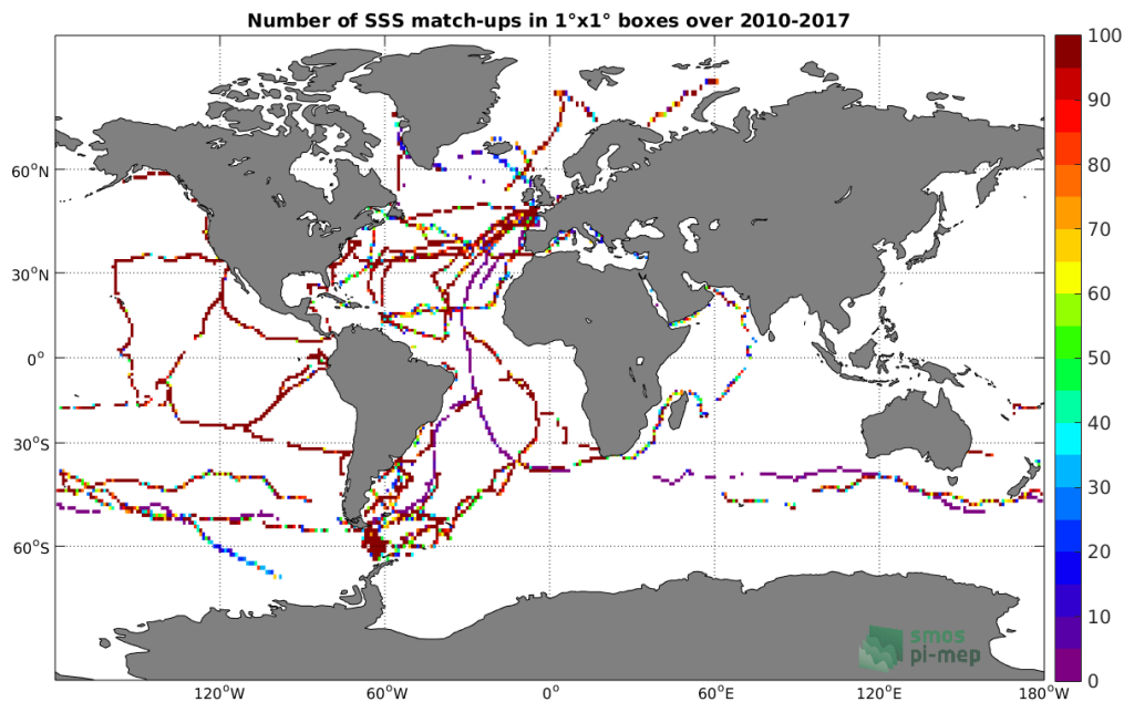
Figure 4: Number of SSS match-ups between TSG (GOSUD-Sailing-ship) SSS and the CCI SSS L4 Merged-OI v2.31 - 30-day running (ESA) SSS product for the Global Ocean Pi-MEP region over 1°x1° boxes and for the full satellite product period.
