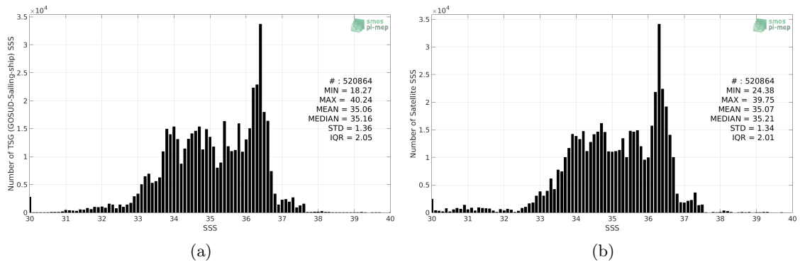
Figure 2: Histograms of SSS from TSG (GOSUD-Sailing-ship) (a) and CCI SSS L4 Merged-OI v2.31 - 30-day running (ESA) (b) considering all match-up pairs per bins of 0.1 over the Global Ocean Pi-MEP region and for the full satellite product period.
