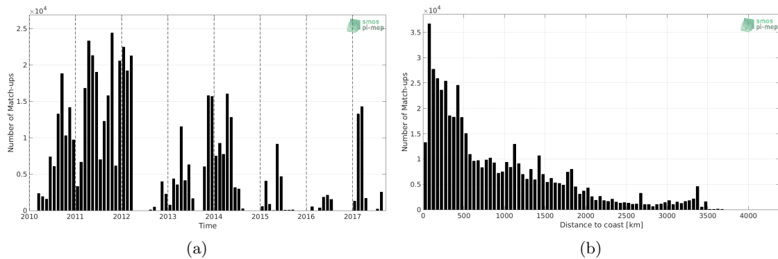
Figure 1: Number of match-ups between TSG (GOSUD-Sailing-ship) and CCI L4 Merged-OI v2.31 - 30-day running (ESA) SSS as a function of time (a) and as function of the distance to coast (b) over the Global Ocean Pi-MEP region and for the full satellite product period.
