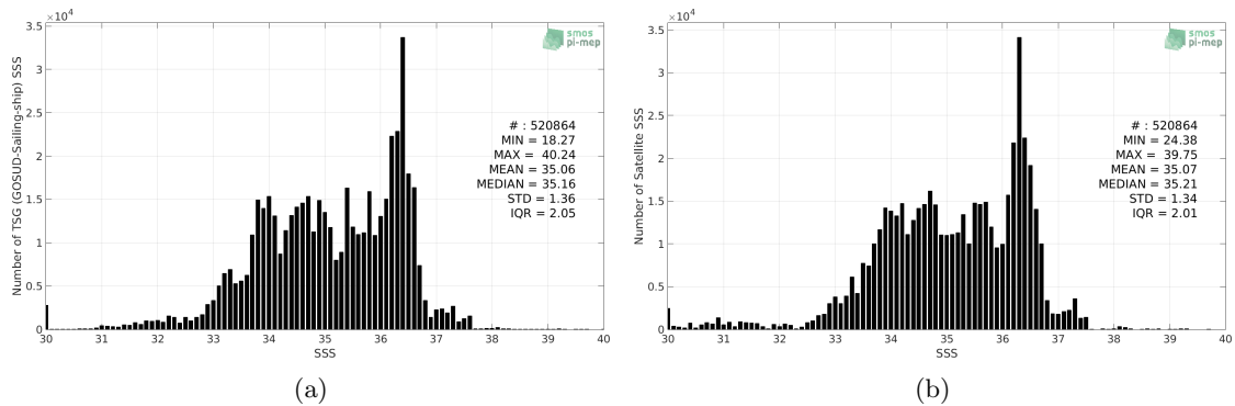
Figure 2: Histograms of SSS from TSG (GOSUD-Sailing-ship) (a) and CCI L4 Merged-OI v2.31 - 30-day running (ESA) (b) considering all match-up pairs per bins of 0.1 over the Global Ocean Pi-MEP region and for the full satellite product period.
