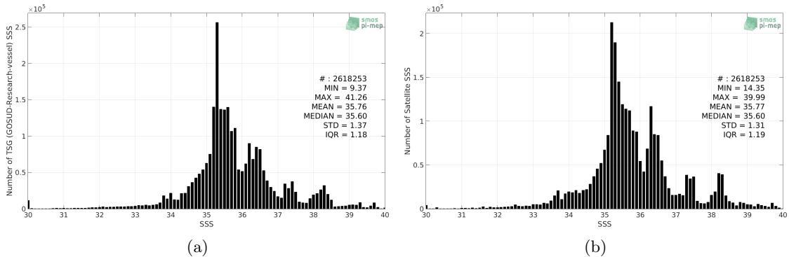
Figure 2: Histograms of SSS from TSG (GOSUD-Research-vessel) (a) and CCI SSS L4 Merged-OI v2.31 - 30-day running (ESA) (b) considering all match-up pairs per bins of 0.1 over the Global Ocean Pi-MEP region and for the full satellite product period.
