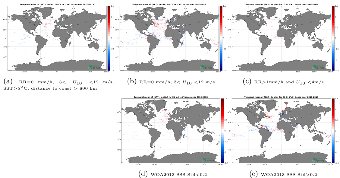
Figure 12: Temporal mean gridded over spatial boxes of size 1^\circ \times 1^\circ of \Delta\text{SSS} (CCI SSS L4 Merged-OI v2.31 - 30-day running (ESA) - TSG (GOSUD-Research-vessel)) for 5 different subdatasets corresponding to:RR=0 mm/h, 3 < U_{10} < 12 m/s, SST>5°C, distance to coast > 800 km (a), RR=0 mm/h, 3 < U_{10} < 12 m/s (b), RR>1mm/h and U_{10} < 4 m/s (c), WOA2013 SSS Std<0.2 (d), WOA2013 SSS Std>0.2 (e).
