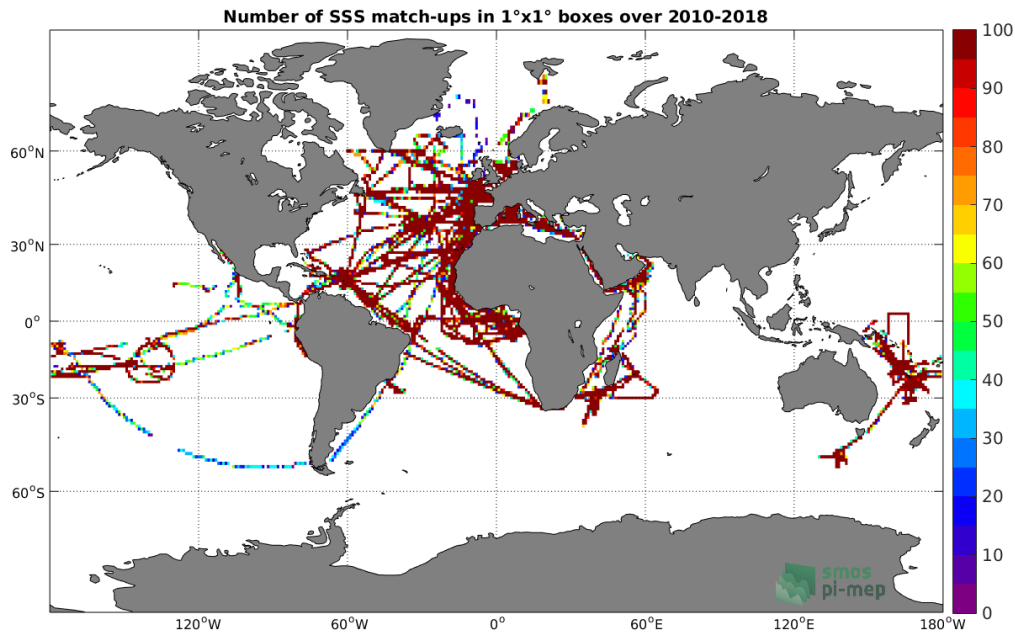
Figure 4: Number of SSS match-ups between TSG (GOSUD-Research-vessel) SSS and the CCI SSS L4 Merged-OI v2.31 - 30-day running (ESA) SSS product for the Global Ocean Pi-MEP region over 1°x1° boxes and for the full satellite product period.
