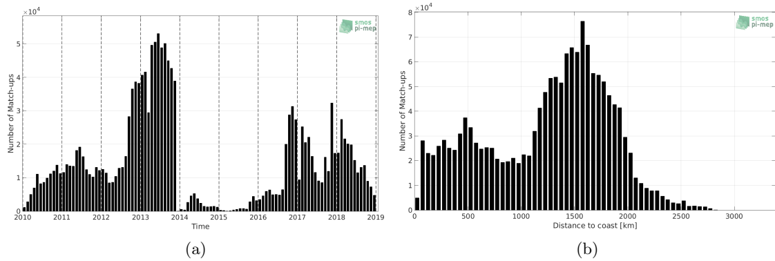
Figure 1: Number of match-ups between Surface drifters and CCI SSS L4 Merged-OI v2.31 - 30-day running (ESA) SSS as a function of time (a) and as function of the distance to coast (b) over the Global Ocean Pi-MEP region and for the full satellite product period.
