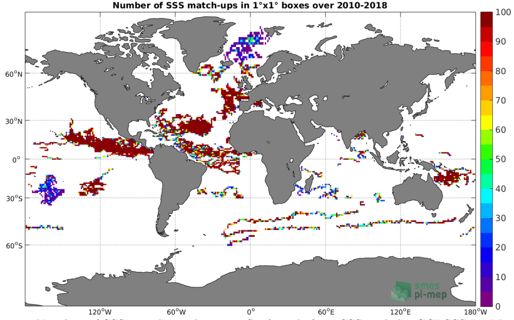
Figure 3: Number of SSS match-ups between Surface drifters SSS and the CCI SSS L4 Merged-OI v2.31 - 30-day running (ESA) SSS product for the Global Ocean Pi-MEP region over 1^\circ \times 1^\circ boxes and for the full satellite product period.
