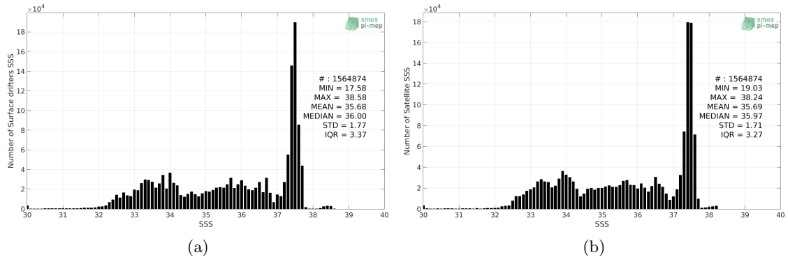
Figure 2: Histograms of SSS from Surface drifters (a) and CCI SSS L4 Merged-OI v2.31 - 30-day running (ESA) (b) considering all match-up pairs per bins of 0.1 over the Global Ocean Pi-MEP region and for the full satellite product period.
