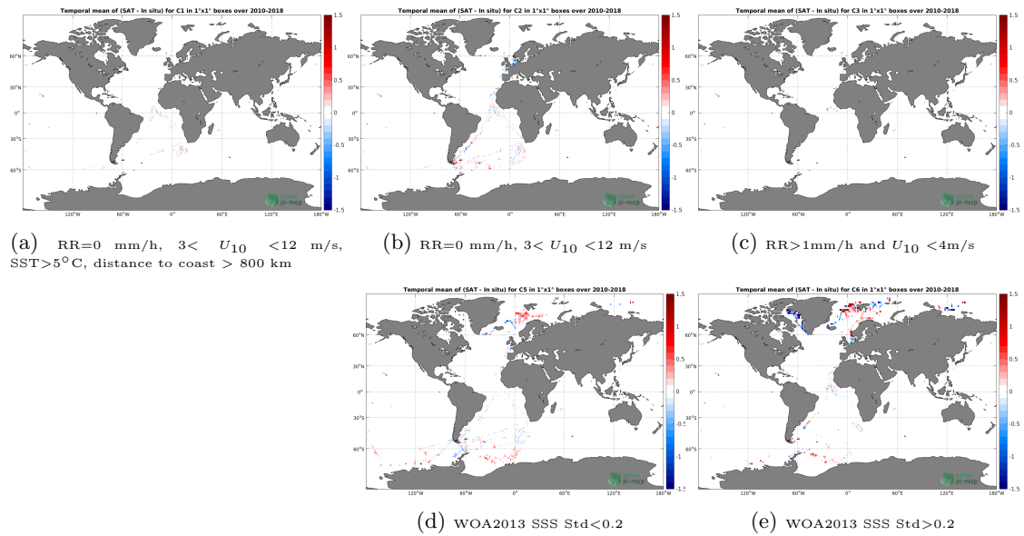
Figure 12: Temporal mean gridded over spatial boxes of size 1^\circ \times 1^\circ of \Delta SSS (CCI L4 Merged-OI v1.8 - 30-day running (ESA) - TSG-POLARSTERN) for 5 different subdatasets corresponding to: RR=0 mm/h, 3 < U_{10} < 12 m/s, SST > 5^\circ\text{C} , distance to coast > 800 km (a), RR=0 mm/h, 3 < U_{10} < 12 m/s (b), RR > 1 mm/h and U_{10} < 4 m/s (c), WOA2013 SSS Std < 0.2 (d), WOA2013 SSS Std > 0.2 (e).
