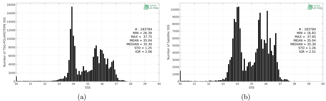
Figure 2: Histograms of SSS from TSG-POLARSTERN (a) and CCI L4 Merged-OI v1.8 - 30-day running (ESA) (b) considering all match-up pairs per bins of 0.1 over the Global Ocean Pi-MEP region and for the full satellite product period.
