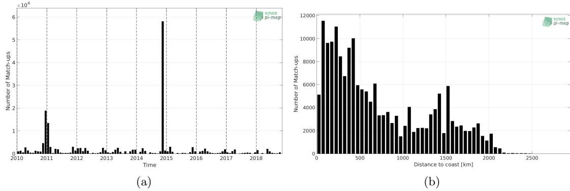
Figure 1: Number of match-ups between TSG-POLARSTERN and CCI L4 Merged-OI v1.8 - 30-day running (ESA) SSS as a function of time (a) and as function of the distance to coast (b) over the Global Ocean Pi-MEP region and for the full satellite product period.
