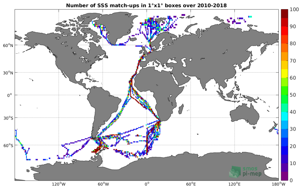
Figure 4: Number of SSS match-ups between TSG-POLARSTERN SSS and the CCI L4 Merged-OI v1.8 - 30-day running (ESA) SSS product for the Global Ocean Pi-MEP region over 1^\circ \times 1^\circ boxes and for the full satellite product period.
