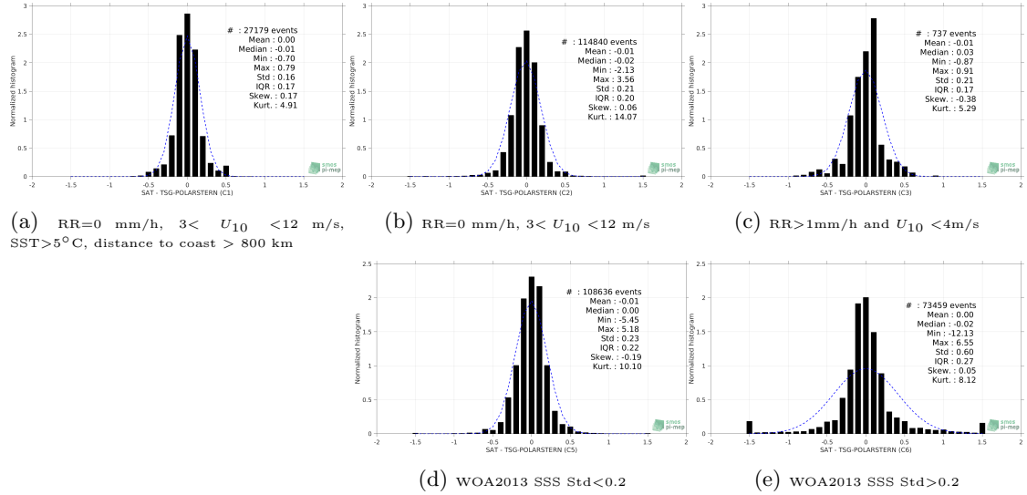
Figure 13: Normalized histogram of \Delta SSS (CCI L4 Merged-OI v1.8 - 30-day running (ESA) - TSG-POLARSTERN) for 5 different subdatasets corresponding to: RR=0 mm/h, 3 < U_{10} < 12 m/s, SST > 5°C, distance to coast > 800 km (a), RR=0 mm/h, 3 < U_{10} < 12 m/s (b), RR > 1mm/h and U_{10} < 4 m/s (c), WOA2013 SSS Std < 0.2 (d), WOA2013 SSS Std > 0.2 (e).
