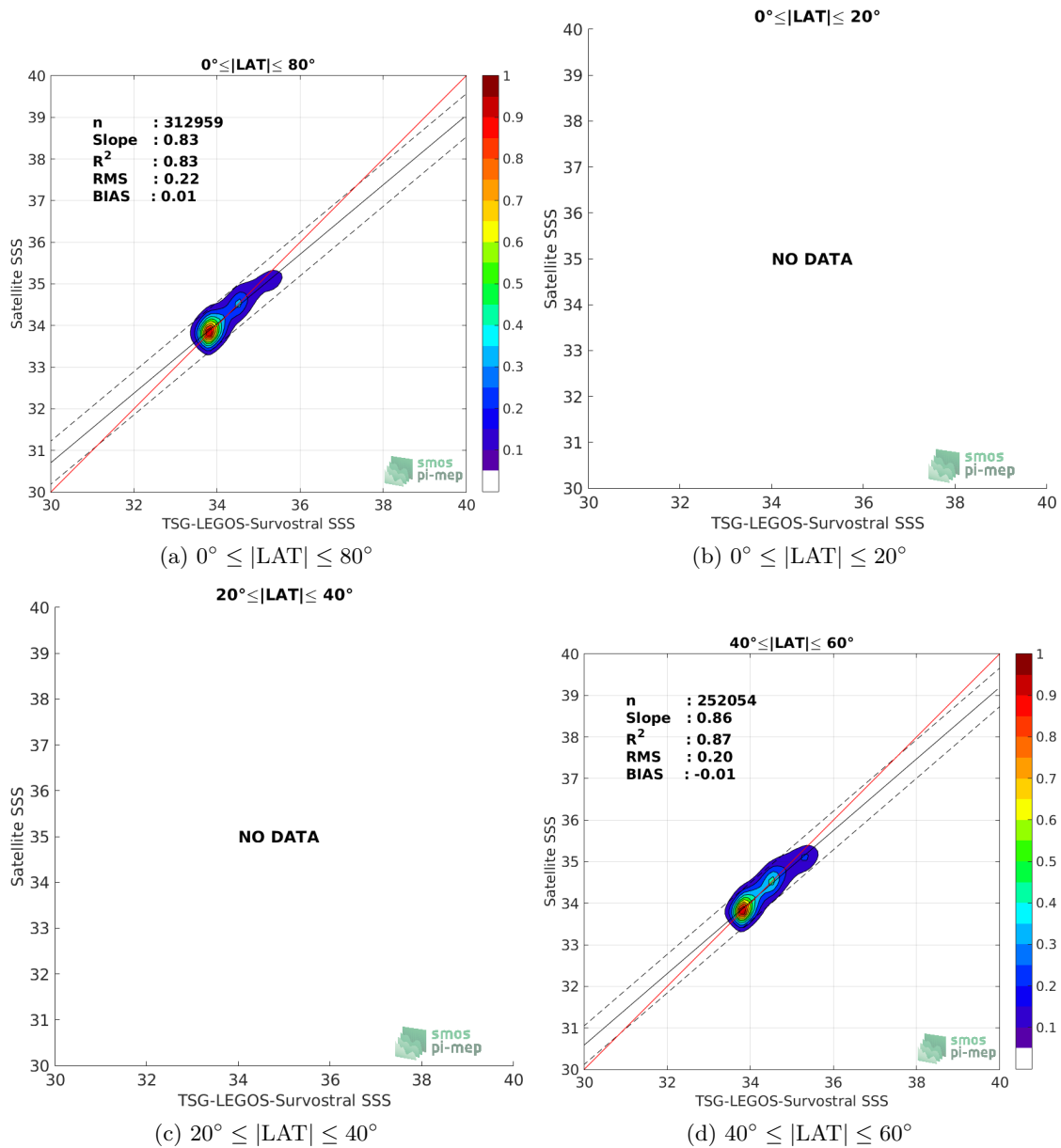
Figure 9: Contour maps of the concentration of CCI L4 Merged-OI v1.8 - 30-day running (ESA) SSS (y-axis) versus TSG-LEGOS-Survostral SSS (x-axis) at match-up pairs for different latitude bands. For each plot, the red line shows x=y . The black thin and dashed lines indicate a linear fit through the data cloud and the \pm 95\% confidence levels, respectively. The number match-up pairs n , the slope and R^2 coefficient of the linear fit, the root mean square (RMS) and the mean bias between satellite and in situ data are indicated for each latitude band in each plots.
