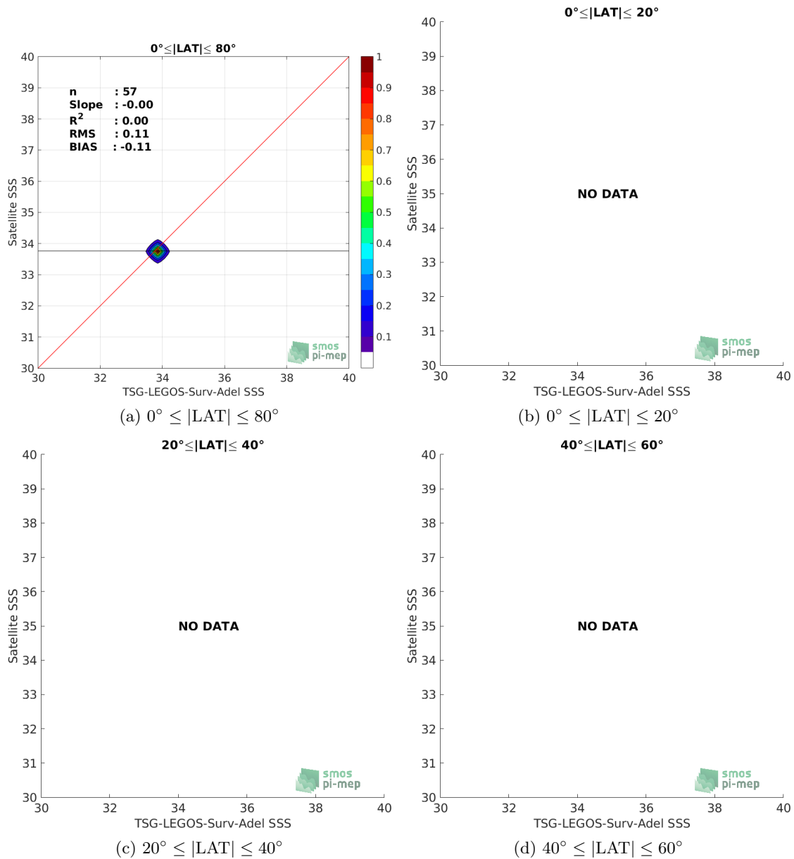
Figure 9: Contour maps of the concentration of CCI L4 Merged-OI v1.8 - 30-day running (ESA) SSS (y-axis) versus TSG-LEGOS-Surv-Adel SSS (x-axis) at match-up pairs for different latitude bands. For each plot, the red line shows x=y . The black thin and dashed lines indicate a linear fit through the data cloud and the \pm 95\% confidence levels, respectively. The number match-up pairs n , the slope and R^2 coefficient of the linear fit, the root mean square (RMS) and the mean bias between satellite and in situ data are indicated for each latitude band in each plots.
