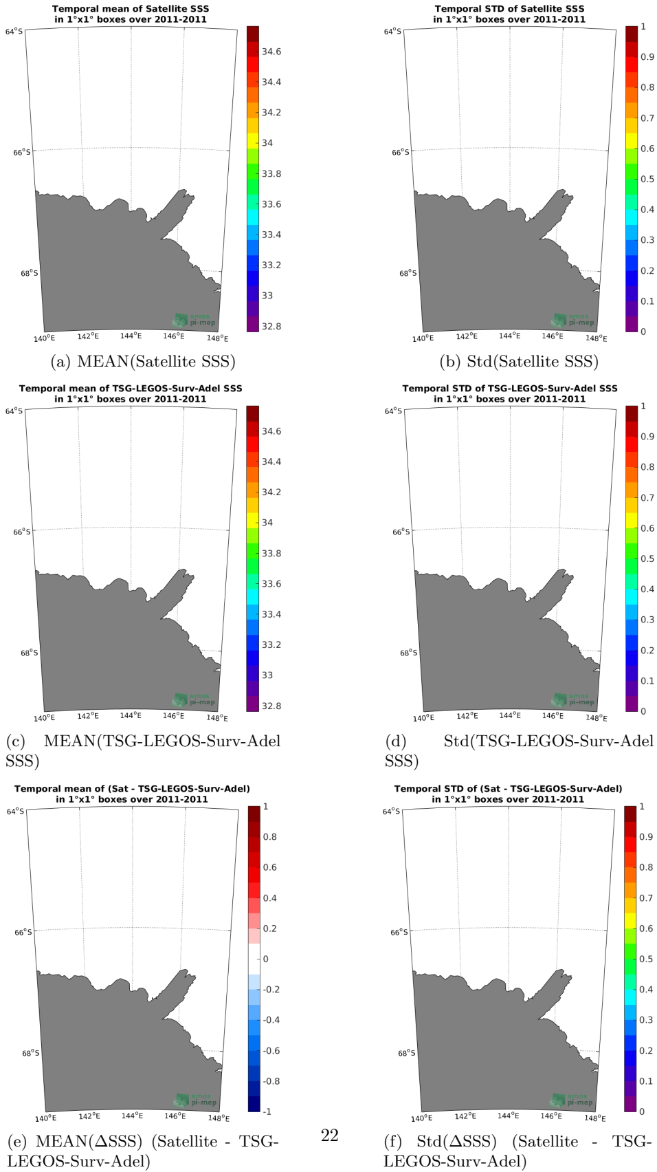
Figure 6: Temporal mean (left) and Std (right) of SSS from CCI L4 Merged-OI v1.8 - 30-day running (ESA) (top), TSG-LEGOS-Surv-Adel (middle), and of \Delta SSS (Satellite - TSG-LEGOS-Surv-Adel). Only match-up pairs are used to generate these maps.
