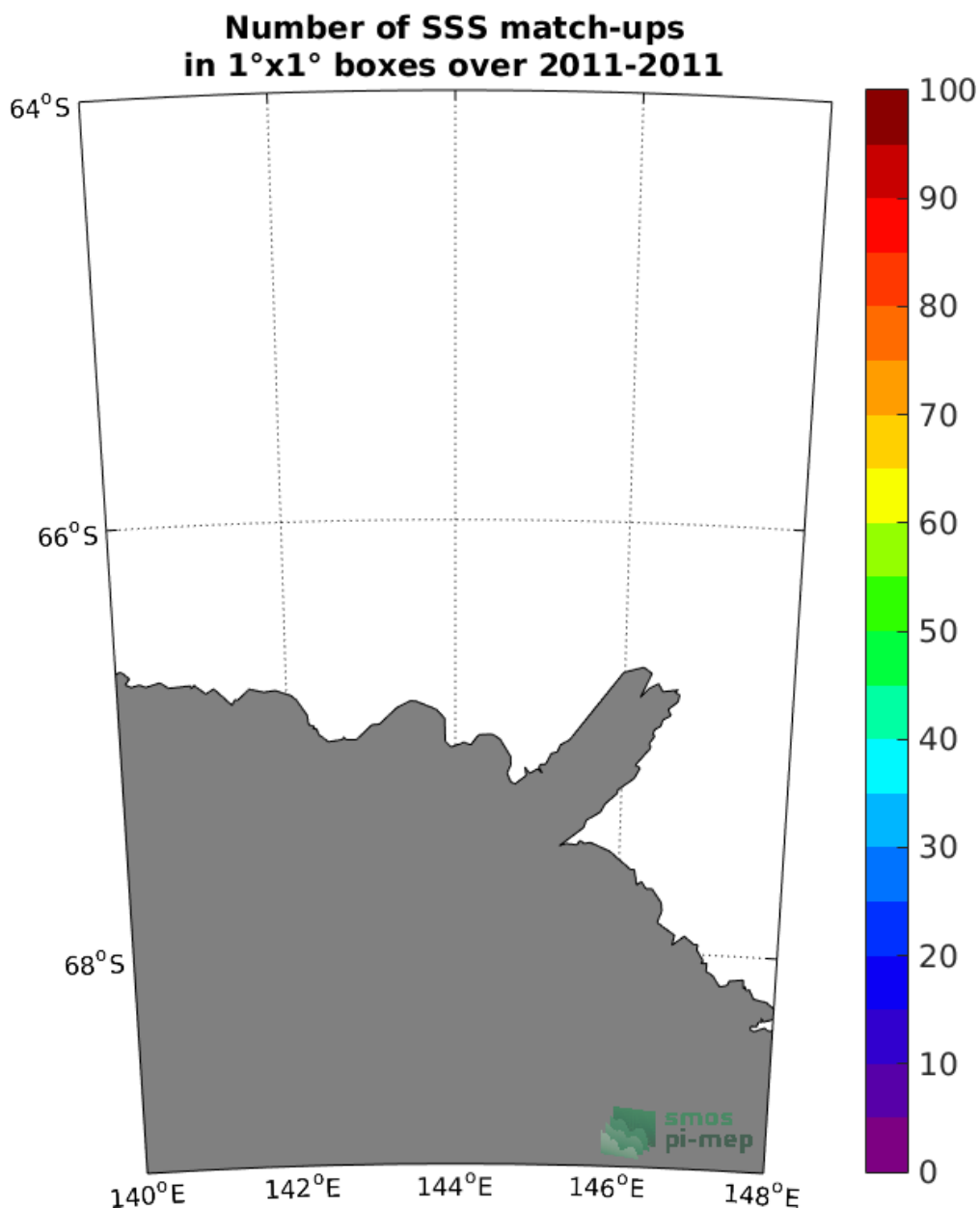
Figure 4: Number of SSS match-ups between TSG-LEGOS-Surv-Adel SSS and the CCI L4 Merged-OI v1.8 - 30-day running (ESA) SSS product for the Global Ocean Pi-MEP region over 1°x1° boxes and for the full satellite product period.
