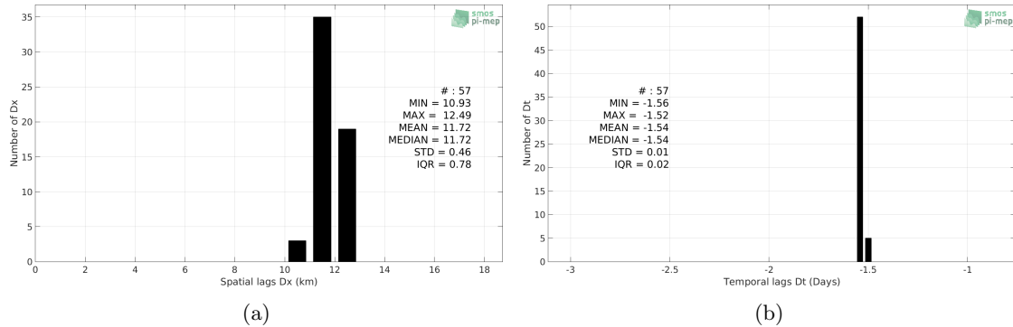
Figure 5: Histograms of the spatial (a) and temporal (b) lags between the time of the TSG-LEGOS-Surv-Adel measurements and the date of the corresponding CCI L4 Merged-OI v1.8 - 30-day running (ESA) SSS product.
