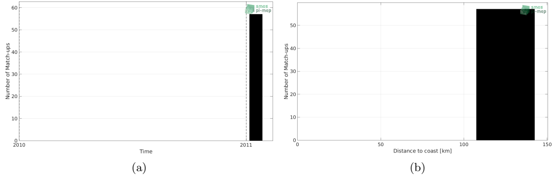
Figure 1: Number of match-ups between TSG-LEGOS-Surv-Adel and CCI L4 Merged-OI v1.8 - 30-day running (ESA) SSS as a function of time (a) and as function of the distance to coast (b) over the Global Ocean Pi-MEP region and for the full satellite product period.
