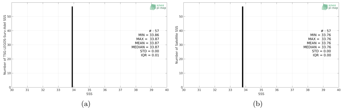
Figure 2: Histograms of SSS from TSG-LEGOS-Surv-Adel (a) and CCI L4 Merged-OI v1.8 - 30-day running (ESA) (b) considering all match-up pairs per bins of 0.1 over the Global Ocean Pi-MEP region and for the full satellite product period.
