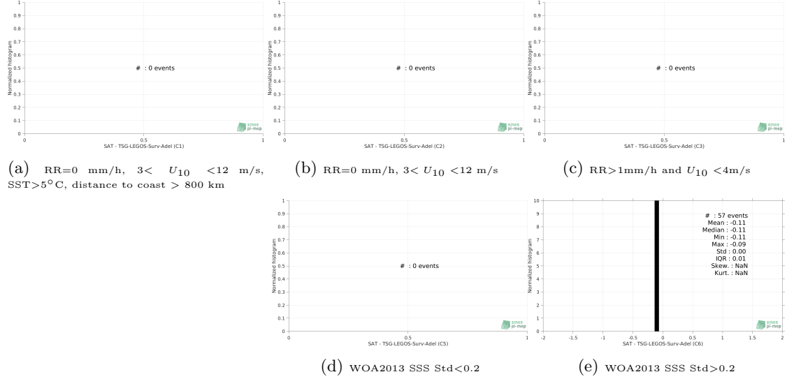
Figure 13: Normalized histogram of \Delta\text{SSS} (CCI L4 Merged-OI v1.8 - 30-day running (ESA) - TSG-LEGOS-Surv-Adel) for 5 different subdatasets corresponding to: RR=0 mm/h, 3 < U_{10} < 12 m/s, SST > 5^{\circ}\text{C} , distance to coast > 800 km (a), RR=0 mm/h, 3 < U_{10} < 12 m/s (b), RR > 1\text{mm/h} and U_{10} < 4\text{m/s} (c), WOA2013 SSS Std < 0.2 (d), WOA2013 SSS Std > 0.2 (e).
