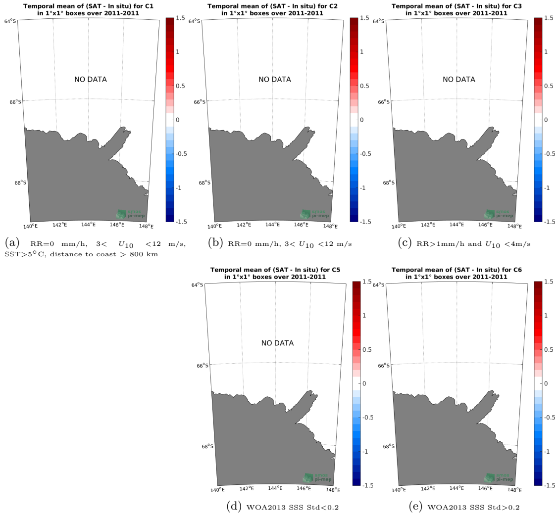
Figure 12: Temporal mean gridded over spatial boxes of size 1°x1° of \Delta SSS (CCI L4 Merged-OI v1.8 - 30-day running (ESA) - TSG-LEGOS-Surv-Adel) for 5 different subdatasets corresponding to: RR=0 mm/h, 3 < U_{10} < 12 m/s, SST>5°C, distance to coast > 800 km (a), RR=0 mm/h, 3 < U_{10} < 12 m/s (b), RR>1mm/h and U_{10} < 4 m/s (c), WOA2013 SSS Std<0.2 (d), WOA2013 SSS Std>0.2 (e).
