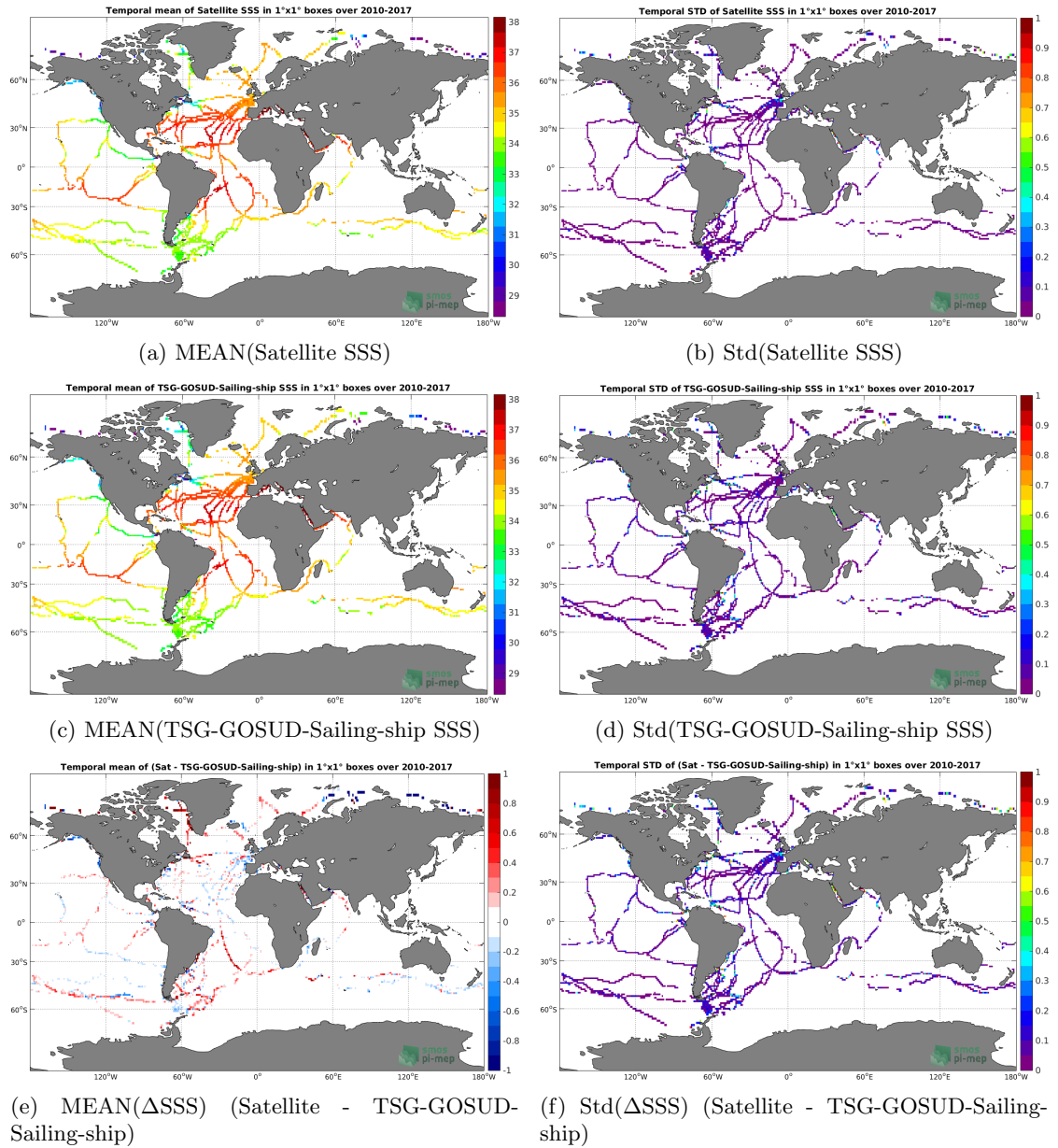
Figure 6: Temporal mean (left) and Std (right) of SSS from CCI L4 Merged-OI v1.8 - 30-day running (ESA) (top), TSG-GOSUD-Sailing-ship (middle), and of \Delta SSS (Satellite - TSG-GOSUD-Sailing-ship). Only match-up pairs are used to generate these maps.
