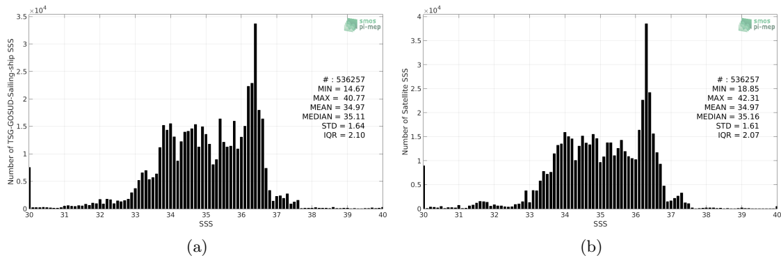
Figure 2: Histograms of SSS from TSG-GOSUD-Sailing-ship (a) and CCI L4 Merged-OI v1.8 - 30-day running (ESA) (b) considering all match-up pairs per bins of 0.1 over the Global Ocean Pi-MEP region and for the full satellite product period.
