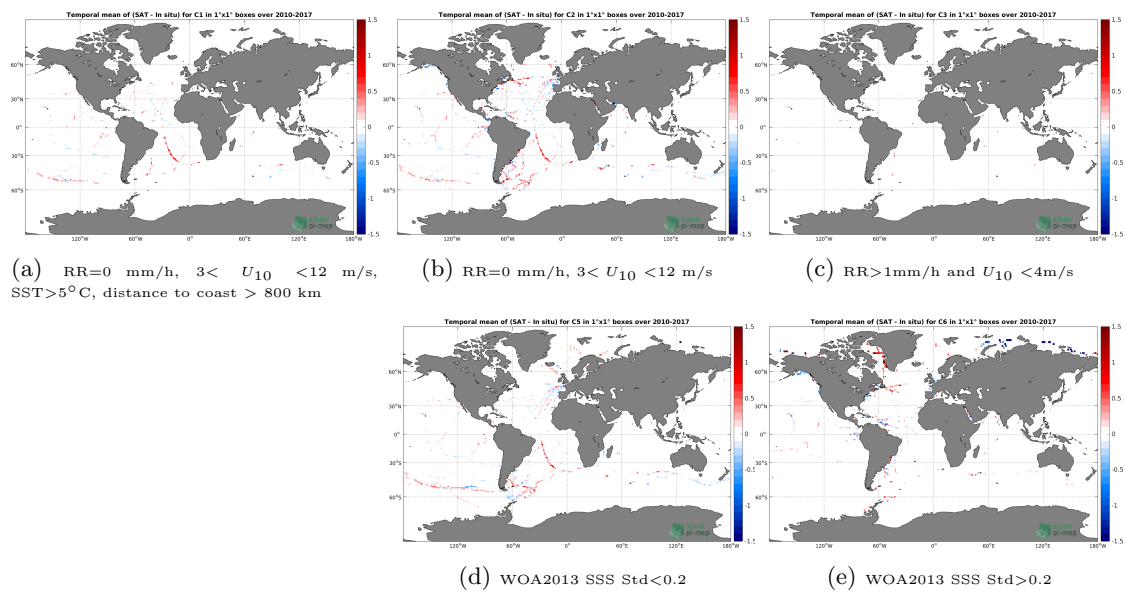
Figure 12: Temporal mean gridded over spatial boxes of size 1^\circ \times 1^\circ of \Delta SSS (CCI L4 Merged-OI v1.8 - 30-day running (ESA) - TSG-GOSUD-Sailing-ship) for 5 different subdatasets corresponding to:RR=0 mm/h, 3 < U_{10} < 12 m/s, SST >5^\circ C, distance to coast > 800 km (a), RR=0 mm/h, 3 < U_{10} < 12 m/s (b), RR >1 mm/h and U_{10} < 4 m/s (c), WOA2013 SSS Std <0.2 (d), WOA2013 SSS Std >0.2 (e).
