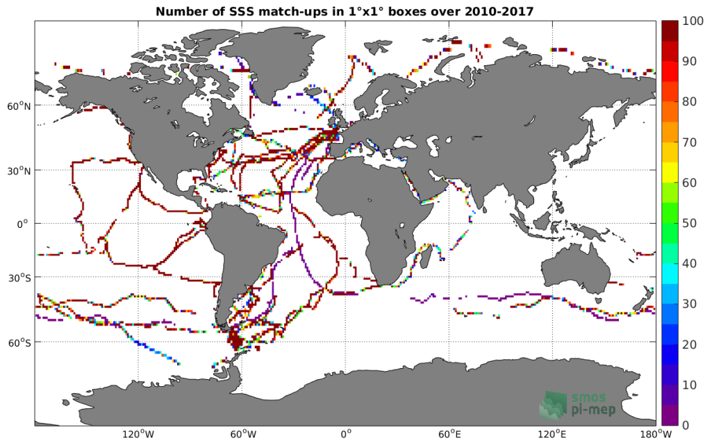
Figure 4: Number of SSS match-ups between TSG-GOSUD-Sailing-ship SSS and the CCI L4 Merged-OI v1.8 - 30-day running (ESA) SSS product for the Global Ocean Pi-MEP region over 1^\circ \times 1^\circ boxes and for the full satellite product period.
