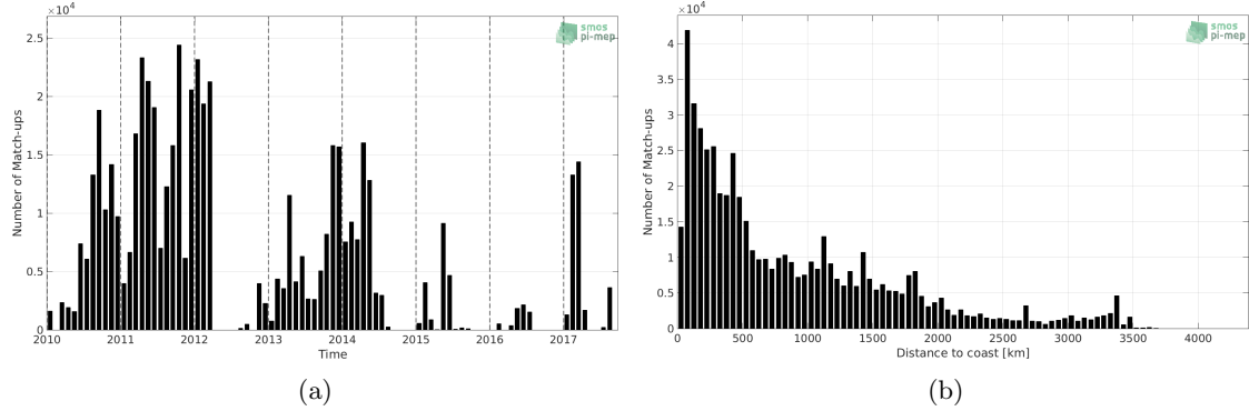
Figure 1: Number of match-ups between TSG-GOSUD-Sailing-ship and CCI L4 Merged-OI v1.8 - 30-day running (ESA) SSS as a function of time (a) and as function of the distance to coast (b) over the Global Ocean Pi-MEP region and for the full satellite product period.
