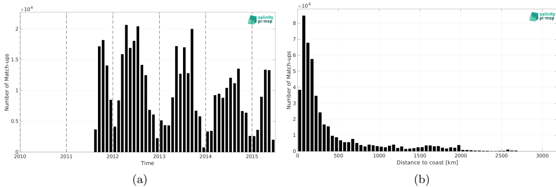
Figure 2: Number of match-ups between TSG (SAMOS) and Aquarius SSS L4 OI v5 - Weekly (IPRC) SSS as a function of time (a) and as function of the distance to coast (b) over the Global Ocean Pi-MEP region and for the full satellite product period.
