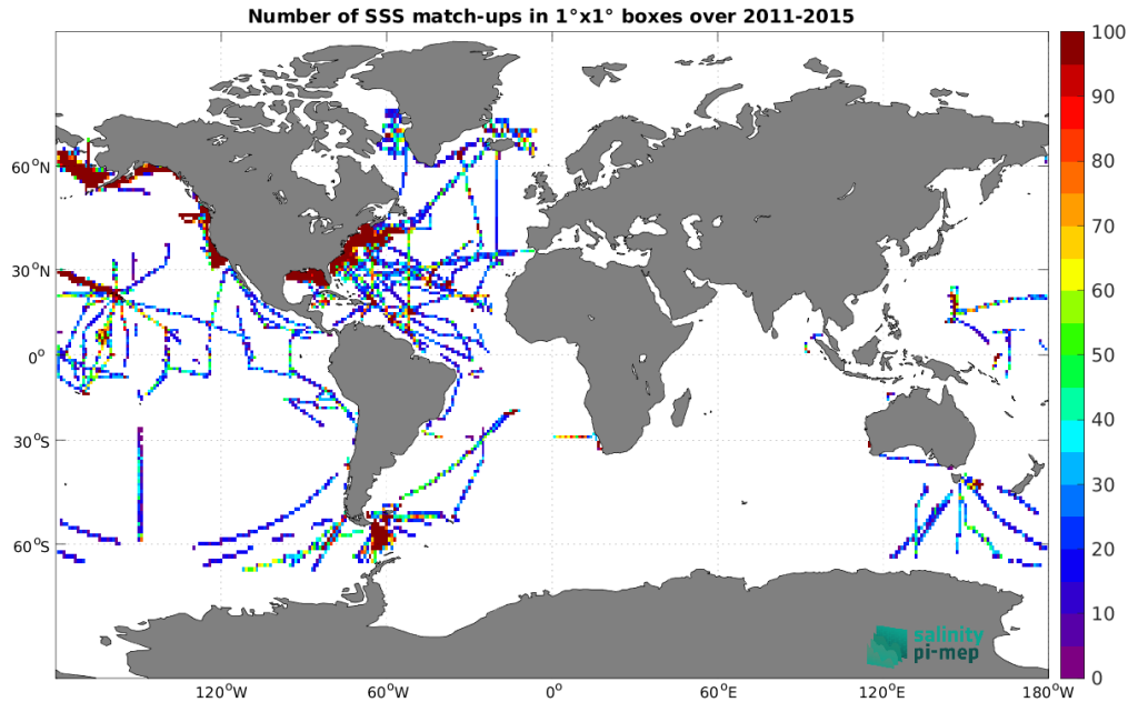
Figure 5: Number of SSS match-ups between TSG (SAMOS) SSS and the Aquarius SSS L4 OI v5 - Weekly (IPRC) SSS product for the Global Ocean Pi-MEP region over 1^\circ \times 1^\circ boxes and for the full satellite product period.
