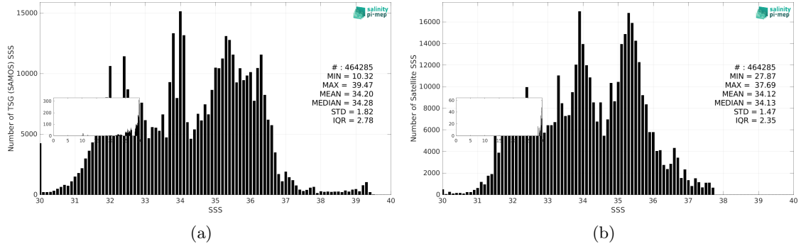
Figure 3: Histograms of SSS from TSG (SAMOS) (a) and Aquarius SSS L4 OI v5 - Weekly (IPRC) (b) considering all match-up pairs per bins of 0.1 over the Global Ocean Pi-MEP region and for the full satellite product period.
