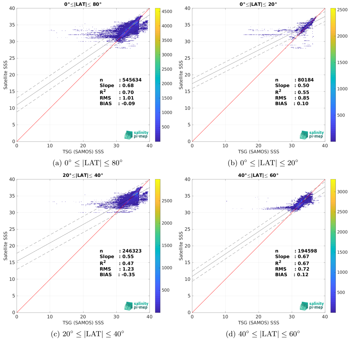
Figure 9: Contour maps of the concentration of Aquarius SSS L4 OI v5 - Weekly (IPRC) SSS (y-axis) versus TSG (SAMOS) SSS (x-axis) at match-up pairs for different latitude bands. For each plot, the red line shows x=y . The black thin and dashed lines indicate a linear fit through the data cloud and the \pm 95\% confidence levels, respectively. The number match-up pairs n , the slope and R^2 coefficient of the linear fit, the root mean square (RMS) and the mean bias between satellite and in situ data are indicated for each latitude band in each plot.
