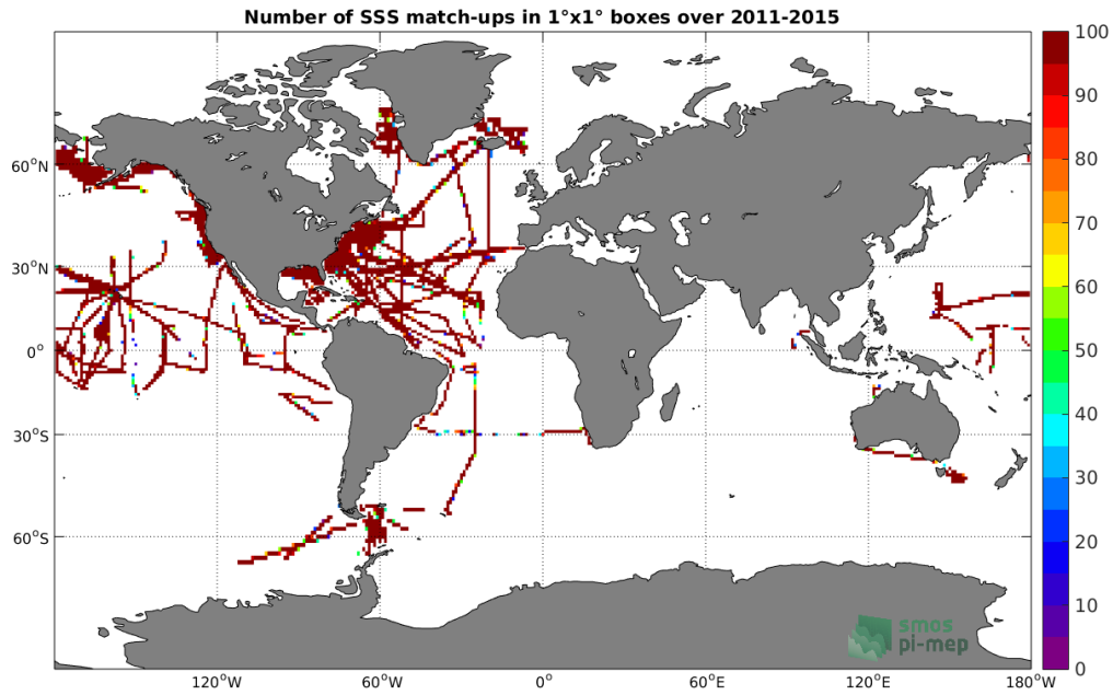
Figure 4: Number of SSS match-ups between TSG-SAMOS SSS and the Aquarius-L4-IPRC-V5-WEEKLY SSS product for the Global Ocean Pi-MEP region over 1°x1° boxes and for the full satellite product period.
