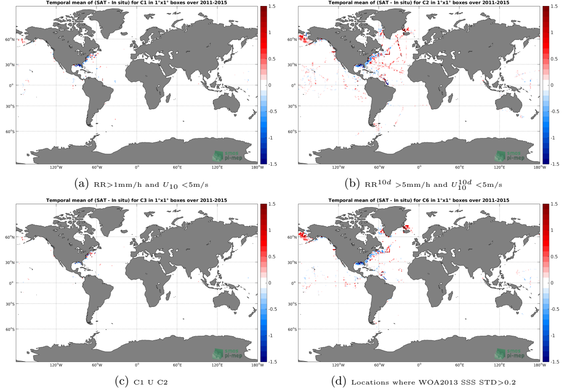
Figure 12: Temporal mean gridded over spatial boxes of size 1^\circ \times 1^\circ of \Delta SSS (Aquarius-L4-IPRC-V5-WEEKLY - TSG-SAMOS) for 4 different subdatasets corresponding to: RR > 1\text{mm/h} and U_{10} < 5\text{m/s} (a), RR^{10d} > 5\text{mm/h} and U_{10}^{10d} < 5\text{m/s} (b), C1 U C2 (c), Locations where WOA2013 SSS STD > 0.2 (d).
