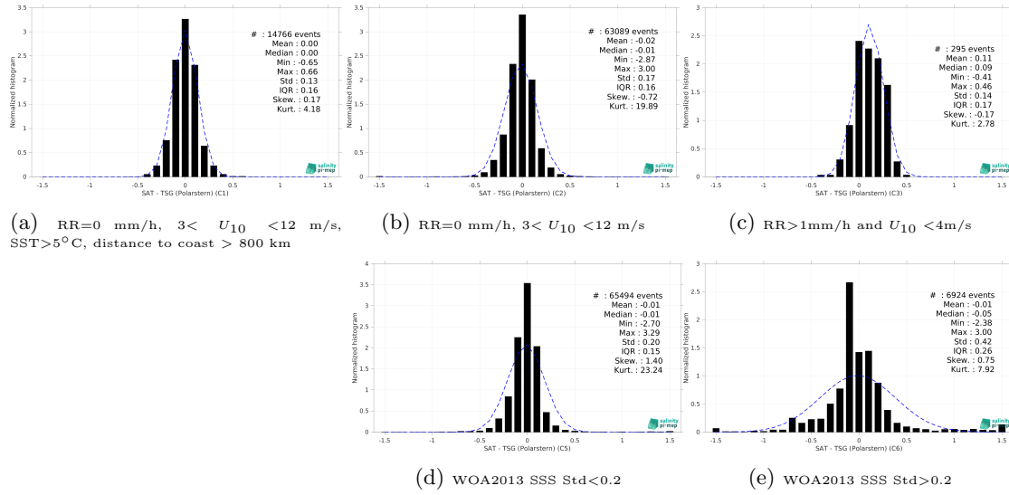
Figure 15: Normalized histogram of \Delta SSS (Aquarius SSS L4 OI v5 - Weekly (IPRC) - TSG (Polarstern)) for 5 different subdatasets corresponding to: RR=0 mm/h, 3 < U_{10} < 12 m/s, SST > 5°C, distance to coast > 800 km (a), RR=0 mm/h, 3 < U_{10} < 12 m/s (b), RR > 1mm/h and U_{10} < 4 m/s (c), WOA2013 SSS Std < 0.2 (d), WOA2013 SSS Std > 0.2 (e).
