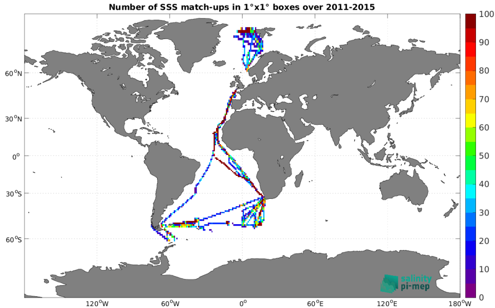
Figure 4: Number of SSS match-ups between TSG (Polarstern) SSS and the Aquarius SSS L4 OI v5 - Weekly (IPRC) SSS product for the Global Ocean Pi-MEP region over 1°×1° boxes and for the full satellite product period.
