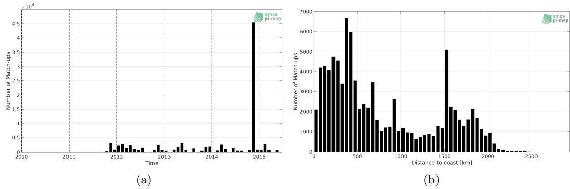
Figure 1: Number of match-ups between TSG (Polarstern) and Aquarius SSS L4 OI v5 - Weekly (IPRC) SSS as a function of time (a) and as function of the distance to coast (b) over the Global Ocean Pi-MEP region and for the full satellite product period.
