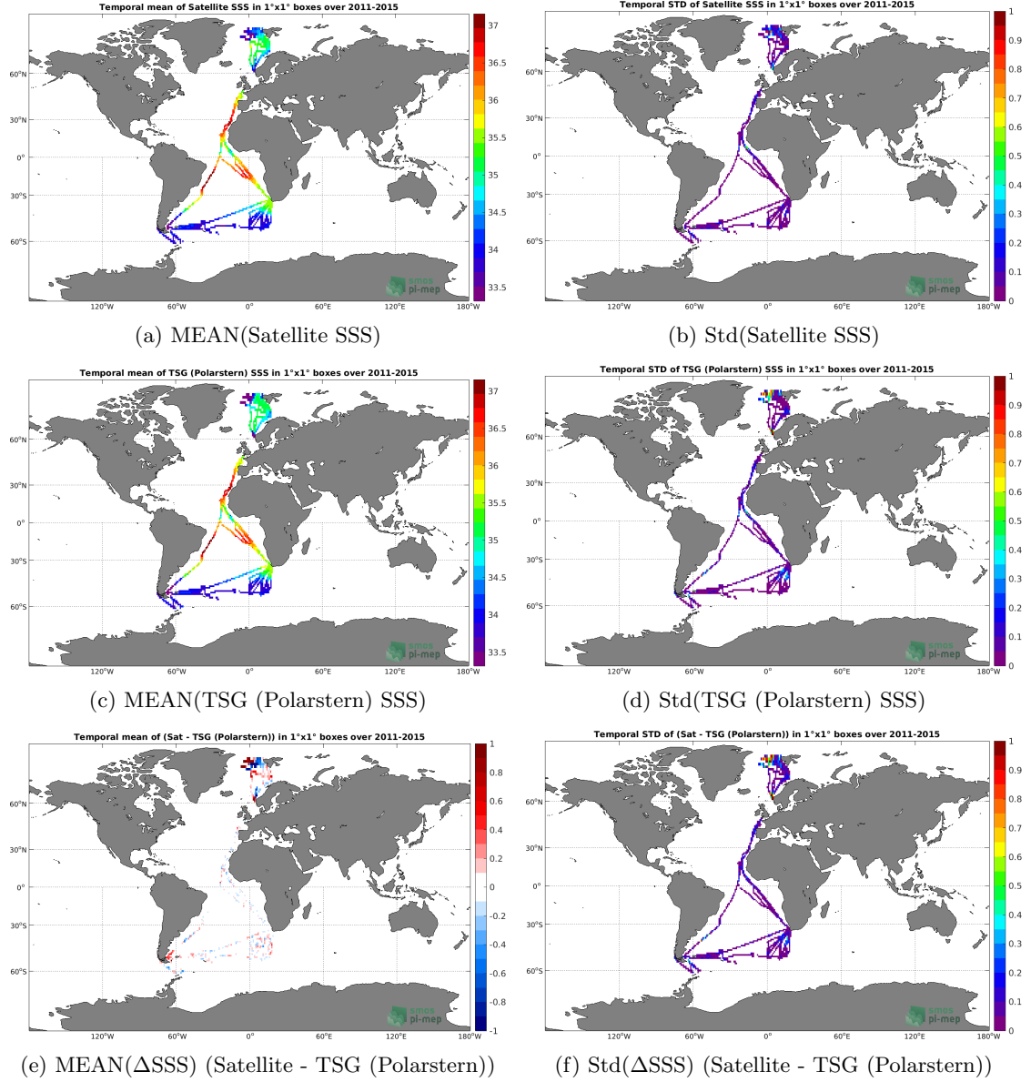
Figure 6: Temporal mean (left) and Std (right) of SSS from Aquarius SSS L4 OI v5 - Weekly (IPRC) (top), TSG (Polarstern) (middle), and of \Delta SSS (Satellite - TSG (Polarstern)). Only match-up pairs are used to generate these maps.
