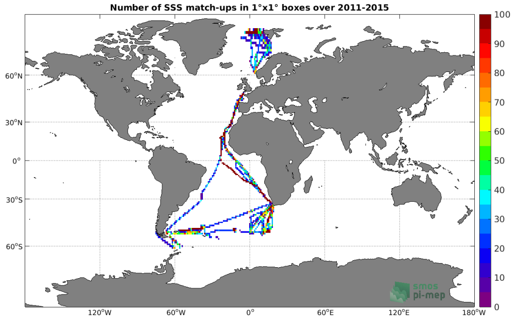
Figure 4: Number of SSS match-ups between TSG (Polarstern) SSS and the Aquarius SSS L4 OI v5 - Weekly (IPRC) SSS product for the Global Ocean Pi-MEP region over 1^\circ \times 1^\circ boxes and for the full satellite product period.
