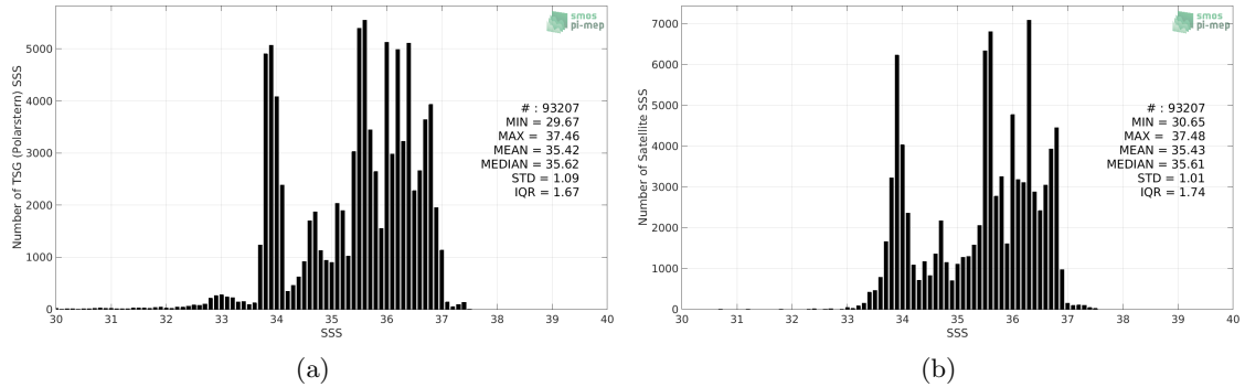
Figure 2: Histograms of SSS from TSG (Polarstern) (a) and Aquarius SSS L4 OI v5 - Weekly (IPRC) (b) considering all match-up pairs per bins of 0.1 over the Global Ocean Pi-MEP region and for the full satellite product period.
