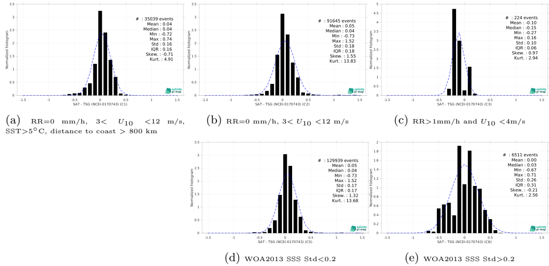
Figure 15: Normalized histogram of \Delta\text{SSS} (Aquarius SSS L4 OI v5 - Weekly (IPRC) - TSG (NCEI-0170743)) for 5 different subdatasets corresponding to: RR=0 mm/h, 3 < U_{10} < 12 m/s, SST>5°C, distance to coast > 800 km (a), RR=0 mm/h, 3 < U_{10} < 12 m/s (b), RR>1mm/h and U_{10} < 4 m/s (c), WOA2013 SSS Std<0.2 (d), WOA2013 SSS Std>0.2 (e).
