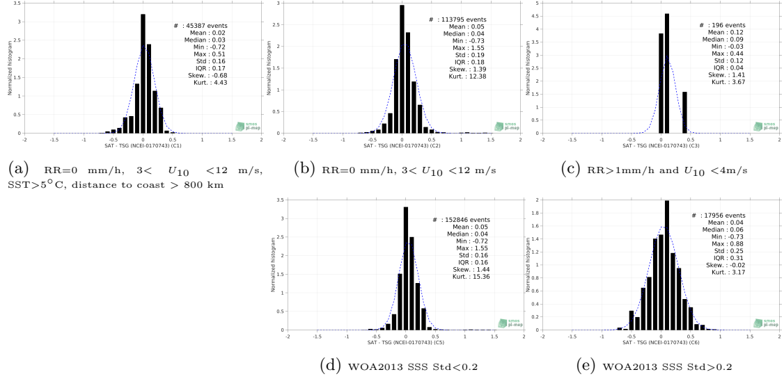
Figure 13: Normalized histogram of \Delta SSS (Aquarius SSS L4 OI v5 - Weekly (IPRC) - TSG (NCEI-0170743)) for 5 different subdatasets corresponding to: RR=0 mm/h, 3 < U_{10} < 12 m/s, SST>5°C, distance to coast > 800 km (a), RR=0 mm/h, 3 < U_{10} < 12 m/s (b), RR>1mm/h and U_{10} < 4 m/s (c), WOA2013 SSS Std<0.2 (d), WOA2013 SSS Std>0.2 (e).
