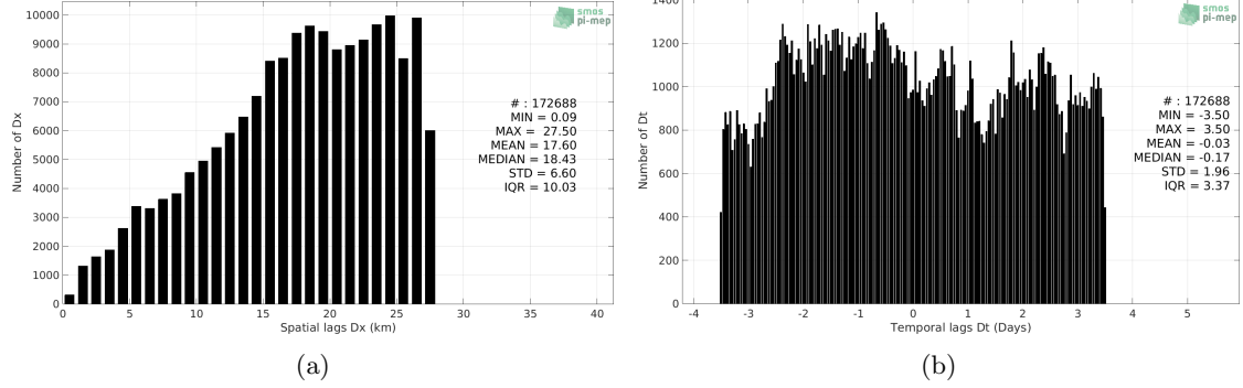
Figure 5: Histograms of the spatial (a) and temporal (b) lags between the time of the TSG (NCEI-0170743) measurements and the date of the corresponding Aquarius SSS L4 OI v5 - Weekly (IPRC) SSS product.
