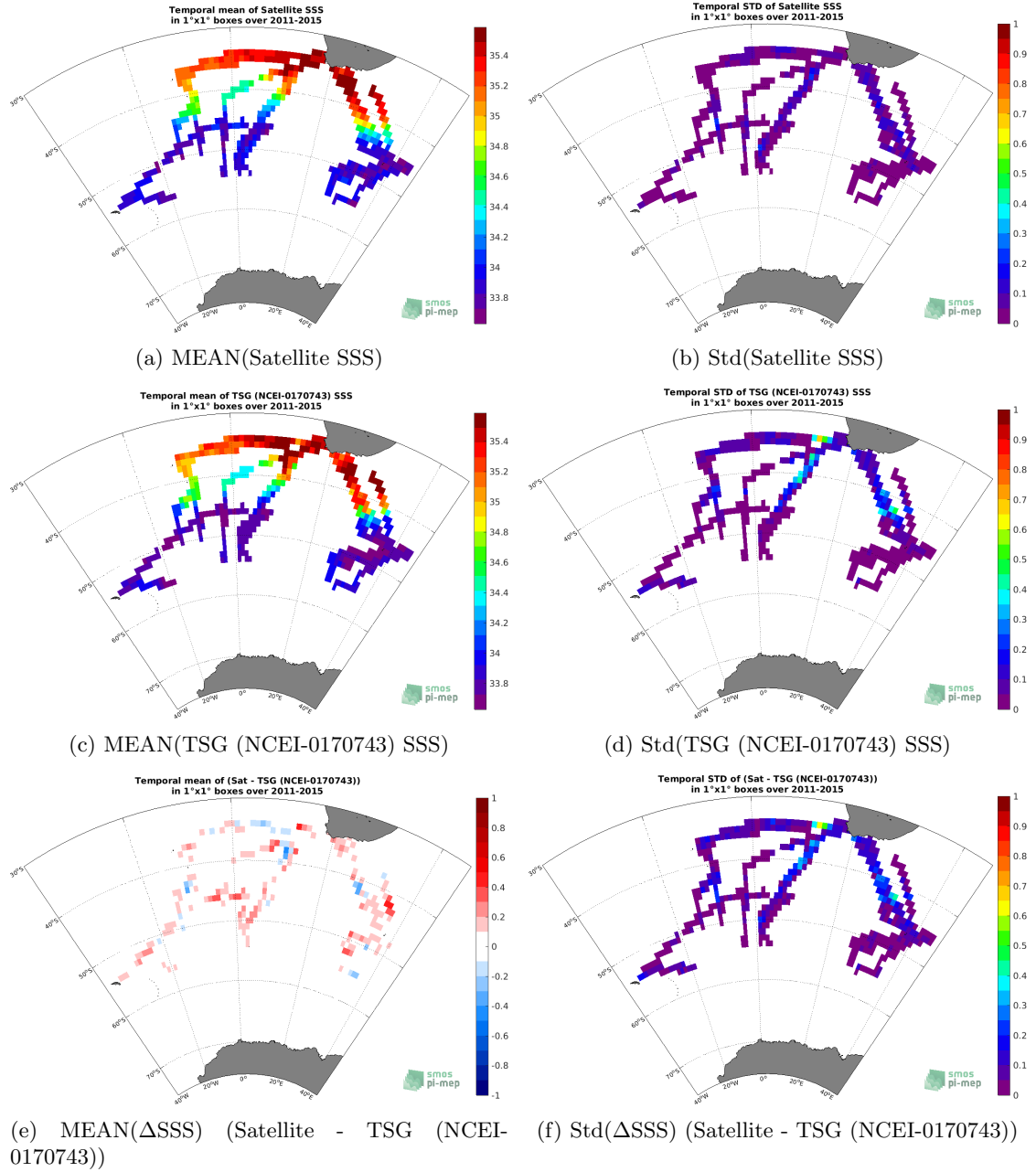
Figure 6: Temporal mean (left) and Std (right) of SSS from Aquarius SSS L4 OI v5 - Weekly (IPRC) (top), TSG (NCEI-0170743) (middle), and of \Delta SSS (Satellite - TSG (NCEI-0170743)). Only match-up pairs are used to generate these maps.
