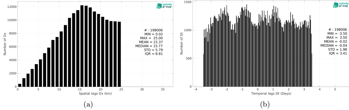
Figure 6: Histograms of the spatial (a) and temporal (b) lags between the location/time of the TSG (LEGOS-Survostral) measurement and the date of the corresponding Aquarius SSS L4 OI v5 - Weekly (IPRC) SSS pixel.
