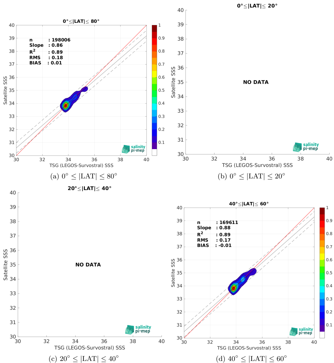
Figure 10: Contour maps of the concentration of Aquarius SSS L4 OI v5 - Weekly (IPRC) SSS (y-axis) versus TSG (LEGOS-Survostral) SSS (x-axis) at match-up pairs for different latitude bands. For each plot, the red line shows x=y . The black thin and dashed lines indicate a linear fit through the data cloud and the \pm 95\% confidence levels, respectively. The number match-up pairs n , the slope and R^2 coefficient of the linear fit, the root mean square (RMS) and the mean bias between satellite and in situ data are indicated for each latitude band in each plots.
