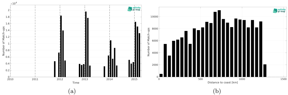
Figure 2: Number of match-ups between TSG (LEGOS-Survostral) and Aquarius SSS L4 OI v5 - Weekly (IPRC) SSS as a function of time (a) and as function of the distance to coast (b) over the Global Ocean Pi-MEP region and for the full satellite product period.
