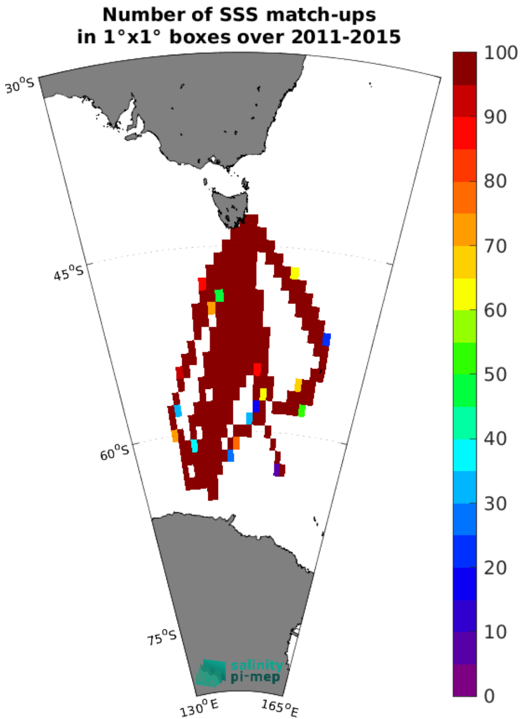
Figure 5: Number of SSS match-ups between TSG (LEGOS-Survostral) SSS and the Aquarius SSS L4 OI v5 - Weekly (IPRC) SSS product for the Global Ocean Pi-MEP region over 1°x1° boxes and for the full satellite product period.
