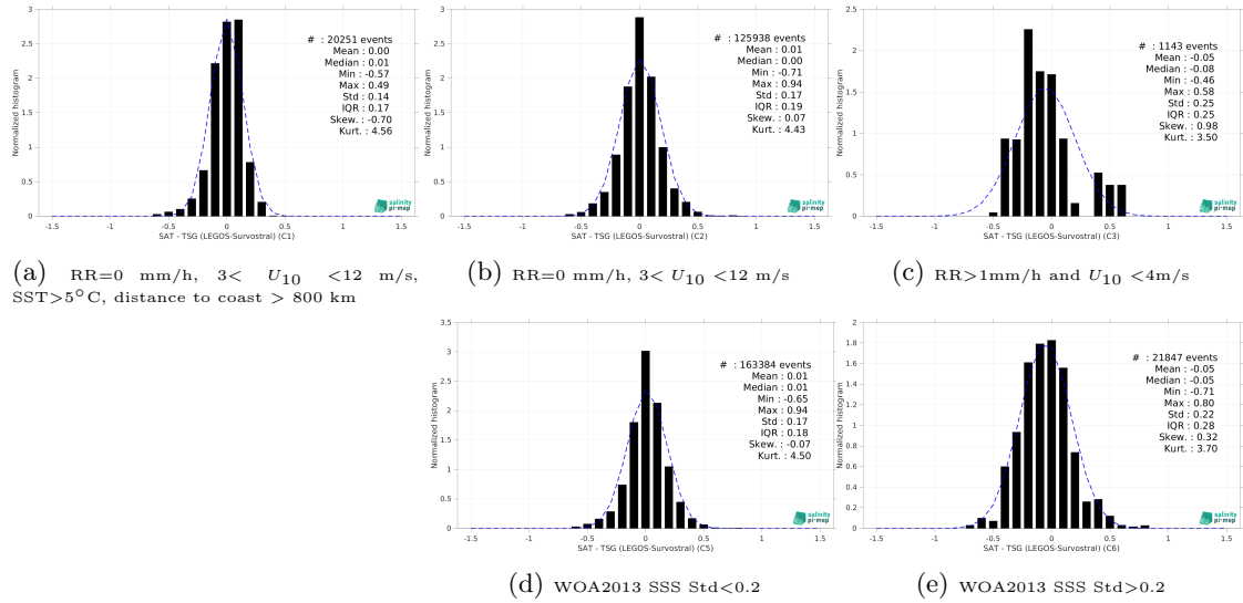
Figure 15: Normalized histogram of \Delta SSS (Aquarius SSS L4 OI v5 - Weekly (IPRC) - TSG (LEGOS-Survostral)) for 5 different subdatasets corresponding to: RR=0 mm/h, 3 < U_{10} < 12 m/s, SST>5°C, distance to coast > 800 km (a), RR=0 mm/h, 3 < U_{10} < 12 m/s (b), RR>1mm/h and U_{10} < 4 m/s (c), WOA2013 SSS Std<0.2 (d), WOA2013 SSS Std>0.2 (e).
