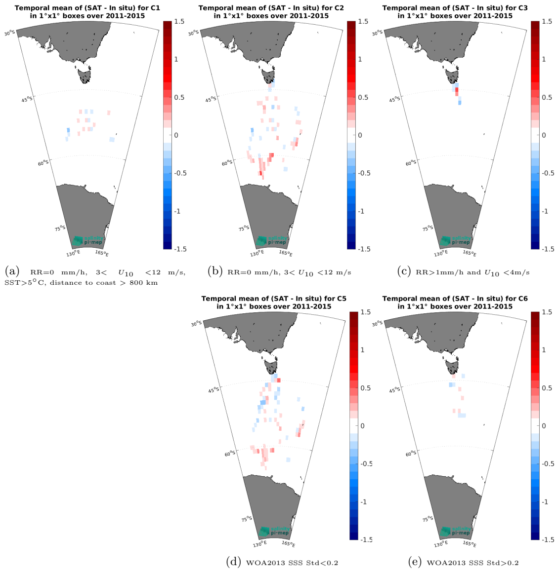
Figure 14: Temporal mean gridded over spatial boxes of size 1^\circ \times 1^\circ of \Delta SSS (Aquarius SSS L4 OI v5 - Weekly (IPRC) - TSG (LEGOS-Survostral)) for 5 different subdatasets corresponding to:RR=0 mm/h, 3 < U_{10} < 12 m/s, SST>5°C, distance to coast > 800 km (a), RR=0 mm/h, 3 < U_{10} < 12 m/s (b), RR>1mm/h and U_{10} < 4 m/s (c), WOA2013 SSS Std<0.2 (d), WOA2013 SSS Std>0.2 (e).
