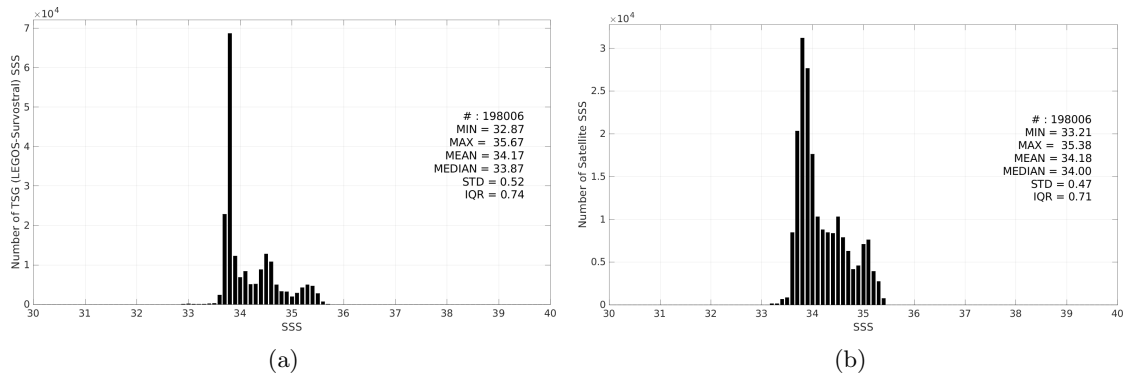
Figure 3: Histograms of SSS from TSG (LEGOS-Survostral) (a) and Aquarius SSS L4 OI v5 - Weekly (IPRC) (b) considering all match-up pairs per bins of 0.1 over the Global Ocean Pi-MEP region and for the full satellite product period.
