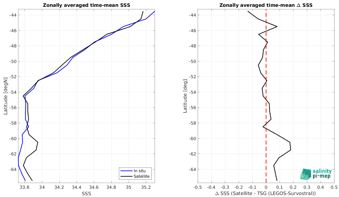
Figure 9: Left panel: Zonal mean SSS from Aquarius SSS L4 OI v5 - Weekly (IPRC) satellite product (black) and from TSG (LEGOS-Survostral) (blue). Right panel: Zonal mean of \Delta SSS (Satellite - TSG (LEGOS-Survostral)) for all the collected Pi-MEP match-up pairs estimated over the full satellite product period.
