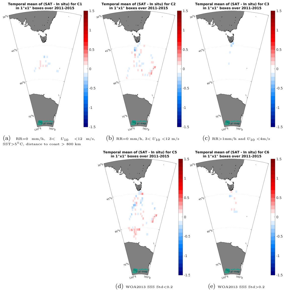
Figure 12: Temporal mean gridded over spatial boxes of size 1^{\circ} \times 1^{\circ} of \Delta\text{SSS} (Aquarius SSS L4 OI v5 - Weekly (IPRC) - TSG (LEGOS-Survostral)) for 5 different subdatasets corresponding to: RR=0 mm/h, 3 < U_{10} < 12 m/s, SST > 5^{\circ}\text{C} , distance to coast > 800 km (a), RR=0 mm/h, 3 < U_{10} < 12 m/s (b), RR > 1 mm/h and U_{10} < 4 m/s (c), WOA2013 SSS Std < 0.2 (d), WOA2013 SSS Std > 0.2 (e).
