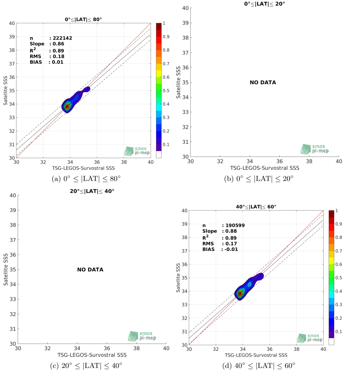
Figure 9: Contour maps of the concentration of Aquarius-L4-IPRC-V5-WEEKLY SSS (y-axis) versus TSG-LEGOS-Survostral SSS (x-axis) at match-up pairs for different latitude bands. For each plot, the red line shows x=y . The black thin and dashed lines indicate a linear fit through the cloud and the \pm 95\% confidence levels, respectively. The number match-up pairs n , the slope and R^2 coefficient of the linear fit, the root mean square (RMS) and the mean bias between satellite and in situ data are indicated for each latitude band in each plots.
