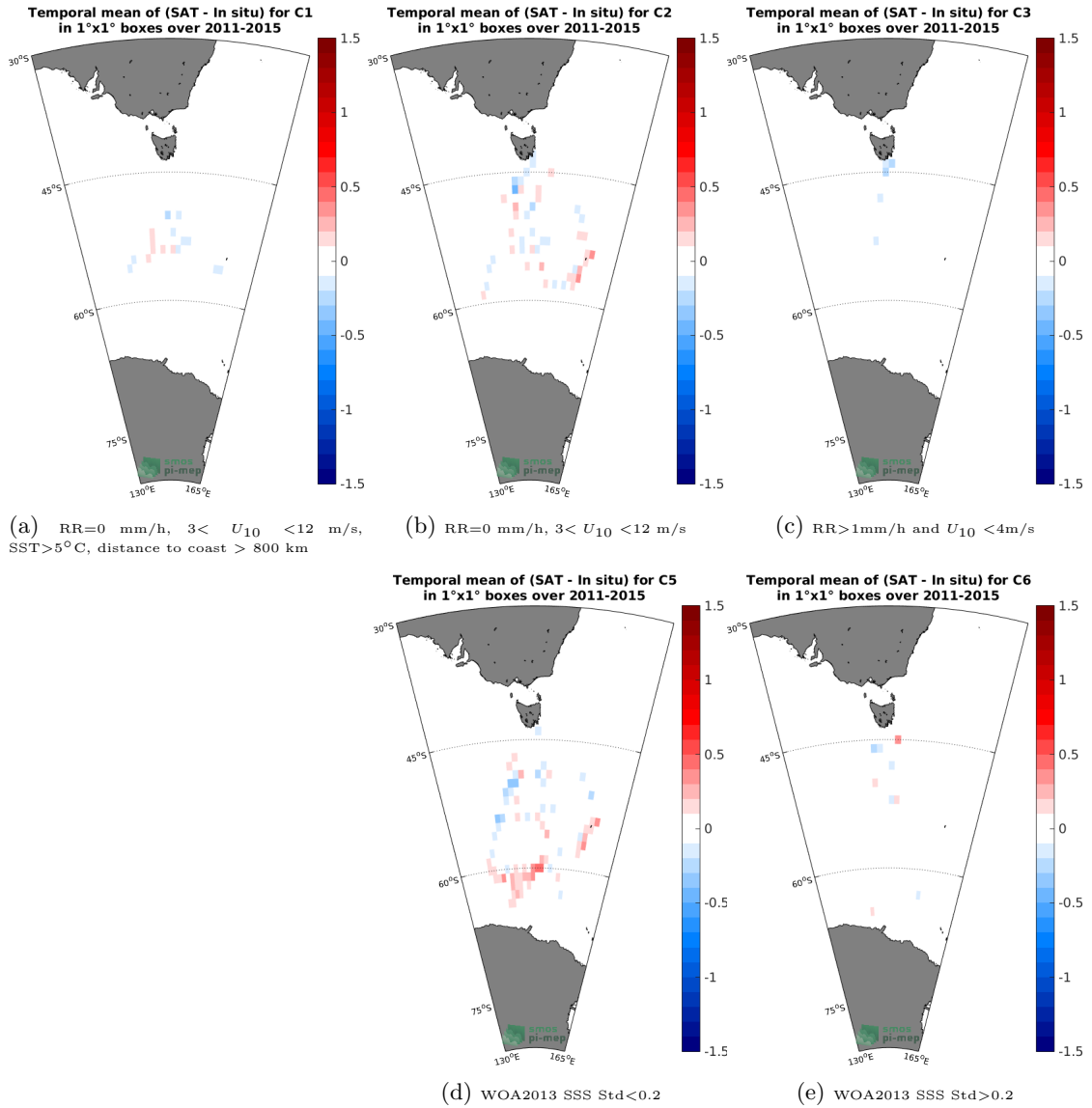
Figure 12: Temporal mean gridded over spatial boxes of size 1^\circ \times 1^\circ of \Delta\text{SSS} (Aquarius-L4-IPRC-V5-WEEKLY - TSG-LEGOS-Survostral) for 5 different subdatasets corresponding to: RR=0 mm/h, 3 < U_{10} < 12 m/s, SST > 5^\circ\text{C} , distance to coast > 800 km (a), RR=0 mm/h, 3 < U_{10} < 12 m/s (b), RR > 1 mm/h and U_{10} < 4 m/s (c), WOA2013 SSS Std < 0.2 (d), WOA2013 SSS Std > 0.2 (e).
