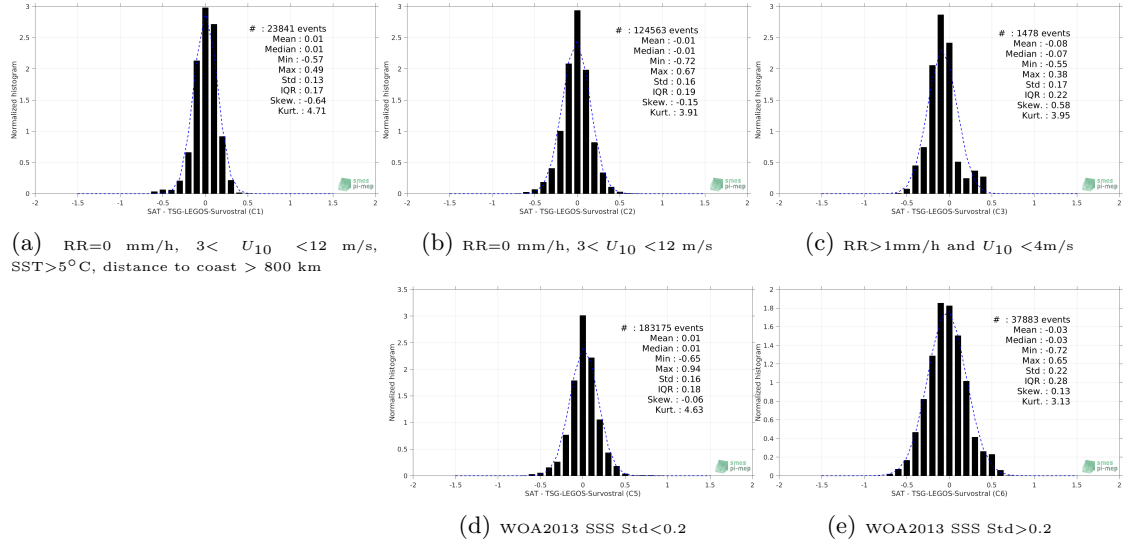
Figure 13: Normalized histogram of \Delta SSS (Aquarius-L4-IPRC-V5-WEEKLY - TSG-LEGOS-Survostral) for 5 different subdatasets corresponding to: RR=0 mm/h, 3 < U_{10} < 12 m/s, SST>5°C, distance to coast > 800 km (a), RR=0 mm/h, 3 < U_{10} < 12 m/s (b), RR>1mm/h and U_{10} < 4 m/s (c), WOA2013 SSS Std<0.2 (d), WOA2013 SSS Std>0.2 (e).
