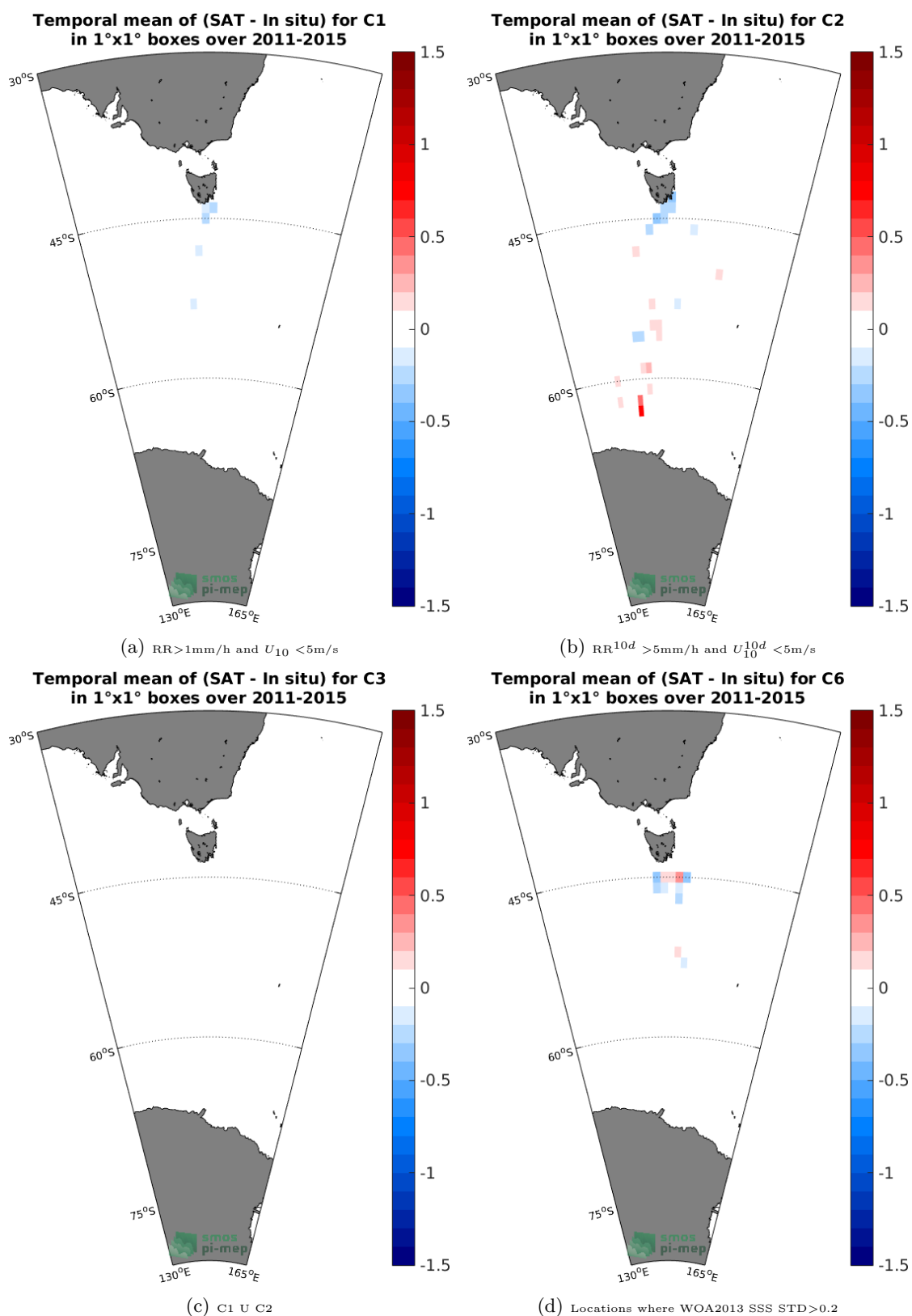
Figure 12: Temporal mean gridded over spatial boxes of size 1°x1° of \Delta\text{SSS} (Aquarius-L4-IPRC-V5-WEEKLY - TSG-LEGOS-Survostral) for 4 different subdatasets corresponding to: RR > 1\text{mm/h} and U_{10} < 5\text{m/s} (a), RR^{10d} > 5\text{mm/h} and U_{10}^{10d} < 5\text{m/s} (b), C1 U C2 (c), Locations where WOA2013 SSS STD > 0.2 (d).
