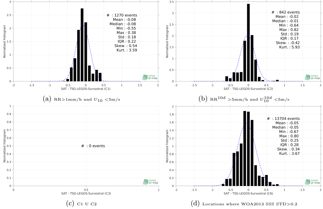
Figure 13: Normalized histogram of \Delta\text{SSS} (Aquarius-L4-IPRC-V5-WEEKLY - TSG-LEGOS-Survostral) for 6 different subdatasets corresponding to: RR > 1\text{mm/h} and U_{10} < 5\text{m/s} (a), RR^{10d} > 5\text{mm/h} and U_{10}^{10d} < 5\text{m/s} (b), C1 \cup C2 (c), Locations where WOA2013 SSS STD > 0.2 (d).
