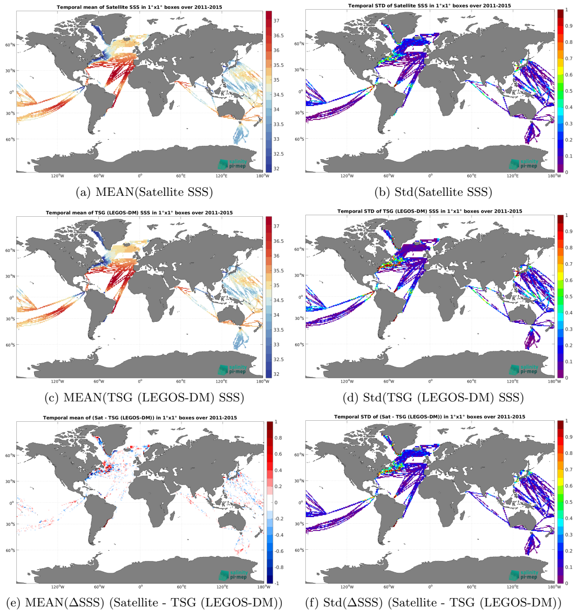
Figure 7: Temporal mean (left) and Std (right) of SSS from Aquarius SSS L4 OI v5 - Weekly (IPRC) (top), TSG (LEGOS-DM) (middle), and of \Delta SSS (Satellite - TSG (LEGOS-DM)). Only match-up pairs are used to generate these maps.
