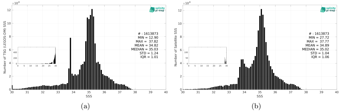
Figure 3: Histograms of SSS from TSG (LEGOS-DM) (a) and Aquarius SSS L4 OI v5 - Weekly (IPRC) (b) considering all match-up pairs per bins of 0.1 over the Global Ocean Pi-MEP region and for the full satellite product period.
