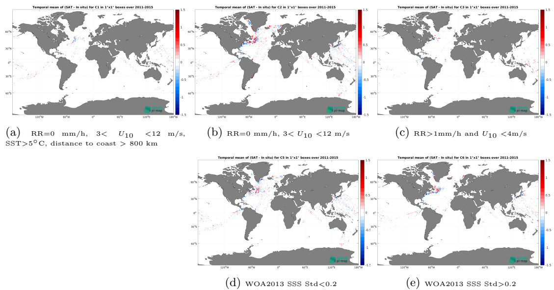
Figure 14: Temporal mean gridded over spatial boxes of size 1^\circ \times 1^\circ of \Delta SSS (Aquarius SSS L4 OI v5 - Weekly (IPRC) - TSG (LEGOS-DM)) for 5 different subdatasets corresponding to:RR=0 mm/h, 3 < U_{10} < 12 m/s, SST > 5^\circ\text{C} , distance to coast > 800 km (a), RR=0 mm/h, 3 < U_{10} < 12 m/s (b), RR > 1 mm/h and U_{10} < 4 m/s (c), WOA2013 SSS Std < 0.2 (d), WOA2013 SSS Std > 0.2 (e).
