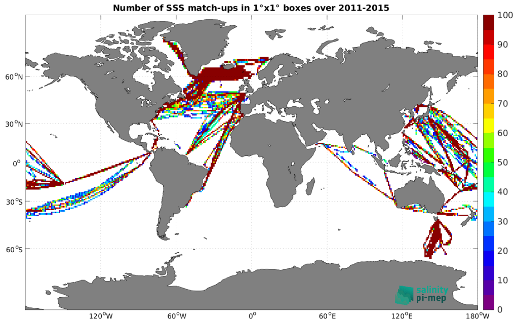
Figure 5: Number of SSS match-ups between TSG (LEGOS-DM) SSS and the Aquarius SSS L4 OI v5 - Weekly (IPRC) SSS product for the Global Ocean Pi-MEP region over 1^\circ \times 1^\circ boxes and for the full satellite product period.
