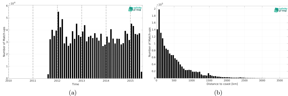
Figure 2: Number of match-ups between TSG (LEGOS-DM) and Aquarius SSS L4 OI v5 - Weekly (IPRC) SSS as a function of time (a) and as function of the distance to coast (b) over the Global Ocean Pi-MEP region and for the full satellite product period.
