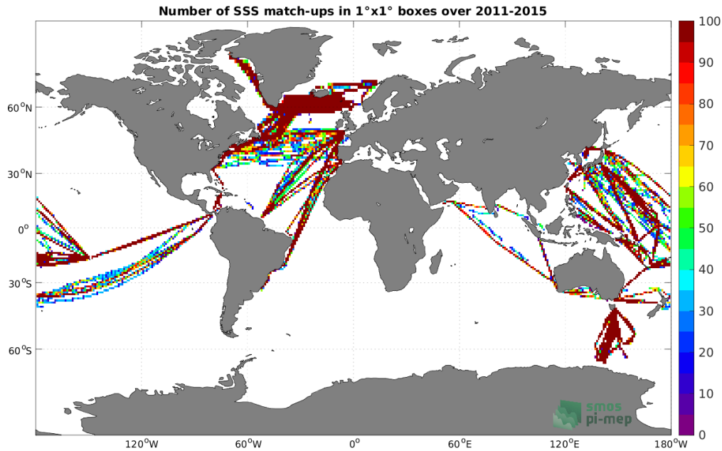
Figure 4: Number of SSS match-ups between TSG (LEGOS-DM) SSS and the Aquarius SSS L4 OI v5 - Weekly (IPRC) SSS product for the Global Ocean Pi-MEP region over 1^\circ \times 1^\circ boxes and for the full satellite product period.
