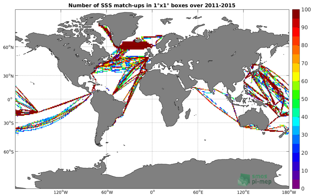
Figure 4: Number of SSS match-ups between TSG-LEGOS-DM SSS and the Aquarius-L4-IPRC-V5-WEEKLY SSS product for the Global Ocean Pi-MEP region over 1^\circ \times 1^\circ boxes and for the full satellite product period.
