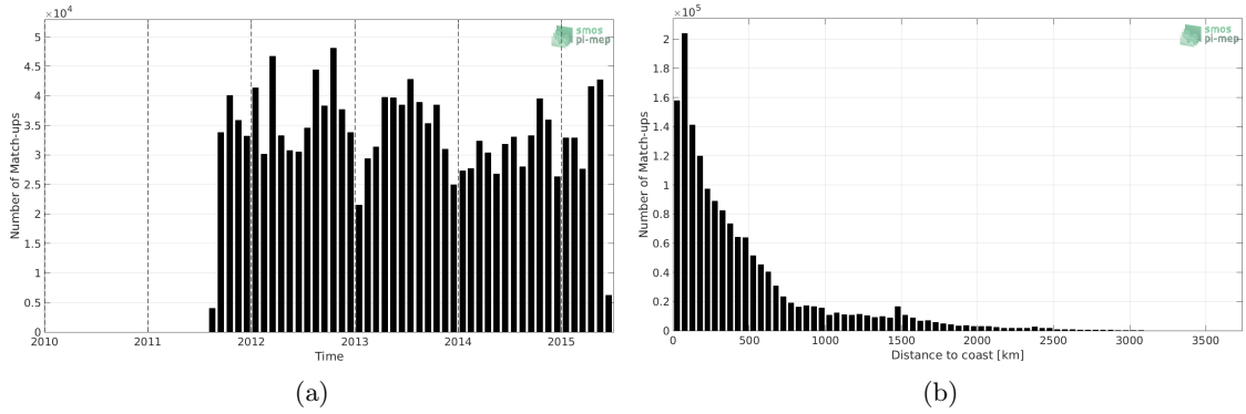
Figure 1: Number of match-ups between TSG-LEGOS-DM and Aquarius-L4-IPRC-V5-WEEKLY SSS as a function of time (a) and as function of the distance to coast (b) over the Global Ocean Pi-MEP region and for the full satellite product period.
