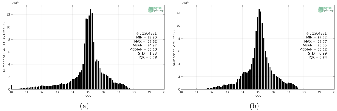
Figure 2: Histograms of SSS from TSG-LEGOS-DM (a) and Aquarius-L4-IPRC-V5-WEEKLY (b) considering all match-up pairs per bins of 0.1 over the Global Ocean Pi-MEP region and for the full satellite product period.
