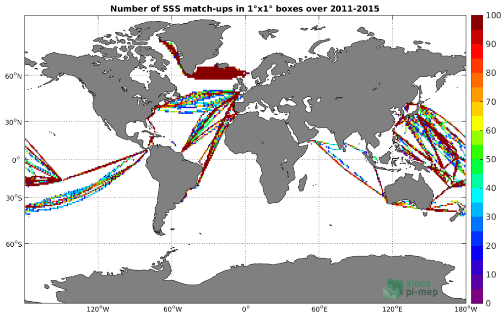
Figure 4: Number of SSS match-ups between TSG-LEGOS-DM SSS and the Aquarius-L4-IPRC-V5-WEEKLY SSS product for the Global Ocean Pi-MEP region over 1°x1° boxes and for the full satellite product period.
