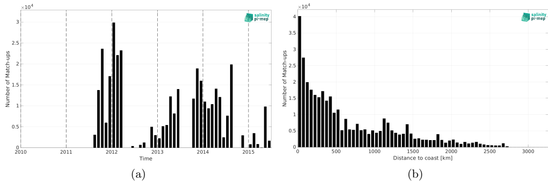
Figure 2: Number of match-ups between TSG (GOSUD-Sailing-ship) and Aquarius SSS L4 OI v5 - Weekly (IPRC) SSS as a function of time (a) and as function of the distance to coast (b) over the Global Ocean Pi-MEP region and for the full satellite product period.
