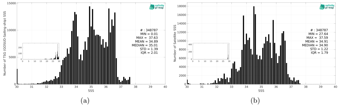
Figure 3: Histograms of SSS from TSG (GOSUD-Sailing-ship) (a) and Aquarius SSS L4 OI v5 - Weekly (IPRC) (b) considering all match-up pairs per bins of 0.1 over the Global Ocean Pi-MEP region and for the full satellite product period.
