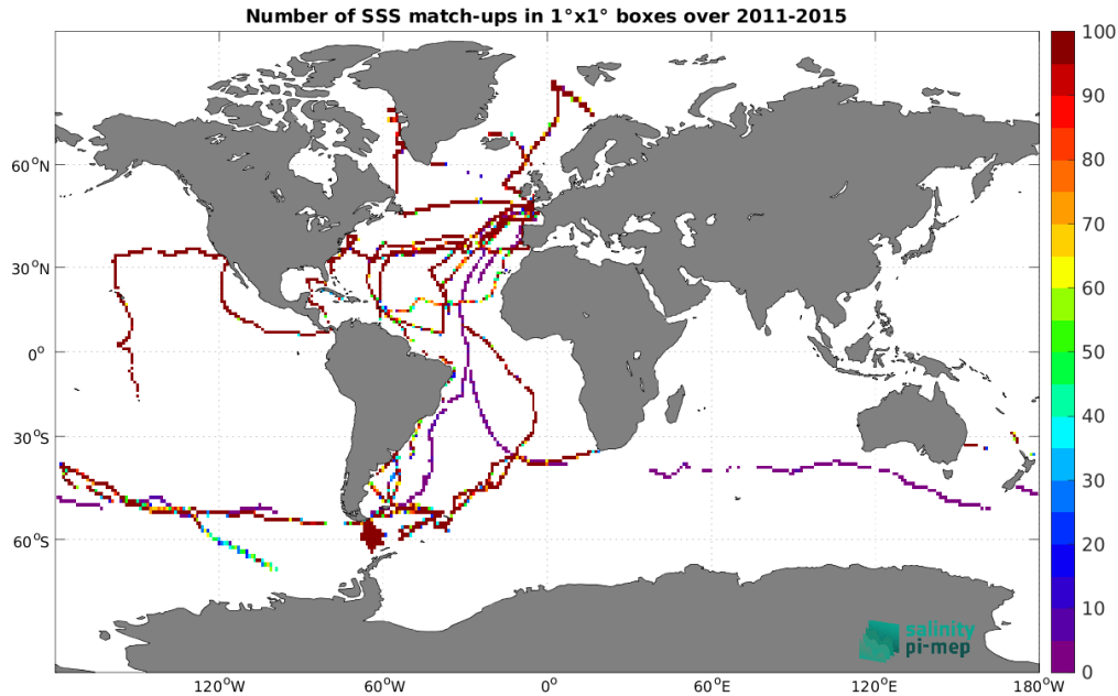
Figure 4: Number of SSS match-ups between TSG (GOSUD-Sailing-ship) SSS and the Aquarius SSS L4 OI v5 - Weekly (IPRC) SSS product for the Global Ocean Pi-MEP region over 1°x1° boxes and for the full satellite product period.
