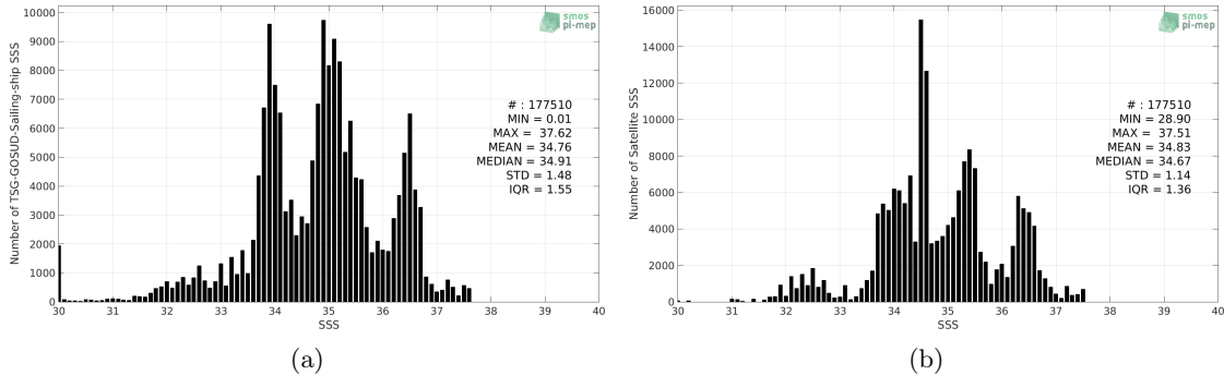
Figure 2: Histograms of SSS from TSG-GOSUD-Sailing-ship (a) and Aquarius-L4-IPRC-V5-WEEKLY (b) considering all match-up pairs per bins of 0.1 over the Global Ocean Pi-MEP region and for the full satellite product period.
